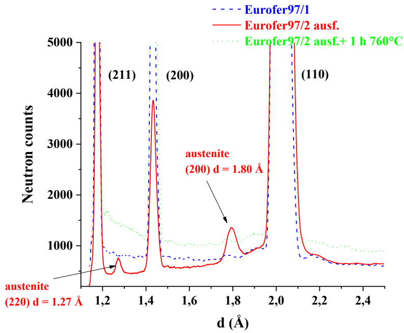
Fig. 7 - Neutron diffractograms (normalized neutron counts vs lattice plane distance, in \text{\AA} ) for the same samples of fig. 3: Eurofer97/1 reference heat 83697, 1040 C 30' + 750° C 1.5 h (blue, dashed line), Eurofer97/2 1175 °C 30' + ausformed at 650° C (red, continuous line) and Eurofer97/2 1175 °C 30' + ausformed at 650° C + 1 h C 760°C (green, dotted line). Due to the low instrument resolution at 2.1 \text{\AA} [20], the (111) austenite and (110) Eurofer peaks could not be separated.
