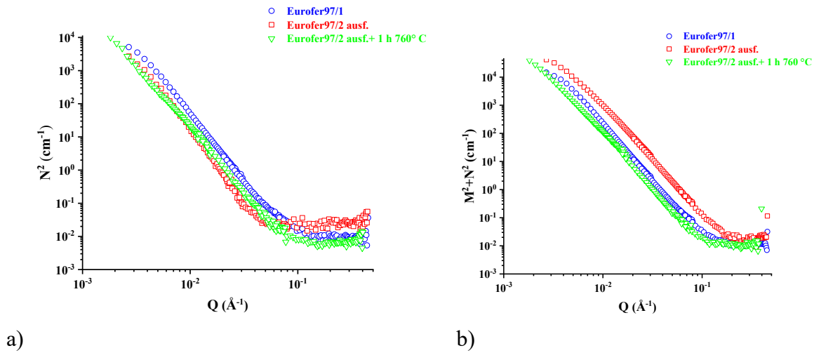
Fig. 4 – Calibrated SANS cross-sections parallel (a) and perpendicular (b) to magnetic field for Eurofer97/1 reference heat 83697, 1040 C 30' + 750° C 1.5 h (blue, circles), for Eurofer97/2 1175 °C 30' + ausformed at 650°C (red, squares) and for Eurofer97/2 1175 °C 30' + ausformed at 650 C + 1 h C 760°C (green, triangles).
