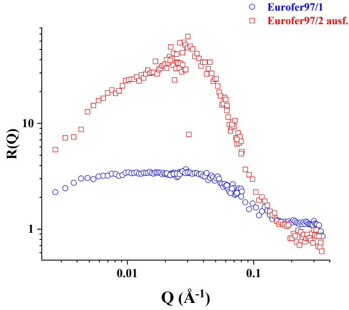
Fig. 5 – R(Q) values for Eurofer97/1 reference heat 83697, 1040 °C 30' + 750 °C 1.5 h (blue, circles) and for Eurofer97/2 1175 °C 30' + ausformed at 650 °C (red, squares).
