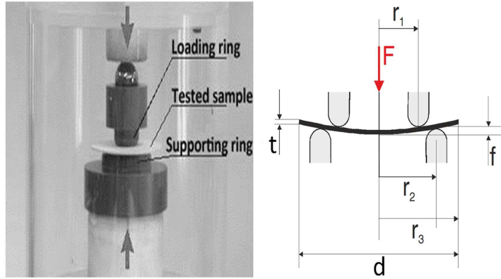
Figure 3.6 The ring-on-ring bending test set-up in IEK-2.
