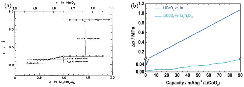
Figure 2.4 (a) Structural changes in tetragonal unit cell dimension of Li x Mn 2 O 4 showing an initial phase change expansion, then stoichiometric expansion and ultimate phase change expansion [109]. (b) A direct comparison of the pressure-change in SSBs with an indium anode (deep blue) and a Li 4 Ti 5 O 12 anode (light blue) [110].
