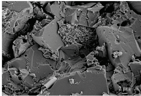
Figure 4.16 SEM micrograph of fracture surface of LATP:Si.
