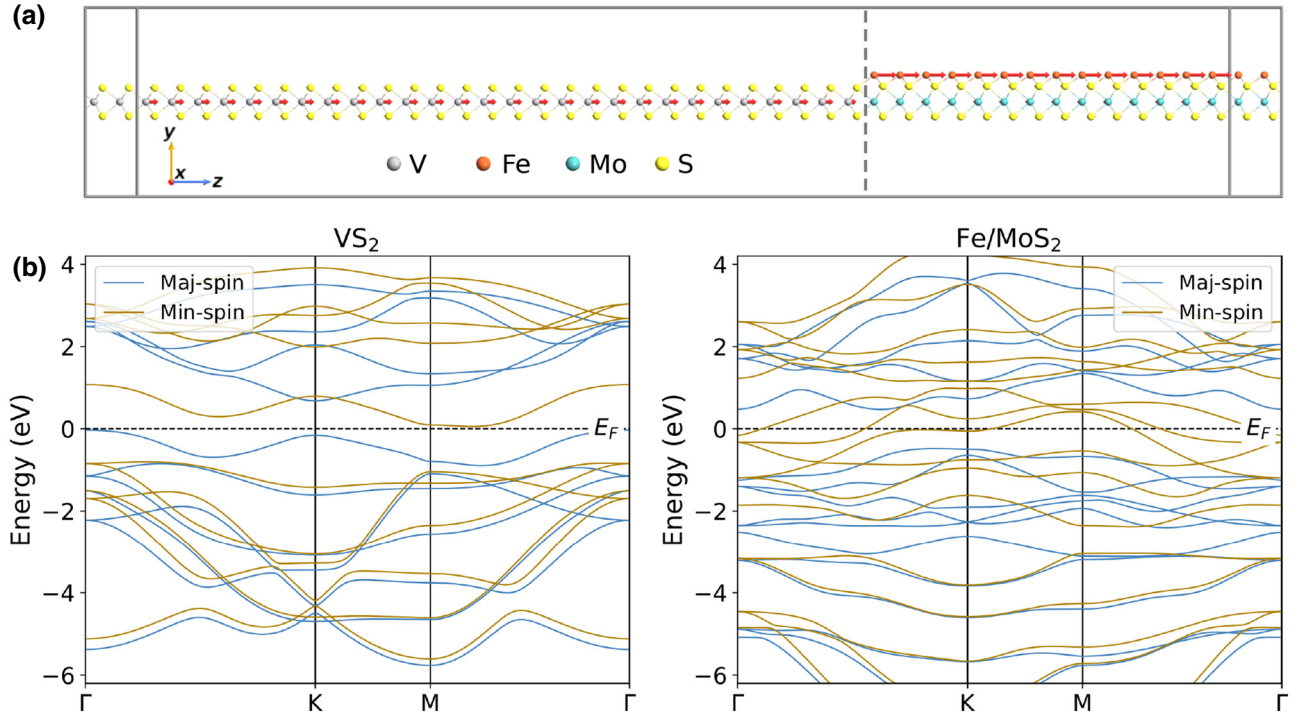
FIG. 6. (a) The atomic structure of the \text{VS}_2 -Fe/MoS _2 Ohmic spin diode. The arrows show the magnetic moments of V and Fe atoms in the SGS and HMM electrodes within the scattering region. The size of the arrows is proportional to the magnitude of the magnetic moments. The system is periodic in the x direction in the plane orthogonal to the magnetization direction, which is also the transport direction. The vertical dashed lines denote the interface. (b) The calculated spin-resolved bulk electronic band structure along the high-symmetry lines in the Brillouin zone for \text{VS}_2 (left-hand panel) and Fe/MoS _2 (right-hand panel). For both compounds, the dashed lines denote the Fermi energy, which is set to zero.
