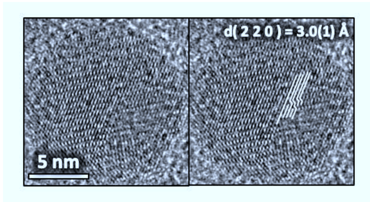
FIG. 6. HRTEM micrographs of one representative NP with visible dislocation.
