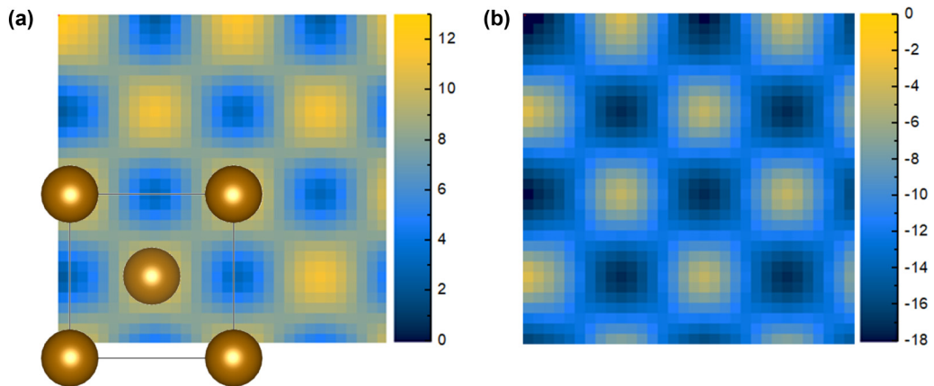
FIG. 6. Spatial mapping of the function D^{l=1}_{\alpha=7\text{mrad}} computed for the Fe (a) L_2 and (b) L_3 edges. The contrast in the images provides access to atomically resolved mapping of magnetic properties of the sample.
