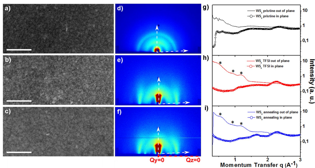
Figure 2. High-magnification SEM images of WS 2 nanoflakes deposited on glass substrates by spin coating: (a) film obtained upon a single deposition step, without any post-deposition treatment; (b,c) films fabricated layer-by-layer by multiple deposition steps and subjected to either (b) TFSI treatment or (c) thermal annealing, respectively, at each deposition step. Scale bars in (a–c) are 100 nm long. (d–f) 2D GIWAXS maps of the WS 2 nanoflake films shown in panels a–c, respectively. (g–i) Corresponding in-plane (open circles) and out-of-plane cuts (solid line) taken along the white arrows in the 2D GIWAXS maps from panels d–f, respectively. Asterisks highlight broad peaks in the low q -range indicating an out-of-plane periodicity of 10 or 20 Å, compatible with a sheet-stacking direction perpendicular to film surface.
