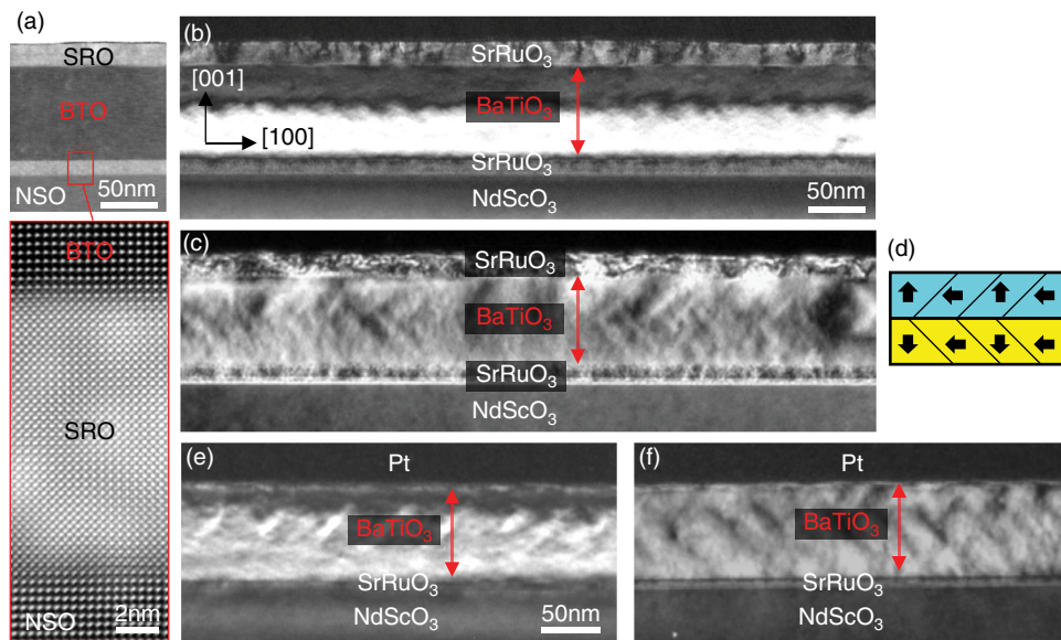
FIG. 1. (a) High resolution scanning transmission electron microscopy with a high angle annular dark-field detector (STEM-HAADF) image of an 80 nm thick \text{BaTiO}_3 film with a 12 nm \text{SrRuO}_3 bottom electrode and a 20 nm \text{SrRuO}_3 top electrode (the quasisymmetric electrode configuration). The bottom image shows a magnified view of the \text{NdScO}_3/\text{SrRuO}_3/\text{BaTiO}_3 interfaces, which shows a defect-free epitaxial growth. (b) Vertical (002) dark-field TEM images of the previous sample, which shows a strong variation of contrast in the middle of the film, attributed to a charged 180^\circ domain wall. (c) Horizontal (200) dark-field image that shows repeated variations of contrast at 45^\circ to the interfaces, attributed to a/c (or 90^\circ ) twin domains. (d) Simplified schematics of the domain structure and polarization directions. The cyan region represents the averaged up-polarized, and the yellow the down-polarized state, as from the vertical dark-field. (e) Vertical (002) and (f) Horizontal (200) dark-field images of an 80 nm thick \text{BaTiO}_3 film with a (reduced) 6 nm \text{SrRuO}_3 bottom electrode and a 300 nm thick Pt top electrode (the asymmetric electrode configuration).
