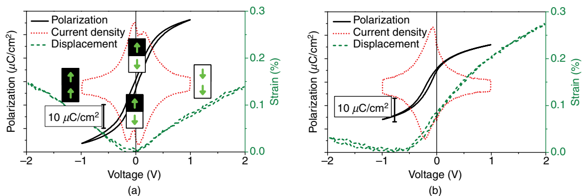
FIG. 2. (a) An 80 nm \text{BaTiO}_3 thin film with quasisymmetric 12 nm bottom and 20 nm \text{SrRuO}_3 top electrodes measured at room temperature for a 100 Hz electric field applied along the [001] out-of-plane direction. The insets show a sketch of the local averaged polarization above and below the original 180^\circ horizontal domain wall. (b) \text{BaTiO}_3 film with asymmetric 6 nm \text{SrRuO}_3 bottom and 20 nm \text{SrRuO}_3 top electrodes. Note that the measurement technique can only measure differences in polarization.
