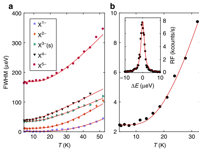
Fig. 4 Linewidths of excitons in an AlAs-capped quantum dot.
