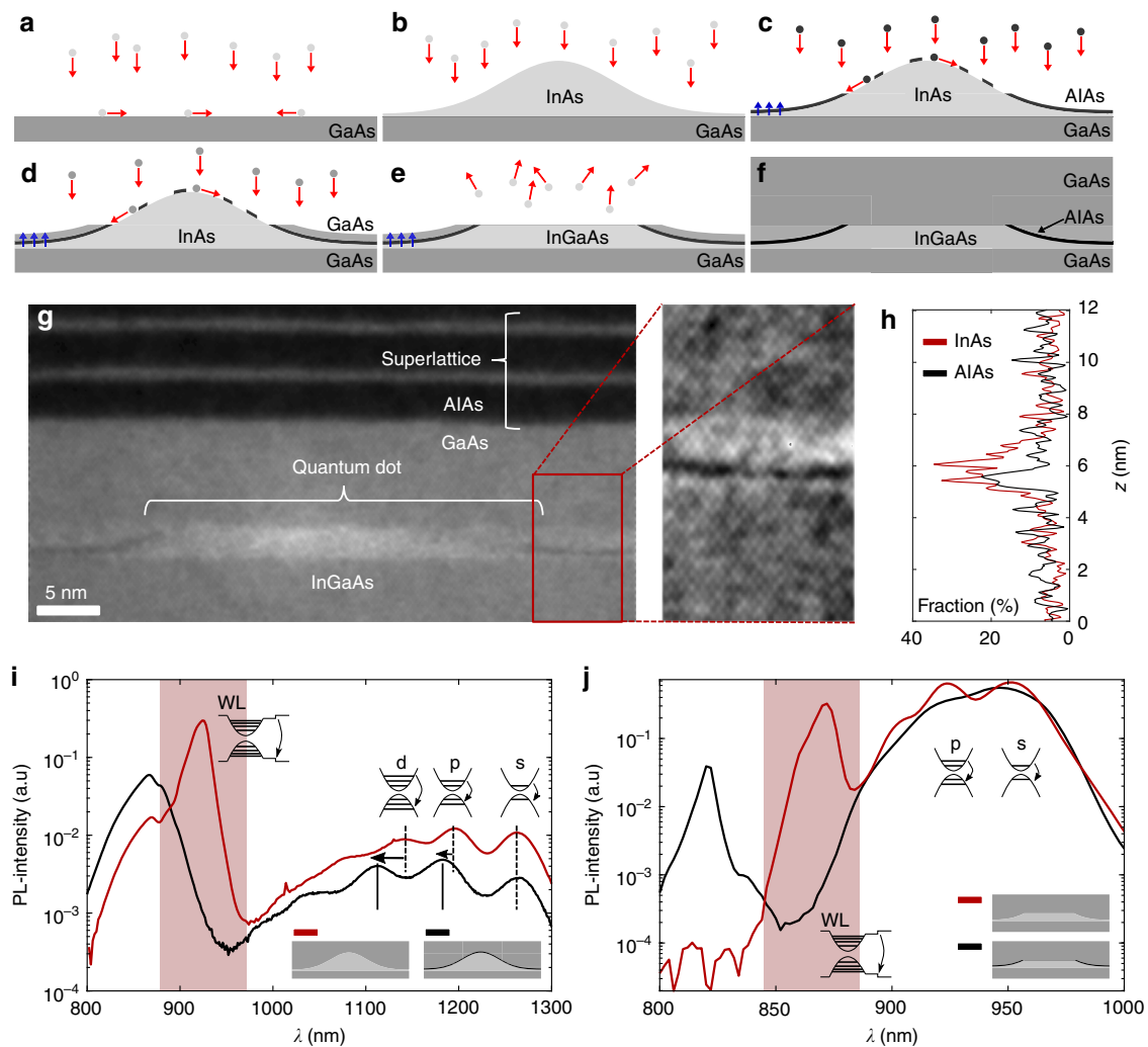
Fig. 1 Growth and characterization of the quantum dots. a–f Schematic process of the quantum dot (QD) growth. a InAs is deposited on a GaAs-surface. b After deposition of ~1.5 monolayers of InAs, strain-driven QD-formation takes place. The QDs are capped with a monolayer of AlAs ( c ) and 2 nm GaAs ( d ). During these steps segregation of In atoms takes place (blue arrows) resulting in a wetting layer (WL) which is an alloy of GaAs, InAs, and AlAs. e The top part of the capped QD evaporates at 630 °C (flushing step). f The flushed QDs are overgrown with GaAs. g Scanning transmission electron microscopy image of a flushed QD. InAs appears bright, AlAs dark. h Chemical composition of the WL measured by spatially resolved energy dispersive X-ray (EDX) spectroscopy at a location without a QD (different location to g but nominally the same). i Ensemble photoluminescence (PL) at room temperature from a sample with unflushed, standard InGaAs QDs (red curve) and unflushed, AlAs-capped InGaAs QDs (black curve). The WL PL (highlighted by the red band) dominates the spectrum. The QD PL appears in the regime 1000–1300 nm. The QD-shells are labeled. j Ensemble-PL at 77 K from a sample with flushed, standard InGaAs QDs (red curve) and flushed, AlAs-capped InGaAs QDs (black curve). The flushing blue-shifts the QD-ensemble to ~900–980 nm
