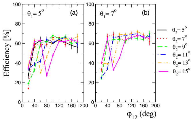
FIG. 12. Efficiency of the detection of proton-proton coincidences determined on the basis of MC simulation. The results for a number of selected kinematical configurations ( \theta_1 , \theta_2 , \phi_{12} ) are shown as points with statistical errors. Lines are added to guide the eye.
