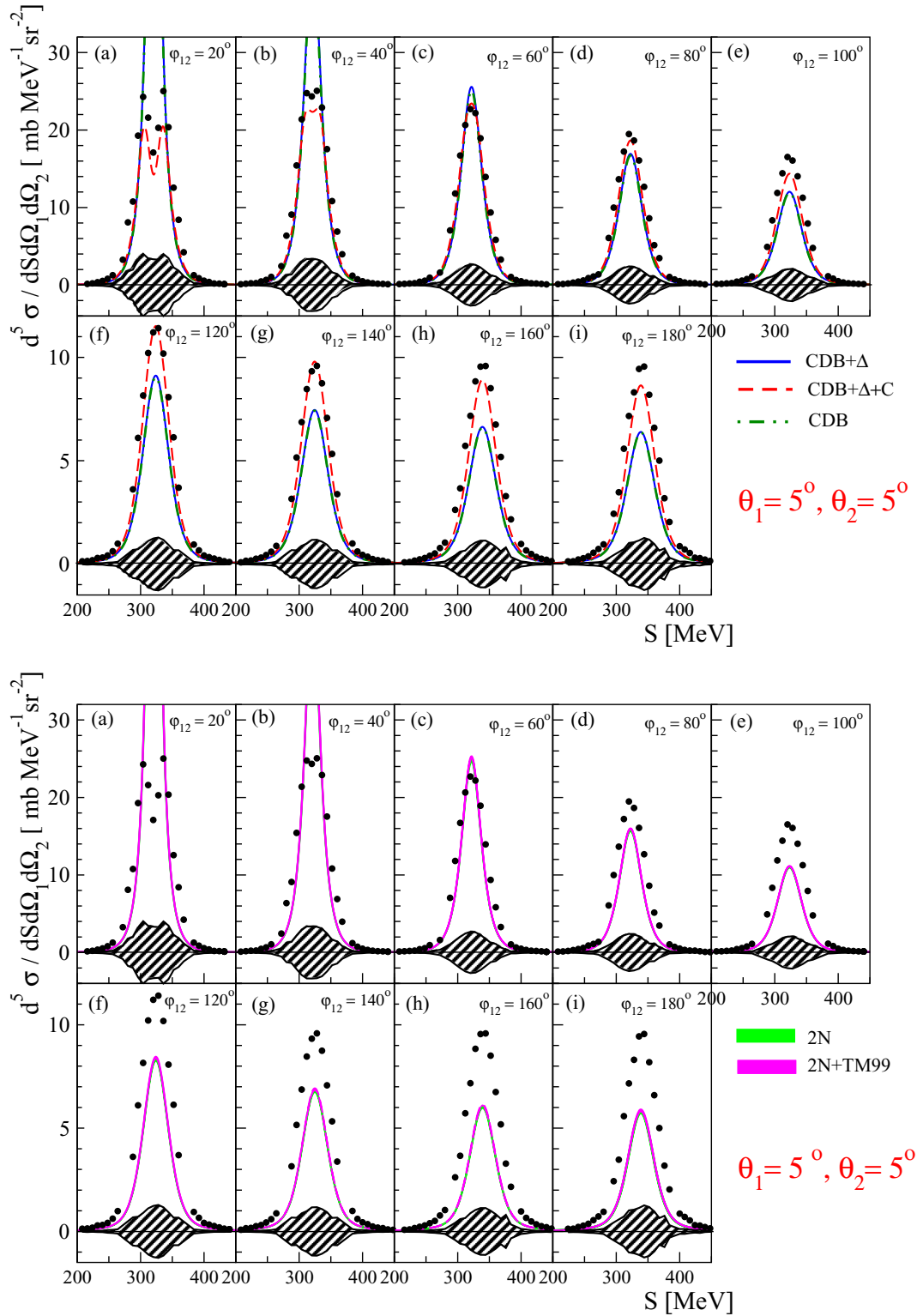
FIG. 15. Differential cross section of ^1\text{H}(d, pp)n breakup reaction at beam energy of 170 MeV/nucleon shown in function of S variable. The presented data belong to nine kinematic configurations characterized with the same combinations of proton polar angles ( \theta_1 = 5^\circ, \theta_2 = 5^\circ ) and various relative azimuthal angles of the two protons, indicated in the individual panels. Statistical errors are smaller than the point size. Systematic uncertainties are represented by hatched band. Top: Data compared to predictions obtained for the calculations within the coupled-channels approach with the CD Bonn potential (CDB, dotted-dashed green line), with the CDBonn+ \Delta potential without (CDB+ \Delta , blue solid line) and with the Coulomb force included (CDB+ \Delta +C, red dashed line). Bottom: The same data confronted with the predictions based on NN potentials: 2N (AV18, CD Bonn, Nijm I and II) [green (light gray) band] and NN combined with the TM99 3NF [magenta (dark gray) band].
