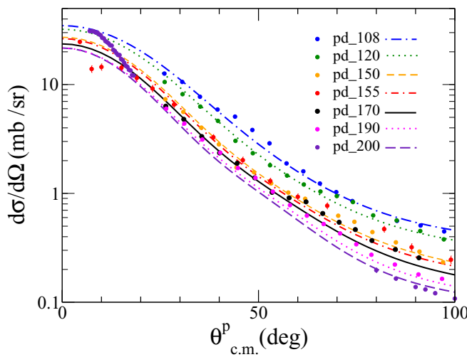
FIG. 9. Experimental differential cross section of the reaction ^2\text{H}(p, dp) in the center of mass (CM) system in the angular range of FD, at the incident-beam energies: 108, 120, 150, 170, 190 [38], 155 [39], and 200 MeV [41,42]. The lines show the results of the theoretical calculations with the CD Bonn potential and the TM99 3NF.
