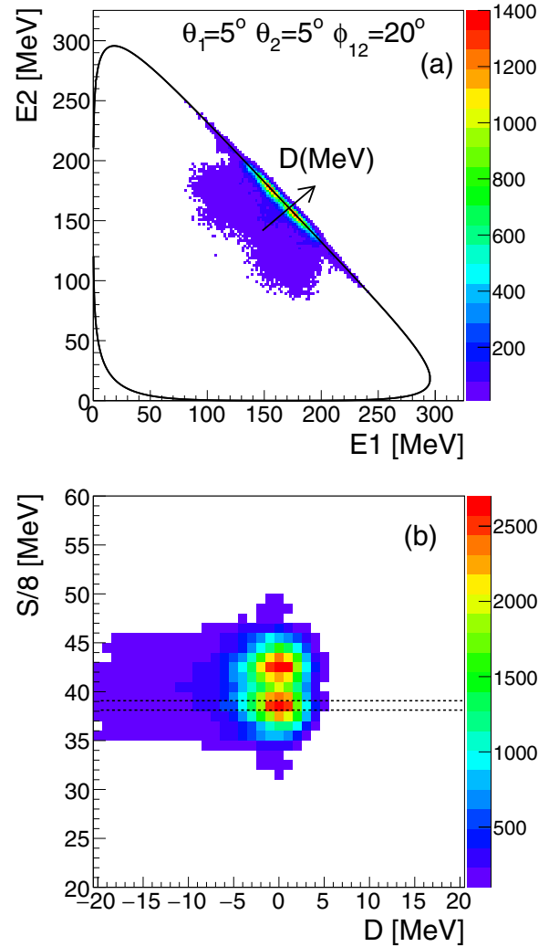
FIG. 4. (a) E_1 vs. E_2 coincidence spectrum of the two protons registered at \theta_1 = 5^\circ \pm 1^\circ , \theta_2 = 5^\circ \pm 1^\circ , and \varphi_{12} = 20^\circ \pm 5^\circ . The solid line shows a three-body kinematical curve, calculated for the central values of experimental angular ranges. D axis illustrates the distance of the (E_1, E_2) point from the kinematical curve. (b) Transformation of E_1 vs. E_2 spectrum to S (arclength) vs. D (distance from kinematical line in E_1 - E_2 plane). Dashed lines represent integration limits ( \Delta S = 8 MeV) for a sample S slice.
