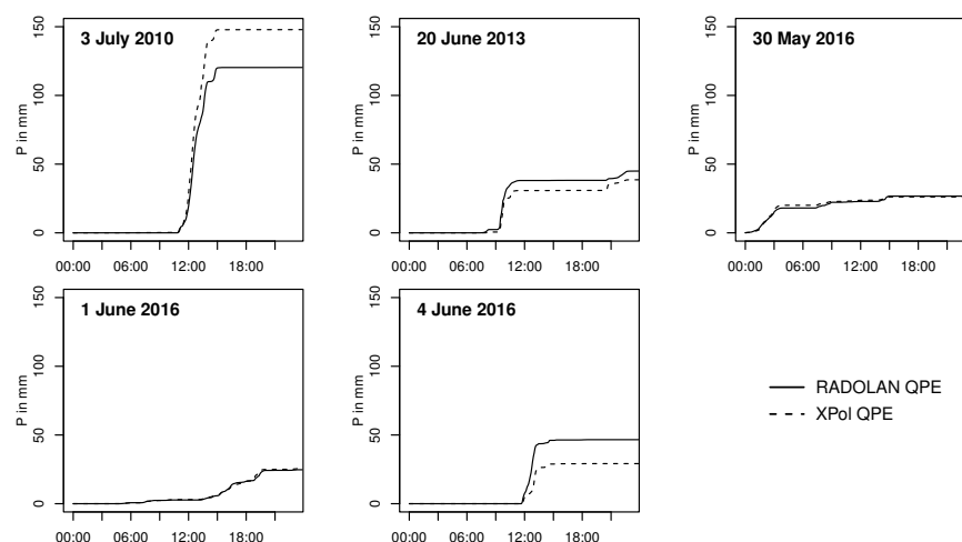
Figure 3. Comparison of cumulative RADOLAN and XPol QPE rain depth, where P is the precipitation in mm.
