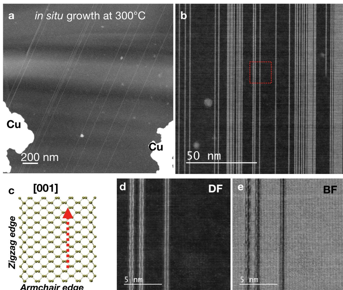
Figure 1: Rapid self-assembly of Copper (Cu) heterostructures of high aspect ratio
