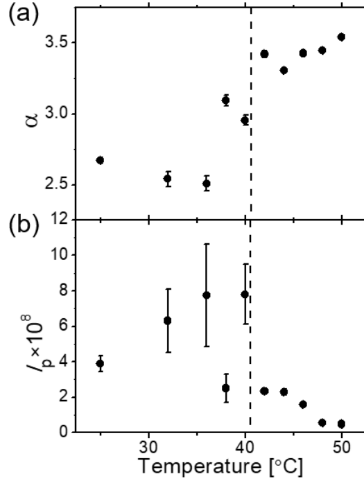
Figure 6. Parameters from the modified Porod term in SANS data of the 30 g L -1 solution of PiPOx 100 -g-PETox 17 in D 2 O in dependence on temperature. (a) Porod exponent \alpha . (b) Scaling factor I_p . The vertical dashed line indicates T_{cp} of the solution.
