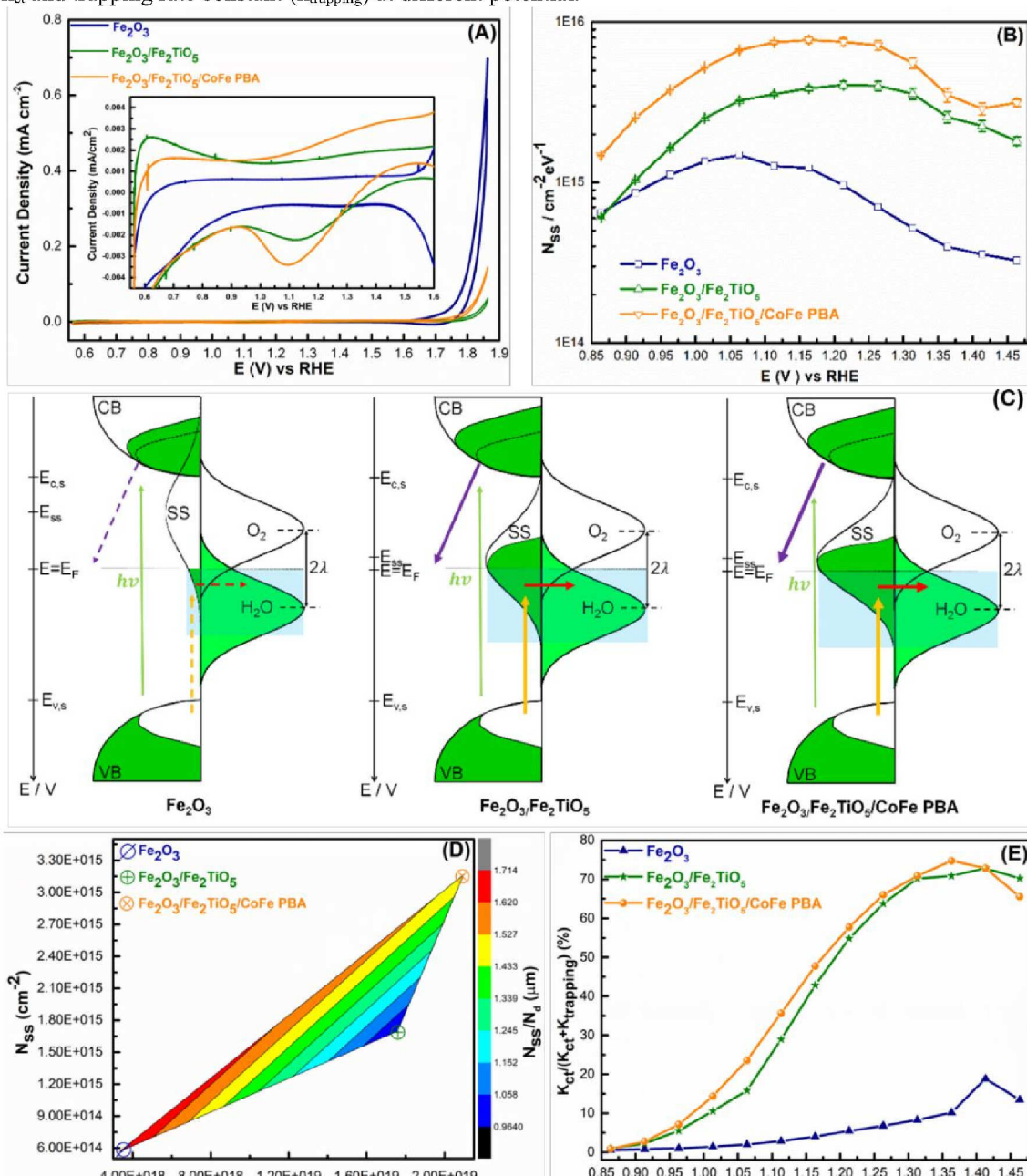
Figure 5. (A): CV curves scanned immediately in dark at 20 \text{ mV s}^{-1} after holding the electrode potential at 1.85 \text{ V vs. RHE} for 1 min under illumination. (The inset shows its magnified plot). (B): Density of surface states (DOSS) as a function of the applied potential. Error bars stem from the goodness of the EIS data fittings. (C) Kinetic scheme of the charge generation and transfer processes at SEI at 1.23 \text{ V vs. RHE} under illumination of these electrodes. Green and white areas represent electron filled and empty states, respectively. The dotted lines marked region in the CB filled states refer to photogenerated electrons with the same relative area as the empty states at the VB; the exceeding green regions highlight the doping levels in these electrodes. The green arrows denote the charge generation process upon photons absorption; the yellow arrows denote the hole trapping process at SS (surface states); the red arrows denote the hole transfer process from SS to electrolyte; the purple arrows denote to electron transfer from CB states to the FTO substrates. The thickness and shape of the arrows reveal the relative rates of the charge transfer processes, where the dotted lines mean the slowest rate ( \text{Fe}_2\text{O}_3 electrode) and the thickest lines means the fastest rate ( \text{Fe}_2\text{O}_3/\text{Fe}_2\text{TiO}_5/\text{CoFe-PBA} electrode). The light indigo shaded areas refer to the relative overlapping of the DOSS and water density of states. E: electrode potential; E_{c,s} : surface CB edge potential; E_F : Fermi level of the semiconductors that matches the electrode potential (E) and the \text{O}_2/\text{H}_2\text{O} couple thermodynamic potential ( 1.23 \text{ V vs. RHE} ); E_{ss} : center potential of the SS distribution; E_{v,s} : surface VB edge potential; \lambda : redox couple reorganization energy. It is worth noting that the relative size of the DOSS distribution for these electrodes has been intentionally enlarged to highlight the SS. (D): Total surface state density ( N_{ss} ), donor density ( N_d ), and their ratio ( N_{ss}/N_d ) plot. N_d was estimated from the slopes of the Mott-Schottky plots (Figure S30), whereas N_{ss} was obtained from integration of the DOSS profiles. Color bar with a unit of \mu\text{m} is plotted at the right Y axis for N_{ss}/N_d . (E): Ratio of the charge transfer rate constant ( k_{ct} ) and the sum of k_{ct} and trapping rate constant ( k_{trapping} ) at different potential.
