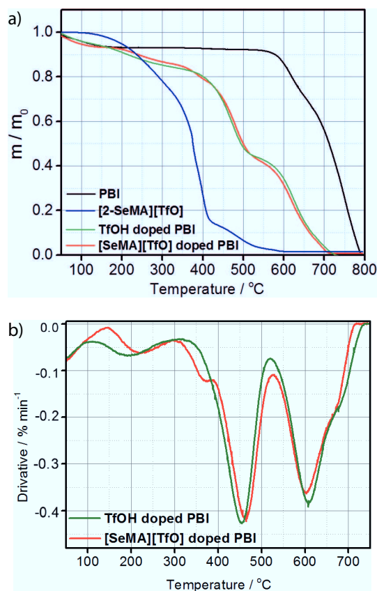
Fig. 6 The (a) TGA curves of m -PBI, [2-Sema][TfO], TfOH doped m -PBI (130 wt.%, m\text{-PBI-H}_2^+(\text{TfO})_2 \cdot 0.61\text{ TfOH} ) and [2-Sema][TfO]doped PBI (130 wt.%, m\text{-PBI-H}_2^+(\text{TfO})_2 \cdot 0.34\text{ [2-Sema][TfO]} ) and the (b) DTG curves of latter two.
