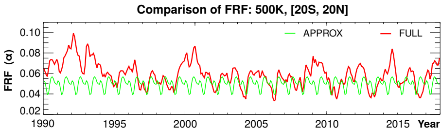
Figure 5.13: Comparison of FRF time series (1990-2017) calculated with the assumption of the instantaneous entry propagation (green line, APPROX) and with propagated entry CH 4 by the age spectrum (red line, FULL). Presented data is at 500 K averaged between 20° S-20° N.
