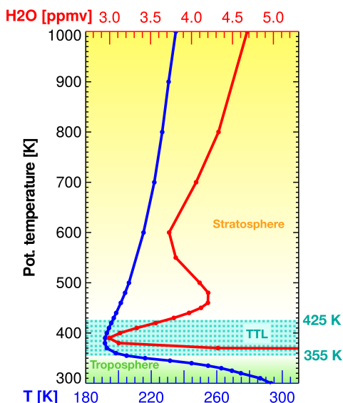
Figure 2.1: Temperature (blue line, [K]) and the \text{H}_2\text{O} mixing ratio (red line, [ppmv]) profile for the boreal winter season (DJF) climatologies (2004–2013 years) for the tropical region ( 20^\circ\text{S} – 20^\circ\text{N} ). The TTL is shown with the light blue area, whereas below, the troposphere is shown in green, and above, the stratosphere is shown in yellow colours. Note, that the temperature values are taken from ERA-Interim reanalysis, and the \text{H}_2\text{O} mixing ratios are from CLaMS simulation driven by ERA-Interim reanalysis.
