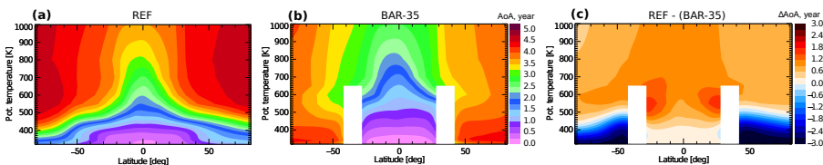
Figure 4.10: Zonal AoA distributions for 2011. Shown data are from the CLaMS reference simulation (a) and from the sensitivity simulation with barriers along latitude circles at 35° N/S (b) and the absolute difference between them (c). Transport barriers are set between the Earth’s surface and the 600 K potential temperature levels and are represented in white.
