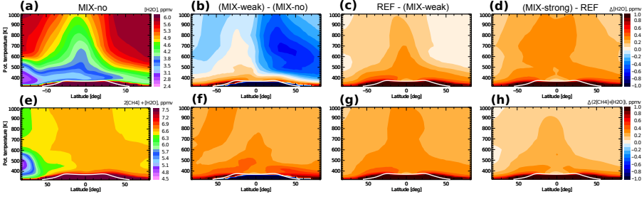
Figure 4.16: Annual zonal mean distributions of \text{H}_2\text{O} (a) and HH (e) from the CLaMS simulation without mixing (MIX-no), as well as the incremental differences between the sensitivity simulations with increasing mixing from the weak mixing case (MIX-weak) through the reference (REF) to the strong mixing case (MIX-strong); i.e. [(MIX-weak) - MIX-no] in the second column (b, f), [REF - (MIX-weak)] in the third column (c, g), and [(MIX-strong) - REF] in the fourth column (d, h). Tropopause is presented as white solid line, and is calculated from ERA-Interim reanalysis data. The data are shown for 2011.
