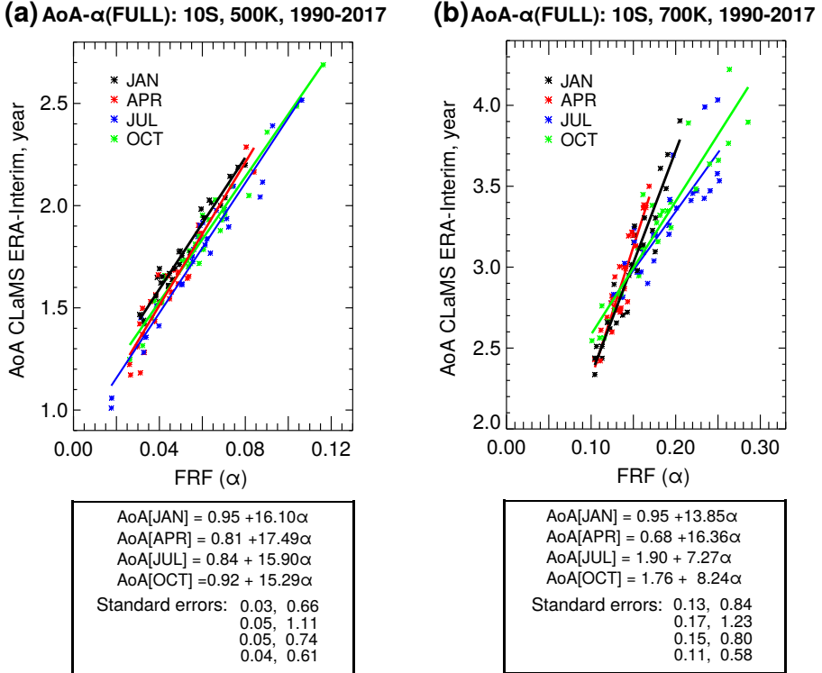
Figure C.2: Relationship between FRF (from FULL method) and CLaMS modelled AoA at the locations of 10^\circ \text{S} at 500 K (a) and 700 K (b) potential temperature. At each sub-figure are shown linear correlation functions depending on the month (January in black line, April in red line, July in blue line, and October is shown with green line). The correlation points are taken from the monthly data through all the years between 1990 and 2017. For each represented month, FRF and CLaMS (driven by ERA-Interim) AoA were taken as zonally averaged data in potential temperature range between 450 and 1000 K (where FRF has positive values due to the method). At this plot, the relationship is shown by fitting linear functions to the AoA-FRF distribution.
