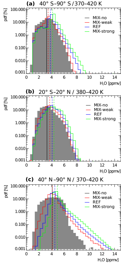
Figure 4.14: PDF for \text{H}_2\text{O} SH extratropics for 40° S–90° S between 370 K and 420 K (a), in the tropics for 20° S–20° N between 380 K and 420 K (b), and in the NH extratropics for 40° N–90° N between 370 K and 420 K (c). Shown data are from 2011 CLaMS sensitivity simulations with different strength of small-scale mixing for the case without mixing (MIX-no, grey shading background), weak mixing (MIX-weak, red solid line), reference simulation (REF, blue solid line) and strong mixing (MIX-strong, green solid line). Dashed coloured lines represent the mean \text{H}_2\text{O} values for the different simulations respectively, whereas the black solid line shows the mean value for the non-mixing case.
