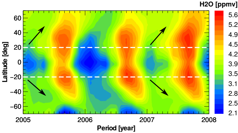
Figure 2.7: Horizontal tape recorder of \text{H}_2\text{O} in the LS at the potential temperature level of 390 K for the years from 2005 to 2008. Tropical region, 20^\circ\text{S} – 20^\circ\text{N} , is shown with the dashed white lines. The black arrows present the horizontal transport from the TTL to higher latitudes. Shown data are from CLaMS simulations, driven by ERA-Interim reanalysis.
