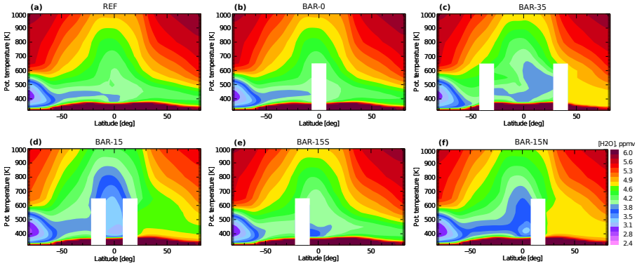
Figure 4.11: Zonal mean H 2 O distributions for 2011. Shown data are from the CLaMS sensitivity simulations for the reference (a) and the horizontal transport barrier simulations along latitude circles at 0° (b), 35° N/S (c), 15° N/S (d), 15° S (e) and 15° N (f). Transport barriers are set between the Earth's surface and the 600 K potential temperature levels and are represented in white.
