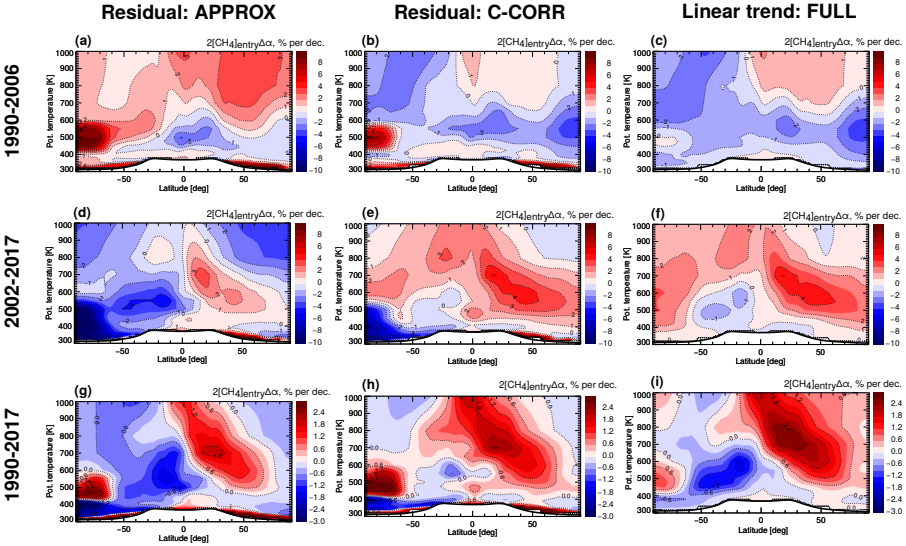
Figure 5.20: Circulation contribution ( 2\text{CH}_4[\text{entry}]\Delta\alpha ) estimated with three approaches: calculated as a residual in APPROX (a, d, g) and in C-CORR (b, e, h) methods, and as a linear trend in FULL method (using a linear fit with the least standard deviation at each latitude-potential temperature grid; c, f, i). The contributions are shown for three periods: 1990-2006 (a, b, c), 1990-2017 (d, e, f) and 2002-2017 (g, h, i). The data are shown in percentage per decade with respect to CLaMS \text{H}_2\text{O} climatologies from the considered period. The black line is the tropopause calculated from ERA-Interim. Below the tropopause, the white region indicates the areas, where the propagation procedure can not be applied.
