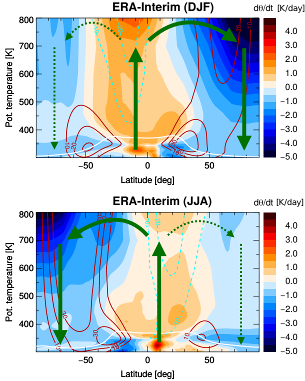
Figure 2.6: Zonally averaged diabatic heating rate distribution (in K/day) from climatologies for 2004-2013 from ERA-Interim for winter (DJF) and summer (JJA) periods. Dark red lines show zonal winds from 10 m/s to 30 m/s with an interval of 10 m/s, while blue dashed lines represent the negative zonal winds respectively. The white line is the tropopause. The green broad arrows highlight the main deep branches of BDC, whereas dashed arrows illustrate weaker circulation in the summer hemisphere. All data shown are taken from ERA-Interim reanalysis.
