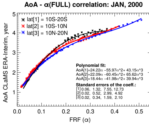
Figure C.1: Relationship between FRF (from FULL method) and CLaMS modelled AoA for January 2000, for three intervals of latitudes: between 10^\circ S and 20^\circ S (black line and black star-dots), 10^\circ S- 10^\circ N (red line and red star-dots), 10^\circ N- 20^\circ N (blue line and blue star-dots). For each interval, FRF and CLaMS (driven by ERA-Interim) AoA were taken as zonally averaged data between 450 and 1000 K (where FRF has positive values due to the method). At this plot, the relationship is shown by fitting third-order polynomial functions to the AoA-FRF distribution.
