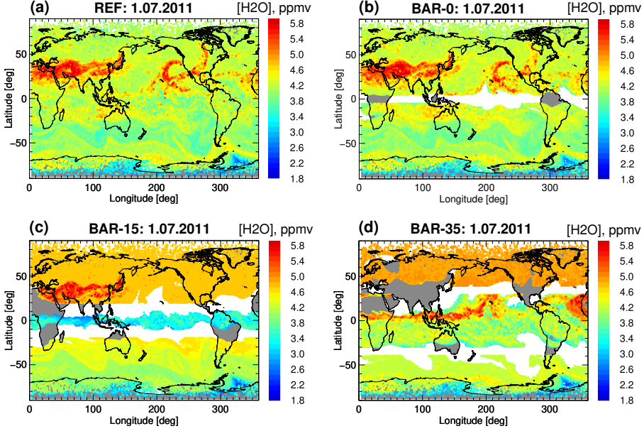
Figure 4.3: Maps of CLaMS APs distribution for the 1st of July 2011, at the potential temperature layer of 400 \pm 10 K: reference case (REF, a) and the sensitivity simulations with the horizontal transport barriers at the equator (BAR-0, b), at 15^\circ N/S (BAR-15, c) and at 35^\circ N/S (BAR-35, d). The colours of the APs respond to the CLaMS simulated \text{H}_2\text{O} mixing ratios. The transparent regions represent the areas without APs, including the artificial horizontal transport barriers.
