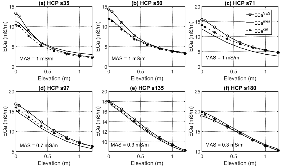
Figure B.4: Measured ECa ( \text{ECa}^{\text{mea}} ), and calibrated ECa using Gauss-Newton method ( \text{ECa}^{\text{cal}} ) and VES ( \text{ECa}^{\text{VES}} ) methods.
