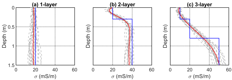
Figure B.2: Inversion results for the subsurface models with 0.1 mS/m noise added to the apparent electrical conductivity values. The grey dashed lines show the inversion results of twenty simulations, and the red solid lines represent their mean values.
