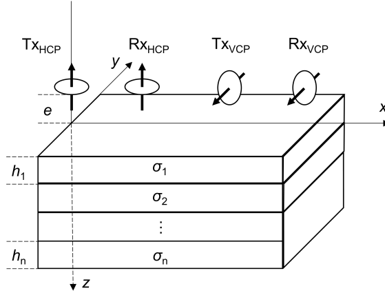
Figure 3.1: HCP and VCP configurations of the EMI system: a horizontal coplanar orientated transmitter-receiver pair ( Tx_{HCP} - Rx_{HCP} ) and a vertical coplanar orientated transmitter-receiver pair ( Tx_{VCP} - Rx_{VCP} ) placed at elevation e above a horizontally layered electrical conductivity ( \sigma_1, \dots, \sigma_n ) model. The lowest zone is a homogeneous half-space.
