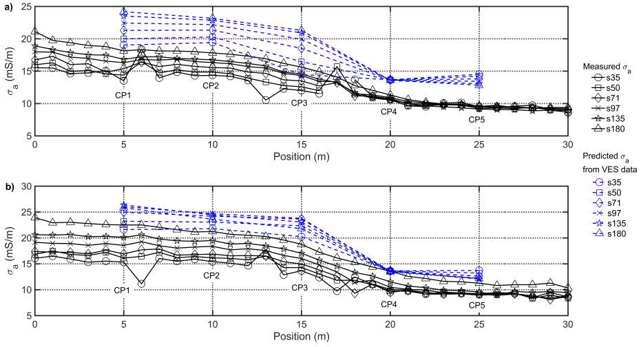
Figure 3.8: Measurements along the 30m long transect line on a bare-soil test field in Selhausen (North Rhine-Westphalia, Germany) for (a) VCP and (b) HCP configurations. Solid black lines with markers show ECa values ( ECa^{mea} ) obtained from each coil separation. The corresponding dashed blue lines with markers are the predicted ECa values ( ECa^{pre} ) obtained from inverted VES data at five selected calibration positions (CP1 to CP5) at 5, 10, 15, 20, and 25 m, respectively. Note that the predicted ECa values are used for the VES calibration.
