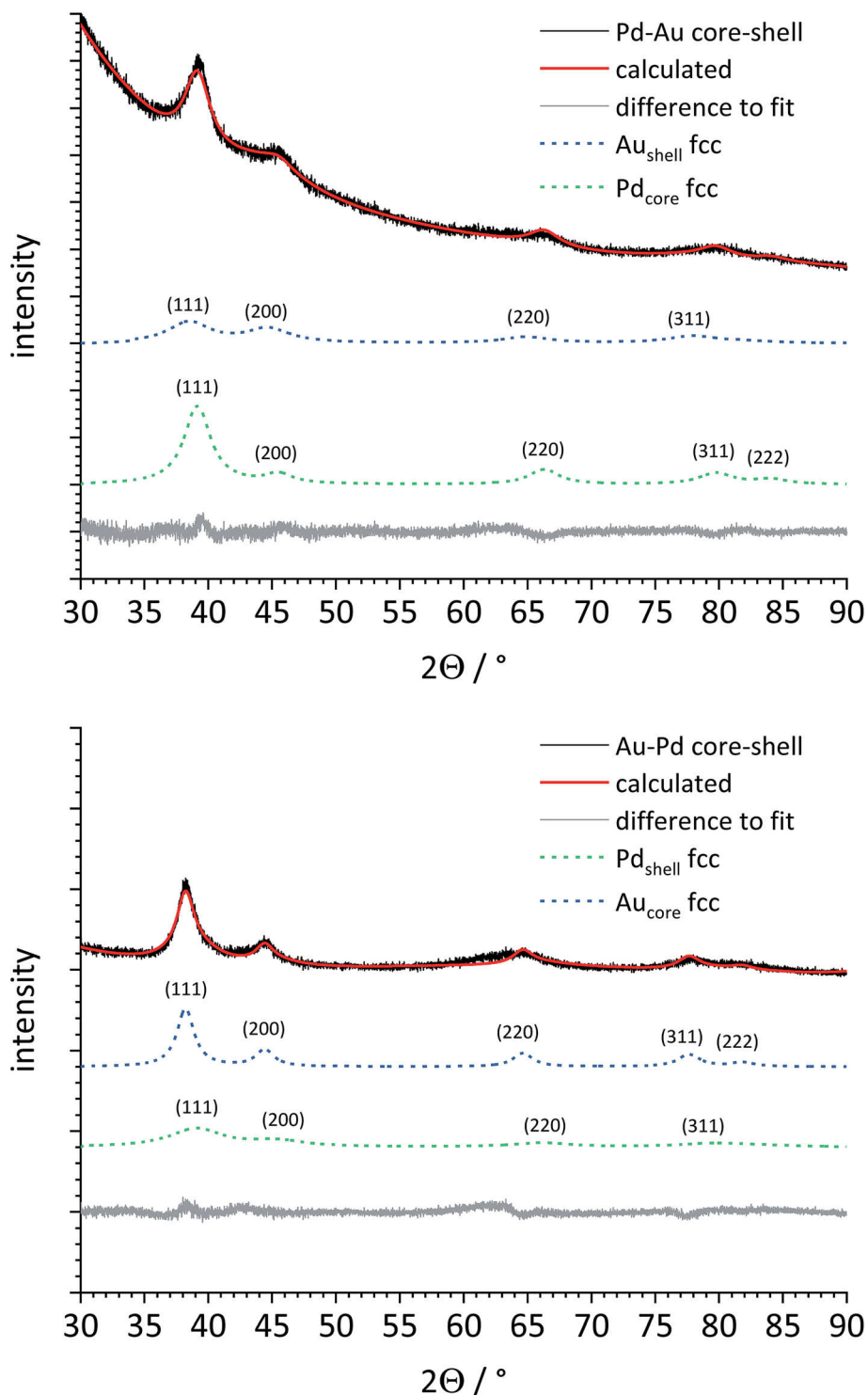
Fig. 7 X-ray powder diffraction patterns and Rietveld refinement of Pd–Au (top) and Au–Pd core–shell nanoparticles (bottom). The dashed lines for Au fcc and Pd fcc represent the baseline-corrected fits of these two metals. The core metal (Au or Pd) and the shell metal (Pd or Au) are well distinguishable in both cases. The bigger core size (5–6 nm) leads to narrower peaks for the core metal compared to the shell metal (shell thickness 1–2 nm).
