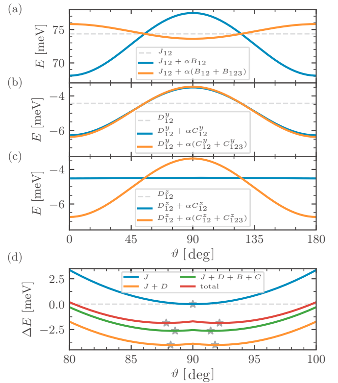
FIG. 4. Contributions to the energy of C_{3v} -symmetric magnetic structures of \text{Cr}_3 on Pt(111). (a) Effective isotropic interaction \tilde{J}_{12}(\theta) = J_{12} + \alpha(\theta)(B_{12} + B_{123}) . (b) y component and (c) z component of the effective chiral interaction vector \tilde{\mathbf{D}}_{12}(\theta) = \mathbf{D}_{12} + \alpha(\theta)(\mathbf{C}_{12} + \mathbf{C}'_{123}) . (d) Total magnetic energy per trimer atom relative to the energy of the planar Néel state ( \theta = 90^\circ ) given by J_{12} alone. The analytic form of the energy due to the isotropic and chiral interactions is given in Eq. (38). For each \theta , we consider the value of \phi that minimizes the energy. The last curve includes the contribution from the symmetric anisotropic interactions. The energy minima are indicated by the gray stars.
