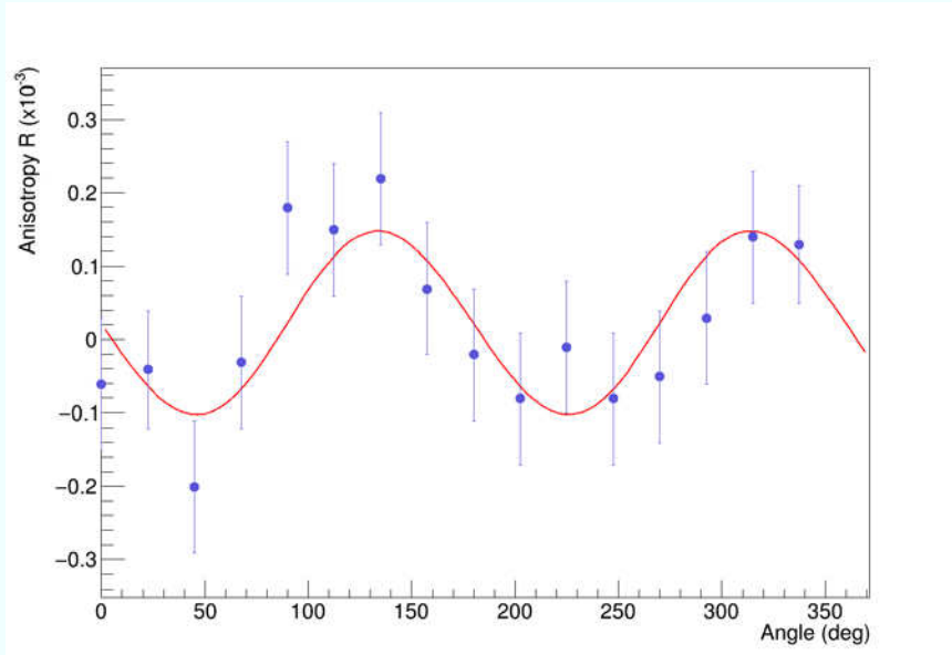
FIG. 4. Experimental angular dependence of the T-odd asymmetry coefficient R of \gamma -ray emission in ^{236}\text{U}^* fission.
