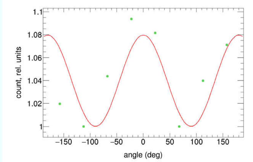
FIG. 3. Prompt \gamma -ray angular distribution. The curve is the result of approximation by Eq. (2).
