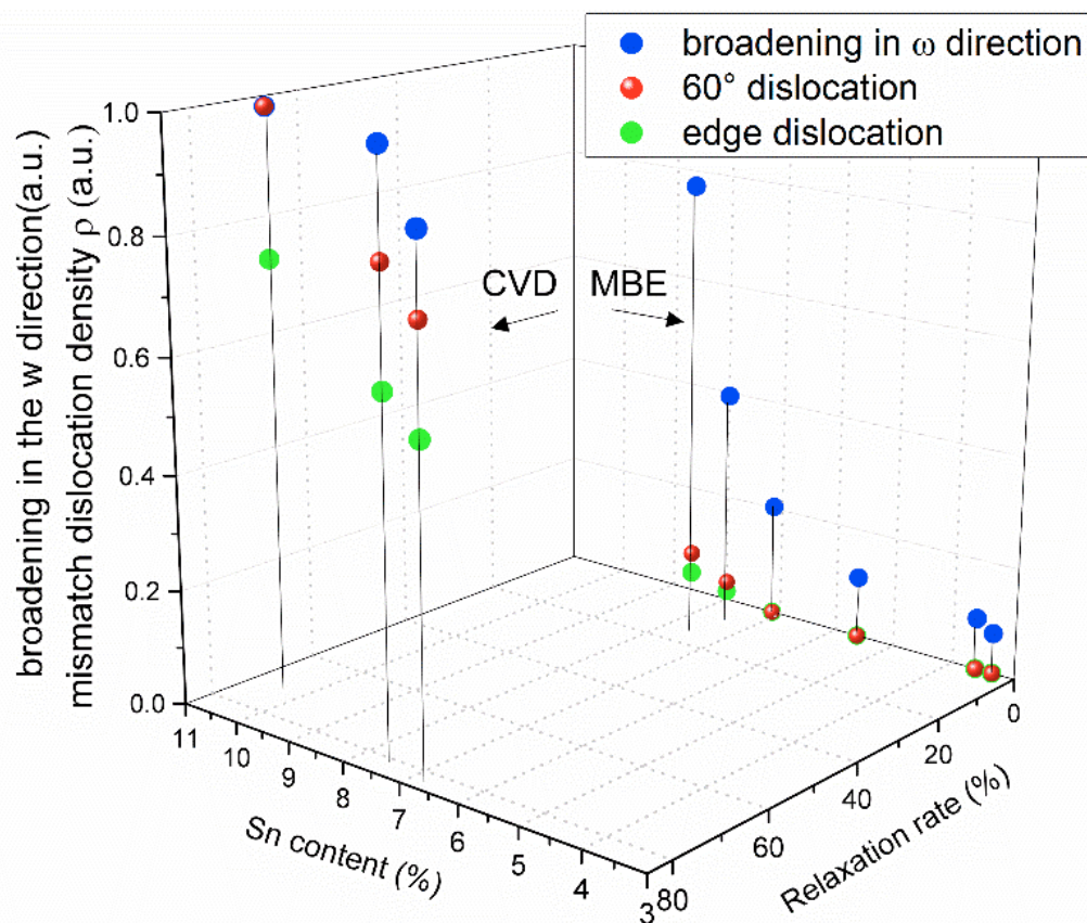
Figure 5. Normalized broadening in the \omega direction (blue), and the dislocation density calculated based on all 60° dislocation (red) and all edge dislocation (green) assumption with different Sn contents and relaxations.
