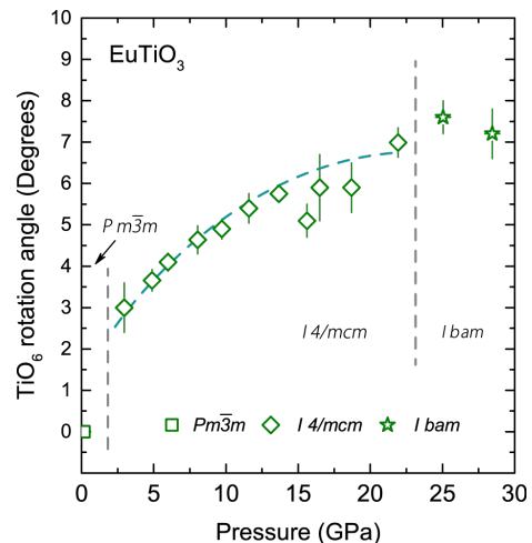
Figure 6: The relative rotation angle of the \text{TiO}_6 octahedra up to 30 GPa calculated in the structures identified in this study. The dashed line is a guide for the eyes.
