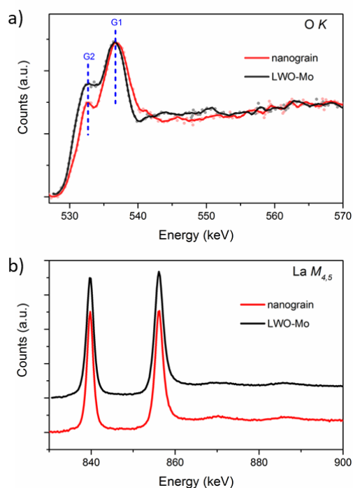
Fig. 4 EELS spectra showing the O K (a) and La M_{4,5} (b) edge recorded from the nanograin and the LWO-Mo. The spectra in (b) are offset in the vertical direction.
