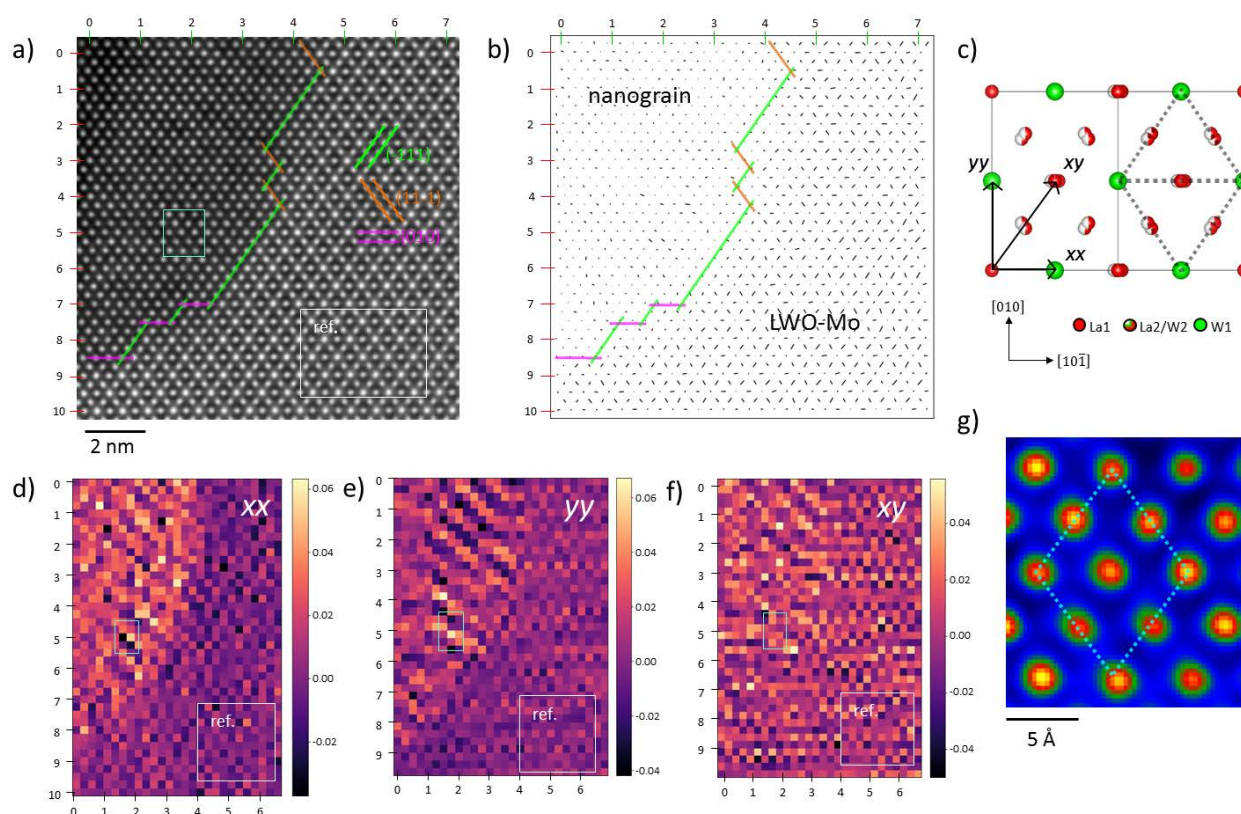
Fig. 5 Structural changes accompanying the grain boundary segregation. (a) HAADF image containing both LWO-Mo and the nanograin. Edge of the nanograin is indicated using relevant planes of LWO. The HAADF image is also scaled by the unit cell of LWO, as marked on the top and left. (b) Mapping the ellipticity of each atomic column in (a). (c) One unit cell of LWO oriented along [101] direction. (d-f) Strain maps estimated from (a), along xx , yy and xy directions as indicated in (c). The lower right part from LWO-Mo was used for reference, and the maps are scaled by the LWO unit cell. (g) Color-coded HAADF image cropped from the left rectangle region in (a).
