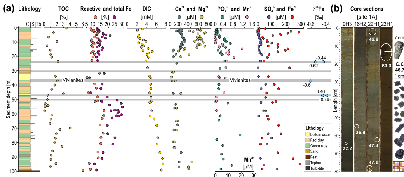
Figure 2. Stratigraphy of composite site TDP-1A: multiple profiles established on sediment core subsamples and core section images. (a) Stratigraphy of composite site TDP-1 (following Russell et al., 2016) and corresponding grain sizes (C: clay; S: silt; Tb: turbidite); total organic carbon (TOC) and reactive and total iron (weight %) in bulk sediment; dissolved inorganic carbon (DIC) (mM), calcium, magnesium, phosphate, manganese, sulfate, and ferrous iron concentrations (μM) measured in pore water; and δ 56 Fe isotopic compositions of vivianite crystals. (b) Images of core sections from which vivianite crystals were handpicked. Crystals on the far right were extracted from core catchers.
