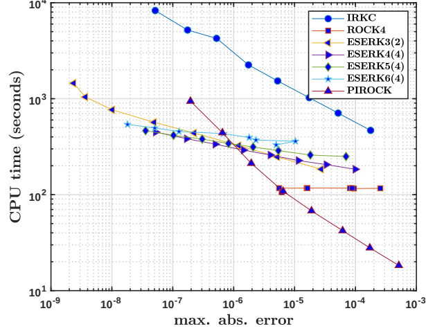
Figure 4: Maximal absolute error versus CPU times in seconds for the second example using ROCK4, IRKC, PIROCK, ESERK3, ESERK4, ESERK5 and ESERK6.
