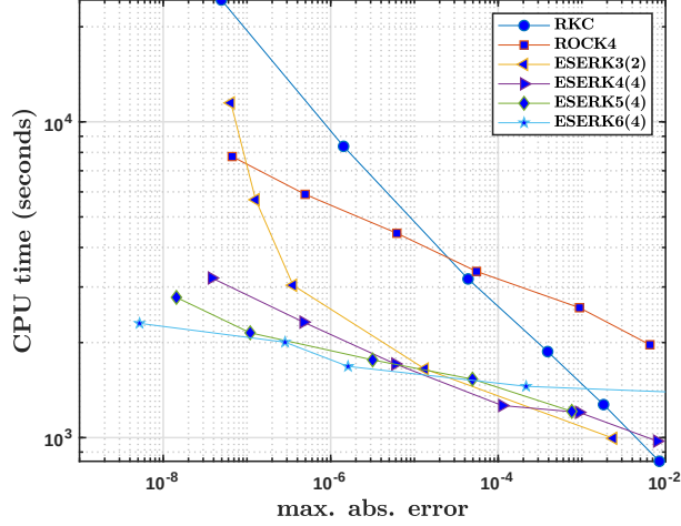
Figure 2: Maximal absolute errors versus CPU times in seconds for the second example using RKC, ROCK4, ESERK3, ESERK4, ESERK5, and ESERK6.
