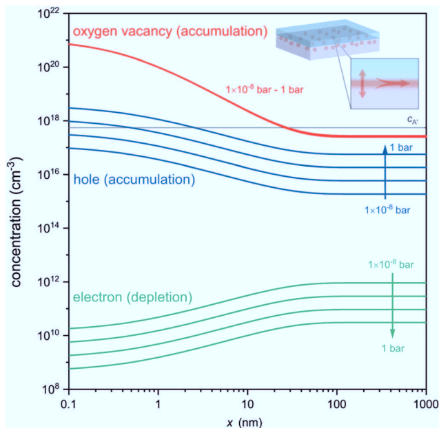
Fig. 4 Defect concentration profiles at the p-type LaAlO 3 /SrTiO 3 interface calculated for different oxygen pressures. The accumulation layer of oxygen vacancies (red lines) is robust against a variation of p\text{O}_2 , and exceeds the hole concentration (blue) as well as the impurity concentration (gray line) by orders of magnitude.
