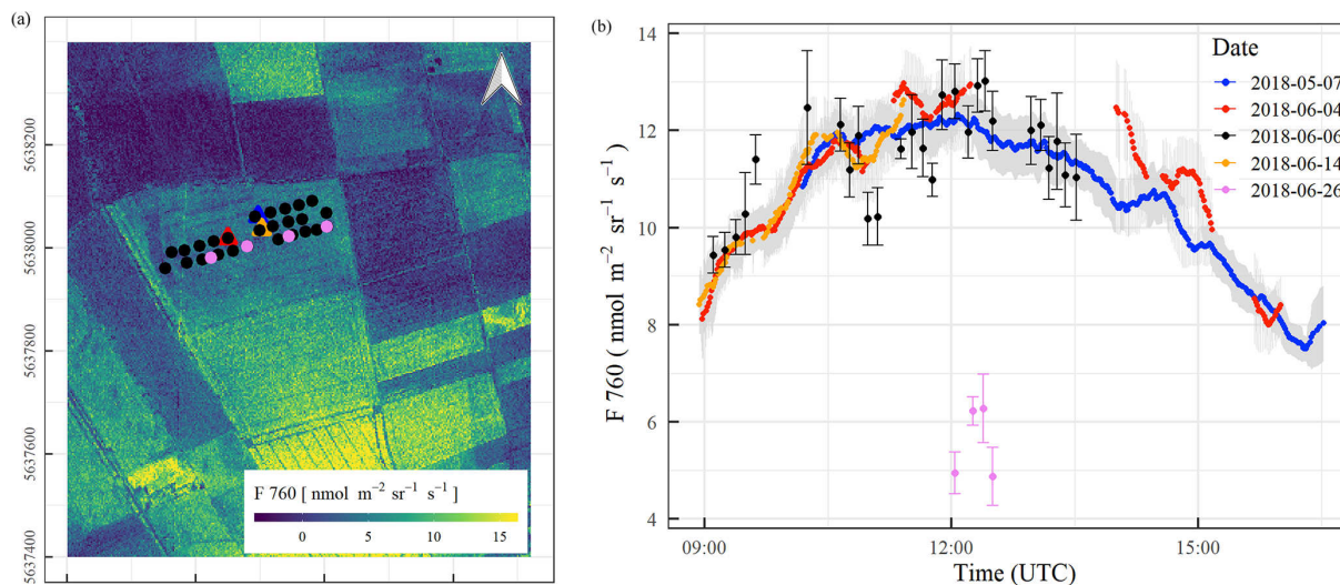
Figure 13. (a) Aerial map of F_{760} on 26 June 2018 with measurement locations used to combine with mobile (circles) and stationary (triangles) measurements. (b) Diurnal changes in F_{760} on different days of the campaign as 5 min measurement averages depicted in the same colours as observation locations in (a).
