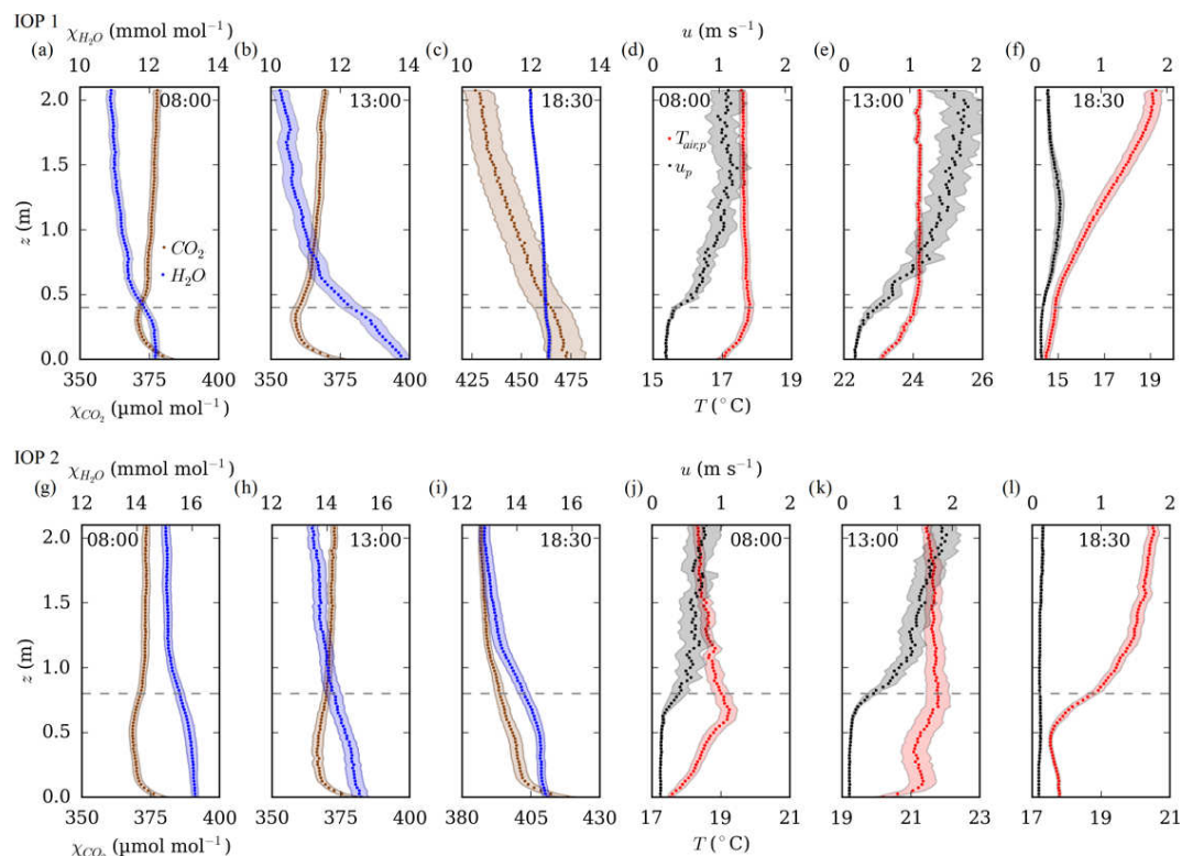
Figure 7. Selected (08:00, 13:00 and 18:30 UTC) 30 min mean profiles of the H_2O and CO_2 mole fractions ( \chi_{H_2O} , \chi_{CO_2} ), wind speed ( u_p ), and temperature ( T_{air,p} ) measured at high vertical resolution during IOP 1 (upper row) and IOP 2 (lower row). Shaded areas indicate the 95 % confidence interval resulting from the standard deviation between individual profiles sampled within a 30 min average interval. The dashed lines indicate the canopy heights.
