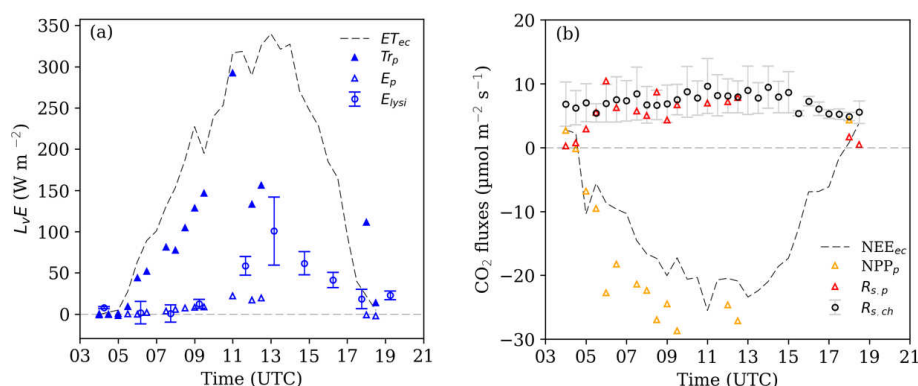
Figure 9. Source partitioning results for (a) H 2 O and (b) CO 2 fluxes for IOP 1. Dashed grey lines show the measured latent heat flux ( ET_{ec} ) and net ecosystem exchange ( NEE_{ec} ) in half-hourly time steps. Values with subscript index p indicate estimates based on inversed profile concentration measurements (Sect. 3.4). Error bars for evaporation calculated from microlysimeters ( E_{lysi} ) and soil respiration measurements ( R_{s,ch} ) indicated to 1 SD. ( ET_{ec} : evapotranspiration measured as latent heat flux L_v E by the eddy covariance system; E : evaporation; Tr_p : transpiration; NPP : above-ground net primary production; R_s : soil respiration).
