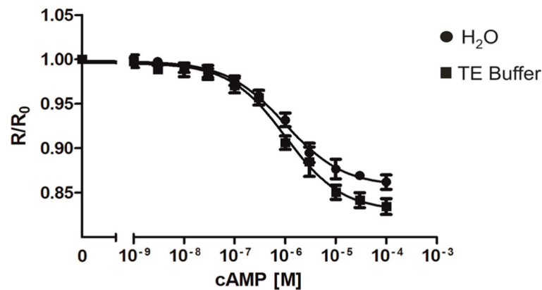
Fig. 4 Change of cAMP-dependent Epac1-camps-His 6 fluorescence using desiccated and re-constituted samples. Purified Epac1-camps-His 6 protein was diluted to a concentration of 0.7 \mu M in IS buffer, transferred to all wells of a 96 MWP, and desiccated in a fridge. Protein in 48 wells was reconstituted in bi-distilled H 2 O and protein in the remaining wells was reconstituted in TE-buffer. This design allowed simultaneous four-fold measurements. Excitation was at 430 nm and emission was recorded at 475 nm (ECFP) and 530 nm (EYFP). After recording the basal fluorescence for ECFP and EYFP, increasing concentrations of cAMP were added. The EYFP/ECFP ratio (R) for each well was calculated and normalized to the ratio of the basal fluorescence in the absence of cAMP (R 0 ). Normalized data (mean values \pm SD) were plotted against cAMP concentrations. EC 50 values were calculated with a four-parameter nonlinear regression using GraphPad Prism v5.04. A representative of two independently performed experiments is shown
