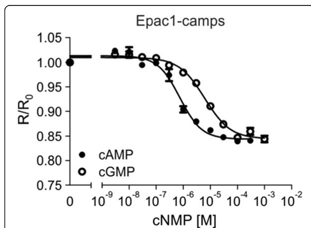
Fig. 1 Characterization of Epac1-camps-His 6 in multi-well plates. Purified Epac1-camps-His 6 protein was diluted to a concentration of 0.7 \mu M in IS buffer and 90 \mu l of the sample was added to each well of a 96 multi well plate. Excitation was at 430 nm and emission was recorded at 475 nm (ECFP) and 530 nm (EYFP). After recording the basal fluorescence for ECFP and EYFP, increasing concentrations of cAMP or cGMP were added to each well. The final volume was 100 \mu l and final concentrations of cyclic nucleotides ranged from 10^{-9} - 10^{-4} M. The EYFP/ECFP ratio (R) for each well was calculated and normalized to the ratio of the basal fluorescence in the absence of cyclic nucleotides ( R_0 ). Normalized data were plotted against cyclic nucleotide concentrations. Each data point is given as mean value ( \pm SD) from four identically treated wells of a representative experiment. EC_{50} values were calculated with a four-parameter nonlinear regression using GraphPad Prism v5.04
