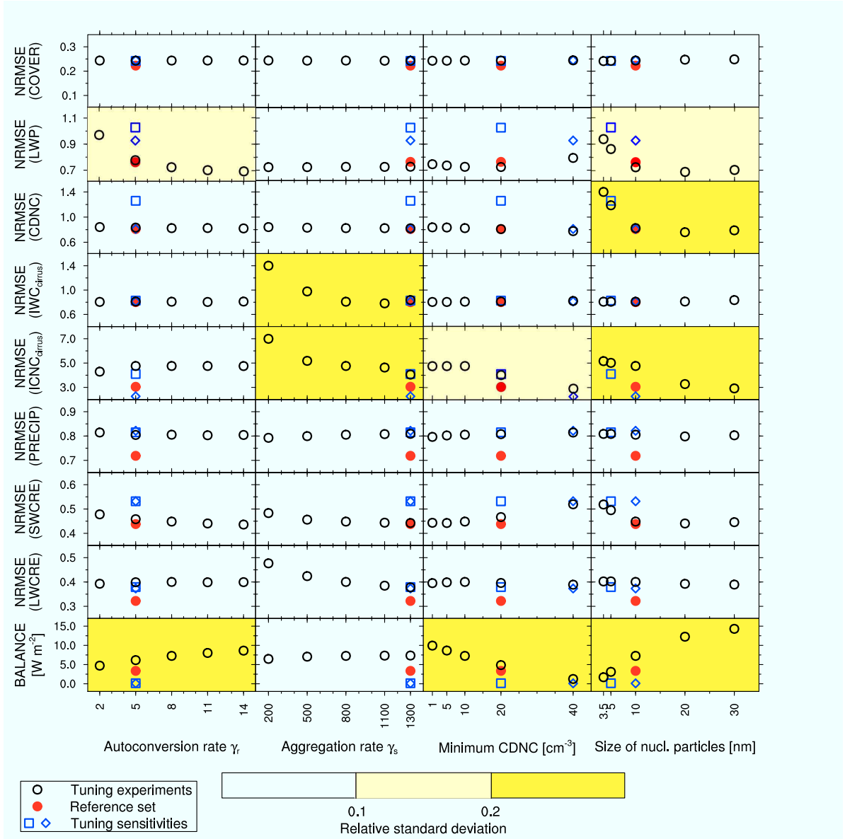
Figure 1. NRMSE of selected cloud and radiation variables in the tuning experiments, together with the resulting model top-of-the-atmosphere radiative balance (in \text{W m}^{-2} ). Each column represents a tuning parameter and shows the NRMSE for the five tuning simulations (black circles) performed to explore the effects of its variation, while keeping the others fixed at their central value (note that for the radiative balance the actual value and not the NRMSE is shown). The red circle represent the results for the reference set of tuning parameters ( \gamma_r = 5 , \gamma_s = 1300 , \text{CDNC}_{\min} = 20 \text{ cm}^{-3} , and d_{\text{nuc}} = 10 \text{ nm} ), while the blue square and diamond show the results of two additional sensitivity runs to further explore the variation on \text{CDNC}_{\min} and d_{\text{nuc}} . The NRMSE is calculated with respect to the observations given in Table 2. The yellow shadings represent the relative standard deviation of the NRMSE within each panel. For SWCRE, the absolute value of the NRMSE is shown for more clarity (since it is negative via the normalization).
