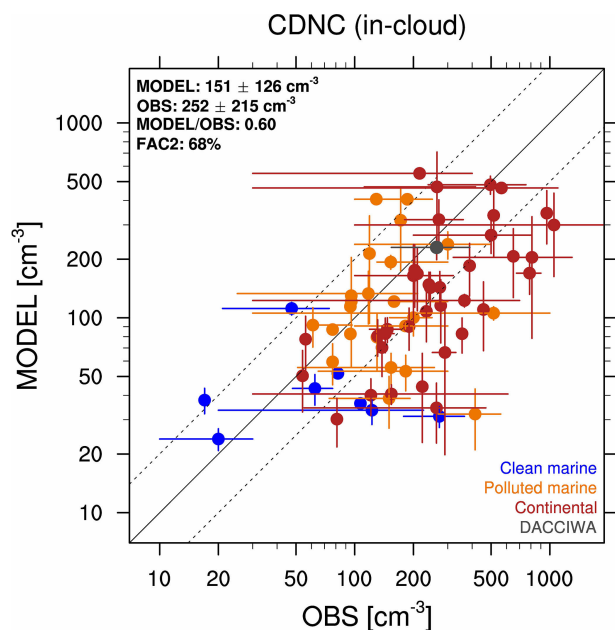
Figure 3. Scatterplot of simulated (vertical) vs. observed (horizontal) CDNC based on various satellite and in situ measurements collected by Karydis et al. (2011, 2017). Different colors represent different groups of measurement locations: clean marine (blue), polluted marine (orange), and continental (red). A further comparison with the mean of 12 flights performed during the Dynamics-Aerosol-Chemistry-Cloud interactions in West Africa (DACCWA) campaign (Flamant et al., 2018) is shown in gray. The horizontal bars represent the range of reported values, while for the DACCWA campaign it spans the range of the means from all flights. The vertical bars show the standard deviation in the model interannual variability. The mean and standard deviation of model and observations are shown in the top left, together with their ratio and the percentage of points within a factor of 2 of the observations (FAC2, i.e., factors between 0.5 and 2), also indicated by the dashed lines.
