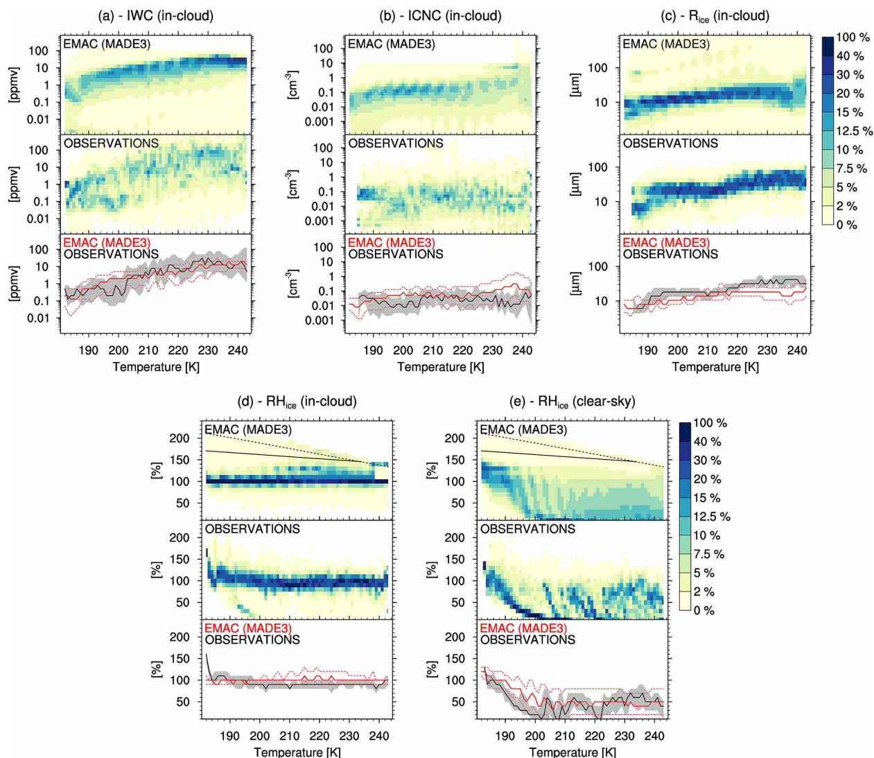
Figure 5. Climatology of various cirrus properties derived from flight campaigns as compared with EMAC (MADE3) simulations: in-cloud ice water content ( a ), in-cloud ice crystal number concentration ( b ), ice crystal mean-volume radius ( c ), in-cloud ( d ) and clear-sky ( e ) relative humidity with respect to ice. The data are plotted as probability distribution functions in 1 K temperature bins in the model (top plot in each panel) and in the observations (middle plot). The bottom plots in each panel show the median (solid red line) and the 25/75 % quantiles (dashed red) of the model compared with the median (solid black line) and the 25/75 % quantiles (gray shading) of the observations. The dashed and solid black lines on the relative humidity panels ( d , e ) represent the water saturation and the homogeneous freezing threshold (Koop et al., 2000), respectively.
