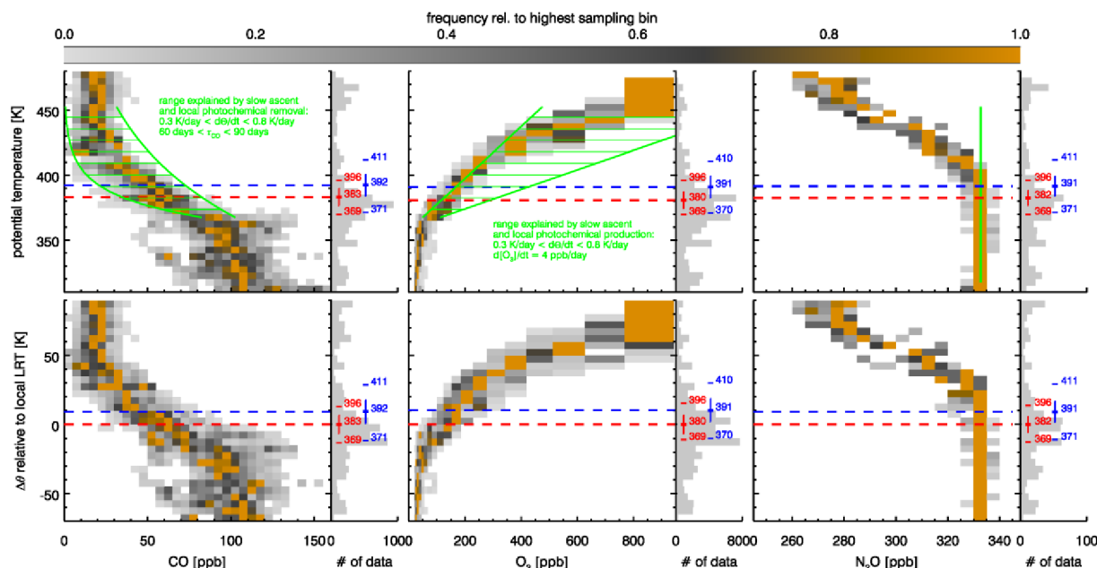
Figure 4 Layer-normalized relative frequency distributions of CO (left), O 3 (middle) and N 2 O (right) inside the ASM anticyclone (MeqLat > 65 °) for vertical coordinates of potential temperature (top) and potential temperature difference relative to the local LRT (bottom). The number of observations on each vertical level is plotted along the right side of each panel. The mean (with standard deviation), minimum and maximum LRT and CPT levels are also shown in red and blue, respectively. Areas marked in green in the CO and O 3 panels indicate the range of concentrations consistent with photochemical removal/production during slow ascent (assuming isentropic ascent rates between 0.3 and 0.8 K day -1 , based on Ploeger et al., 2010, and Garny and Randel, 2016; a CO photochemical lifetime between 60 and 90 days based on Xiao et al., 2007; and O 3 production rates of about 4 ppb day -1 based on Fig. 8 in Gottschaldt et al., 2017). In the N 2 O panel, the green line denotes the average HAGAR N 2 O in the troposphere (below 360 K potential temperature) during the 2017 campaign.
