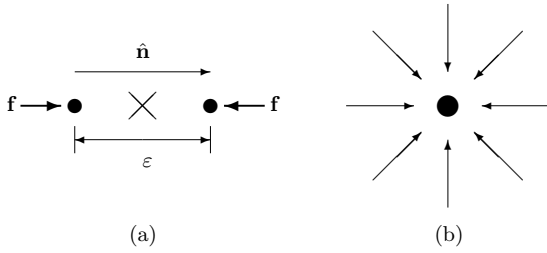
FIG. 2. (a) A single contractile force dipole of size \varepsilon , force f , and orientation \hat{n} . (b) Schematic representation of an isotropic compression center as the orientational average of (a).
