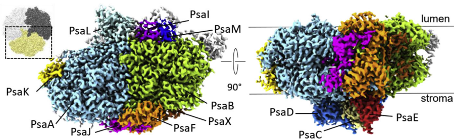
Fig. 1. Cryo-EM structure of the monomeric TePSI crosslinked to Cyt c 6 derived from the symmetry expanded dataset shown from the luminal side (left) and from along the membrane plane (right). The inset on the far left shows the position of the monomer in the PSI trimer as seen from the luminal side.
