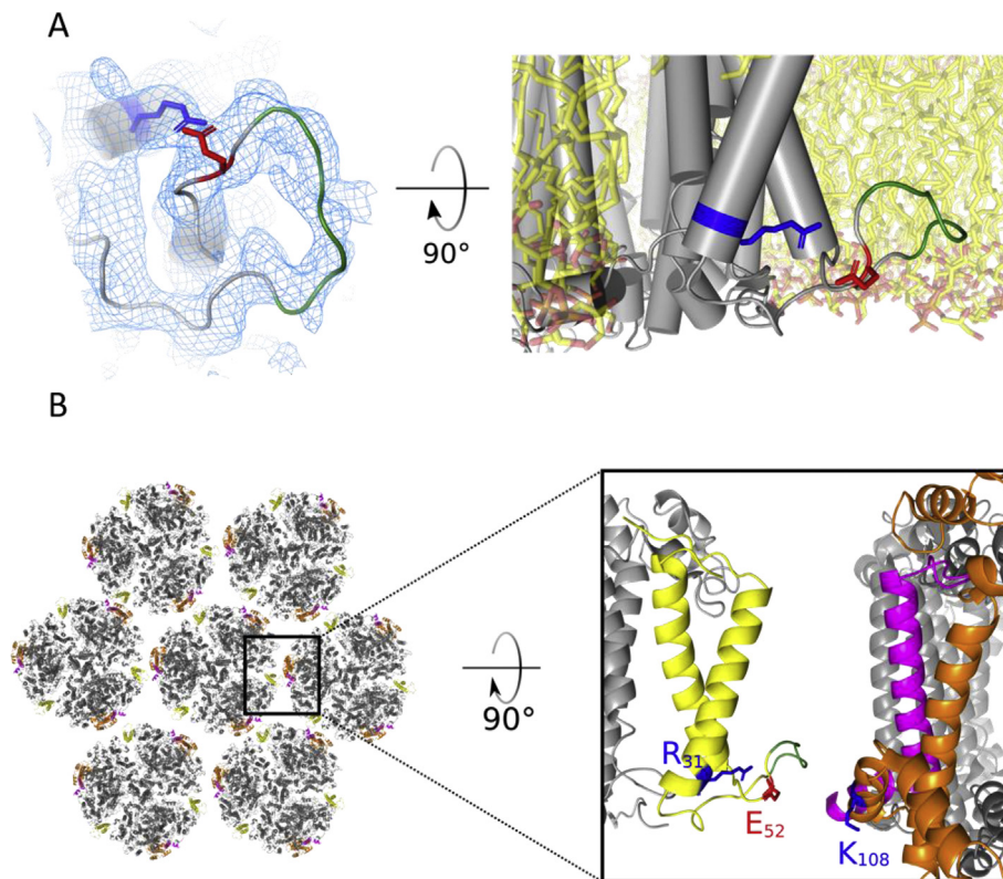
Fig. 3. The structure of Psal loop 32–55. A , View onto cytoplasmic side of the model with symmetry expanded monomeric EM map displayed as blue mesh (left) and view from membrane onto the same section of Psal with modelled palmitoylphosphatidylglycerol (POPG)-membrane (right). The PIALPAL-patch 44–50 is highlighted in green, and the salt bridge-forming residues Arg31 and Glu52 are coloured blue and red, respectively. POPG membrane was simulated using CHARMM membrane builder (Jo et al., 2008). The map is plotted at a B-factor of -173 \text{ \AA}^2 . B , Model of trimer-trimer interface of T. elongatus thylakoid membrane. Hexagonal packing of PSI trimers (left) is based on the AFM images as shown in (MacGregor-Chatwin et al., 2017). Close up of the interface between two neighbouring trimers (right). The subunits at the interface are Psal (orange), Psal (magenta) and Psal (yellow). The PIALPAL-patch 44–50 of Psal is highlighted in green. Psal Glu52 (red), Arg31 and Psal Lys108 (blue) are shown in stick representation.
