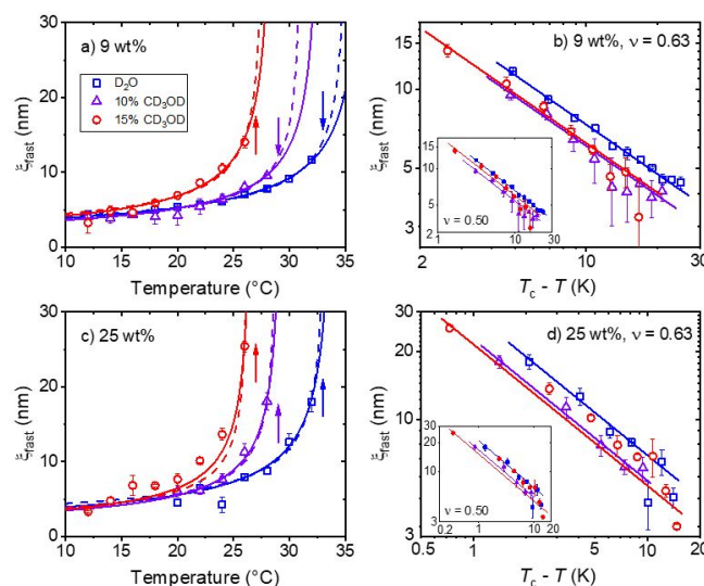
Figure 5. (a) Temperature dependent dynamic correlation length \xi_{\text{fast}} from DLS for the fast mode of all solutions at a polymer concentration of 9 wt% (a, b) and 25 wt% (c, d) and the CD 3 OD contents given in (a). The dashed and full lines in (a) and (c) are fits of eq. 8 with \nu fixed at values of 0.50 or 0.63, respectively. The arrows mark the cloud points T_{\text{cp}} . (b, d) Same data as in (a, c), plotted in a double-logarithmic representation of vs. T_c - T including the fitting curves, using the values of the fitting parameters obtained for \nu = 0.63 . The insets in (b) and (d) show the same data along with fits of eq. 8 with the exponent \nu being fixed at 0.50.
