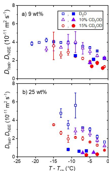
Figure 4. Temperature-dependent diffusion coefficients in dependence on T - T_{\text{cp}} for polymer concentrations of (a) 9 wt% and (b) 25 wt%. The solvent compositions are given in (a). Open symbols: values from the fast mode in DLS, closed symbols: values from NSE.
