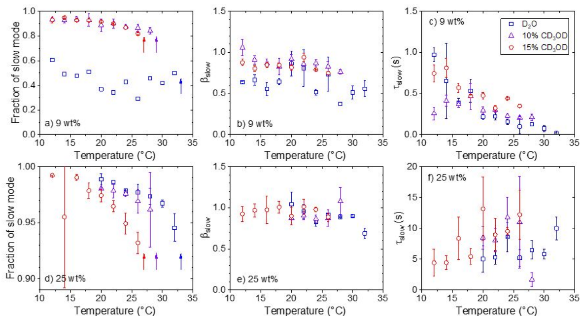
Figure 2. Characteristics of the slow mode in the DLS autocorrelation functions for PNIPAM concentrations of (a-c) 9 wt%, (d-f) 25 wt%. (a, d) Fraction of the slow mode at a scattering angle of 90^\circ , (b, e) stretching exponent \beta_{\text{slow}} and (c, f) relaxation time \tau_{\text{slow}} in dependence on temperature at the \text{CD}_3\text{OD} contents given in (c) For the sample with 9 wt% in pure \text{D}_2\text{O} , \langle \tau_{\text{slow}} \rangle is shown, calculated using eq. 2. The arrows in (a, b) indicate the cloud points T_{\text{cp}} .
