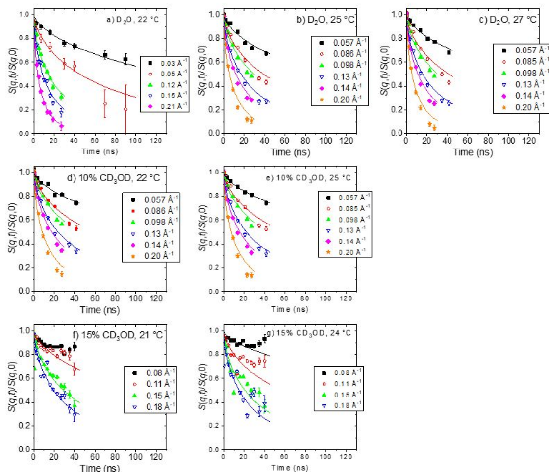
Figure 7. Representative intermediate scattering functions S(q,t)/S(q,0) from NSE on the solutions having polymer concentrations of 25 wt% in pure D_2O (a-c) or containing 10 % (d,e) or 15 % CD_3OD (f,g) at the temperatures and q values given in the graphs. Lines are fits of stretched exponentials as described in the text.
