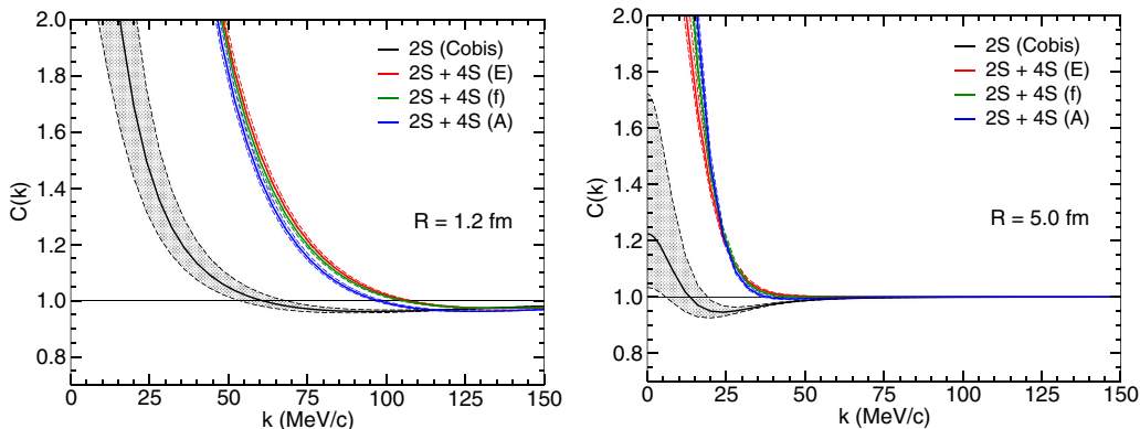
FIG. 4. \Lambda d correlation functions for the source sizes R = 1.2 and 5 fm, based on the {}^2S_{1/2} effective range parameters of Cobis [56]. Same description of curves as in Fig. 1.
