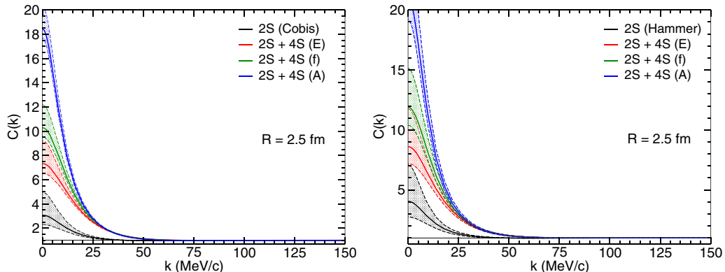
FIG. 2. \Lambda d correlation functions for the source size R = 2.5 fm. Same description of curves as in Fig. 1.
