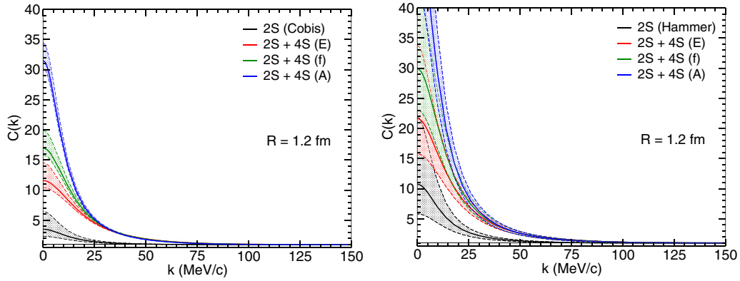
FIG. 1. \Lambda d correlation functions for the source size R = 1.2 fm. Spin-averaged results are shown wherein the ^2S_{1/2} state either the ERE parameters of Cobis [56] (left) or of Hammer [60] (right) are employed. For the ^4S_{3/2} state results from Schäfer [62] are used, building on \Lambda N scattering lengths from Alexander (A) [2], NSC97f (f) [73], or chiral EFT (E) [19] (from top to bottom), see text. The bands are the error due to the uncertainty in the ^3_\Lambda\text{H} binding energy.
