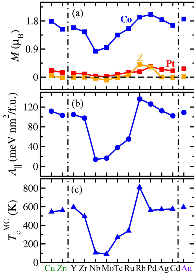
FIG. 3. (a) Magnetic moments of Z, Co, and Pt atoms, (b) spin-stiffness constant A_{||} , extracted from spin-spiral vectors \mathbf{q} along the \overline{\Gamma\text{M}} ( \overline{\text{AL}} ) direction, and (c) critical temperature for magnetic ordering of Z/Co/Pt ( Z = 3d : Cu, Zn; 4d : Y–Cd; 5d : Au) MMLs at the related FM (SAF) equilibrium state.
