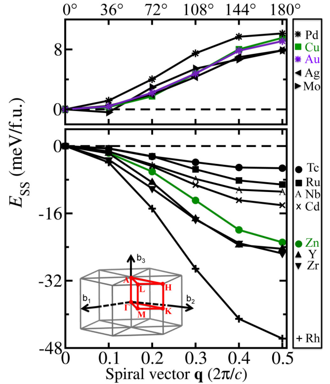
FIG. 4. Energy dispersion of spin spirals in Z/Co/Pt ( Z = 3d : Cu, Zn; 4d : Y–Cd; 5d : Au) MMLs for spin-spiral vectors \mathbf{q} along the \overline{\Gamma\text{A}} direction to explore the interlayer exchange coupling. The inset shows the Brillouin zone of the hexagonal lattice. \mathbf{b}_1 , \mathbf{b}_2 , and \mathbf{b}_3 represent reciprocal lattice vectors for the chemical unit cell.
