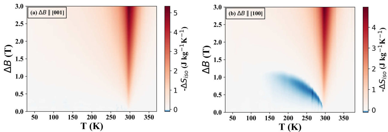
FIG. 7. Color plot of the magnetic entropy change of \text{Mn}_5\text{Ge}_3 as a function of temperature and magnetic field change parallel to [001] and [100]. Blue colors indicate a positive \Delta S_{\text{iso}} and hence an inverse MCE; red colors correspond to a negative \Delta S_{\text{iso}} and hence normal MCE.
