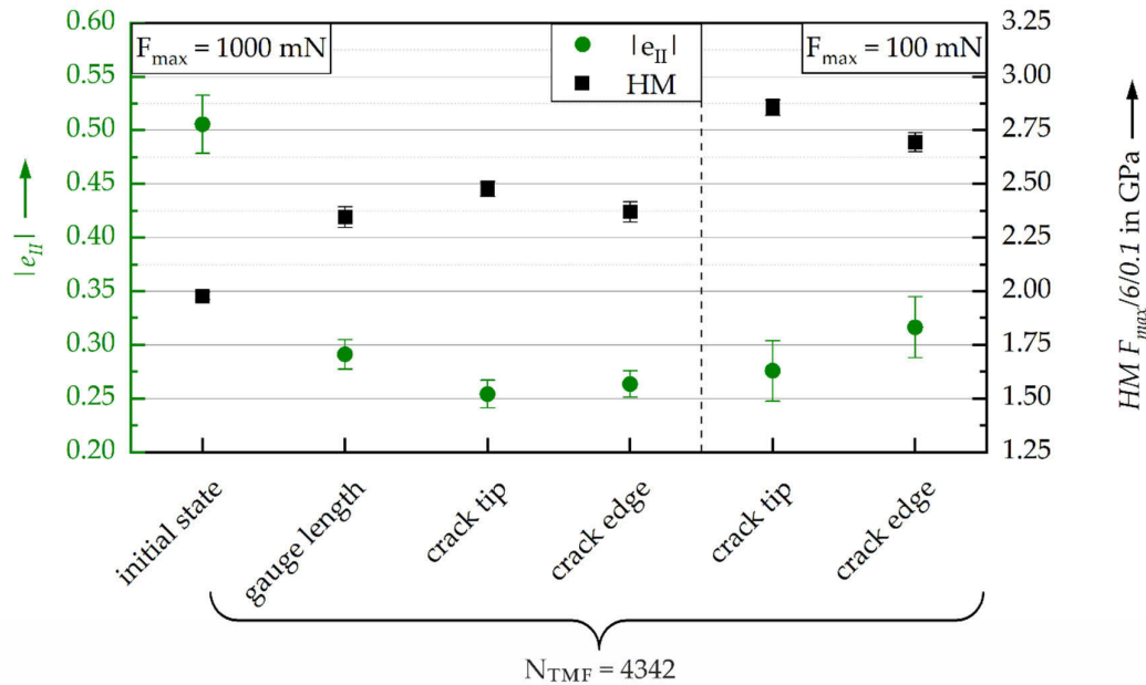
Figure 7. Cyclic hardening exponent |e_{II}| and martens hardness HM at the volume of the gauge length, crack edges and plastic zone in front of the crack tip at a fatigue crack observed at a Crofer®22 H specimen loaded for 4342 TMF-cycles.
