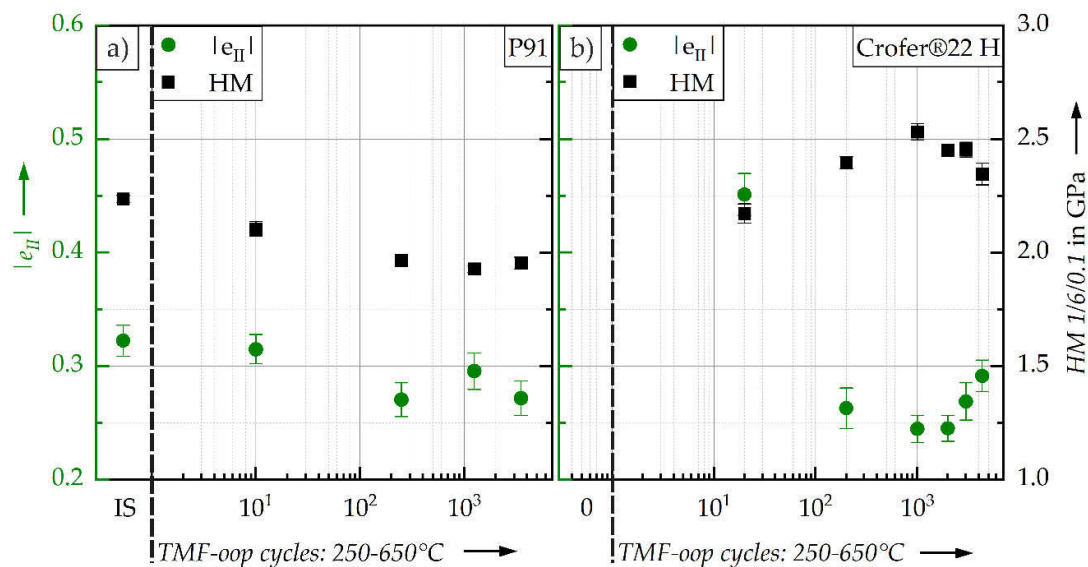
Figure 5. Cyclic hardening exponent |e_{II}| and martens hardness HM of the initial state (IS) and subject to TMF-cycles for (a) P91 and (b) CroFer®22 H.
