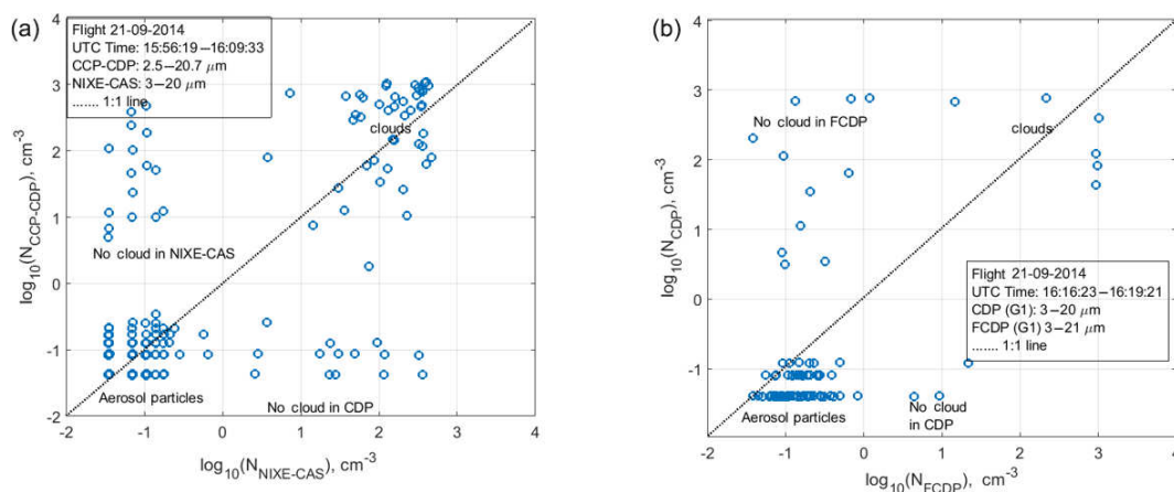
Figure 14. The comparison of cloud droplet concentrations in the same aircraft (a) between NIXE-CAS and CCP-CDP aboard HALO; (b) between CDP and FCDP aboard the G1.
