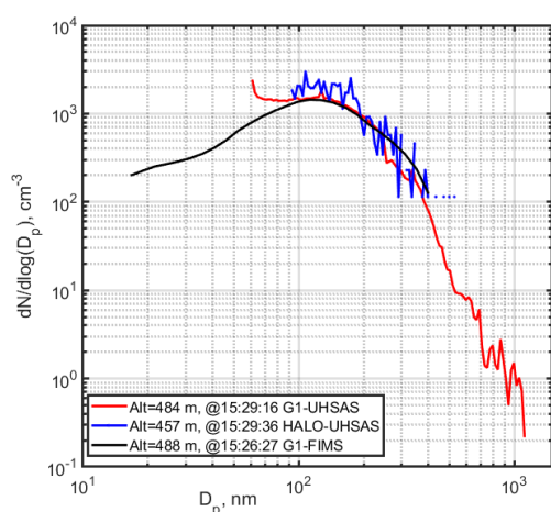
Figure 9. The G1 and HALO comparison for aerosol size distribution measured by UHSAS (from both aircraft) and FIMS (on the G1) on 9 September.
