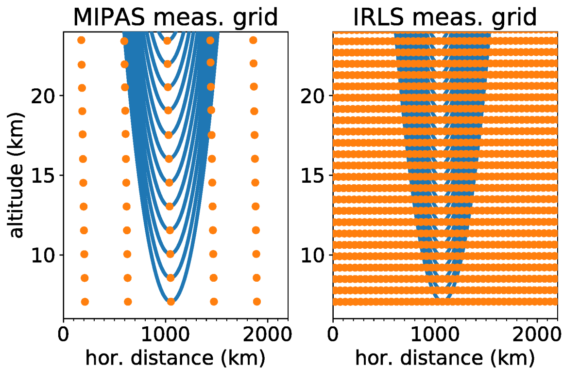
Figure 1. The measurement grid of a MIPAS-like instrument (left panel) and the IRLS (right panel). The blue lines indicate the line-of-sights of a single profile. The orange dots indicate the tangent points of multiple adjacent profiles 2100 km along-track.
