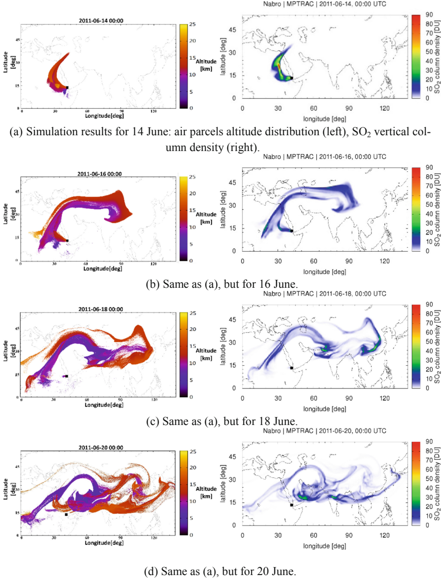
Fig. 5. Final forward simulation results of volcanic \text{SO}_2 released by the Nabro eruption. The black square indicates the location of the Nabro volcano.
