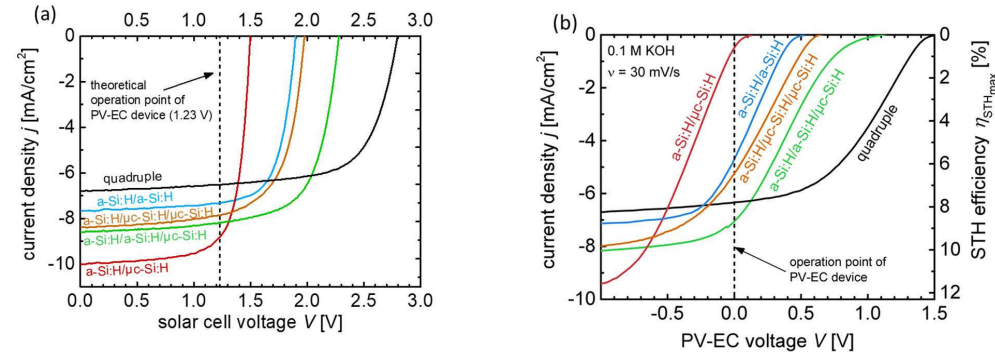
Figure 4.1: (a) Current density-voltage curves for different multi-junction cells under AM1.5G illumination. The thermodynamic water splitting potential is indicated at E_{\text{thermo}} = 1.23 V, adapted from reference [24,34,125] . (b) Current density-voltage curves for PV-EC devices employing different multi-junction cells in 0.1 M KOH under AM1.5G illumination. Platinum and ruthenium oxide were used as catalyst system. The operating voltage (0 V) for unbiased solar driven water splitting is indicated, taken from reference [24,125] .
