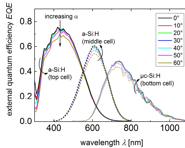
Figure A10: External quantum efficiency at various incident illumination angles plotted versus wavelength (solid lines: top cell, dashed lines: middle cell, dotted lines: bottom cell). The highest EQEs are obtained under 0^\circ incident illumination angle and decrease for an increase of the illumination angle over the entire wavelength range investigated. Comparing the individual sub cells, the most prominent reduction for the top cell is observed in the range from 350 – 500 nm and is possibly due to increased reflection at the air/glass interface. The EQE for the middle cell shows the highest reduction for wavelengths between 550 – 650 nm. The external quantum efficiency of the \mu\text{c-Si:H} bottom cell is mainly affected in the wavelength range from 700 – 850 nm. Here, the interference patterns observed in the long wavelength range (800 – 1000 nm under 0^\circ angle) shift towards shorter wavelength under increased illumination angle (750 – 1000 nm for 60^\circ ). The interference patterns are caused by the reflection of the incident light at the metal back contact of the solar cell. Due to the variation of the incident angle, the reflection at the rear side changes and causes the observed shift of the interference patterns.
