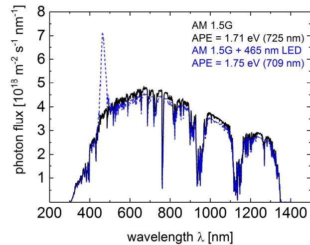
Figure 7.16: Blue modified spectrum (blue dashed curve) with an increased average photon energy of 1.75 eV compared to the AM1.5G spectrum (black solid curve) with an APE of 1.71 eV. The incident power of both spectra is 1000 \text{ W/m}^2 . Operating temperature and incident illumination angle were constant at 25^\circ \text{C} and 0^\circ respectively.
