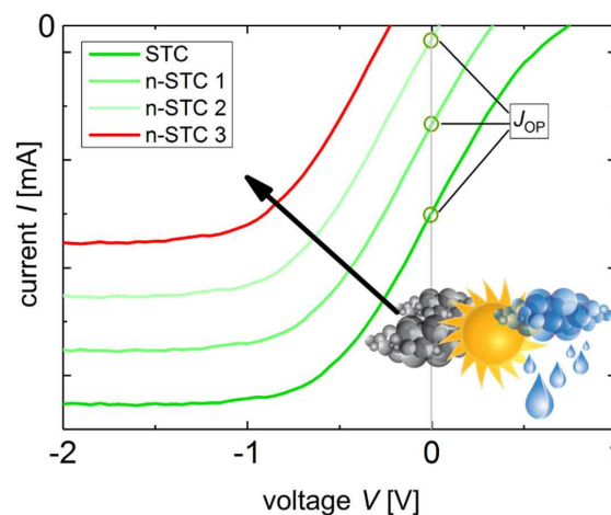
Figure 7.1: Schematic illustration of possible changes of the current-voltage characteristics for unbiased PV-EC devices caused by varying outdoor conditions. For the green IV curves, an operating current at zero bias can be extracted, thus hydrogen can be generated. In the case of the red curve, no operating current can be extracted, therefore the unbiased light induced water splitting device is switched off (no hydrogen production).
