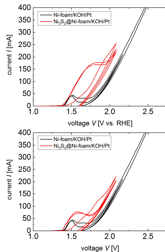
Figure A6: The electrochemical performance obtained by means of cyclic voltammetry (CV) measurements for \text{Ni}_3\text{S}_2 coated nickel foam. A hydrothermally untreated nickel foam reference is shown for comparison. The measurements were performed in 1 M potassium hydroxide solution and platinum served as counter electrode.
