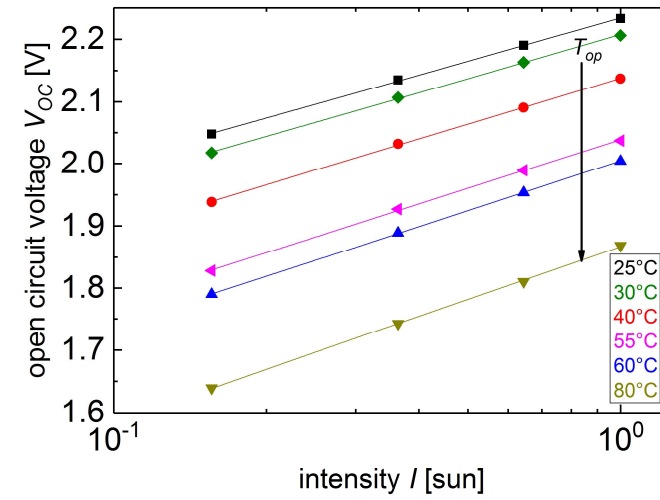
Figure A8: Open circuit voltage plotted versus the illumination intensity on logarithmic scale. The linear fits were performed using Origin and show the logarithmic dependence of the open circuit voltage.
