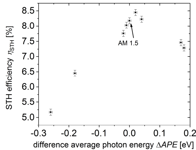
Figure 7.21: Solar-to-hydrogen efficiencies plotted versus the difference average photon energies for the PV-EC device (a-Si:H/a-Si:H/ \mu c-Si:H/Pt/KOH/IrOx), where AM1.5G is equal to zero difference in APE.
