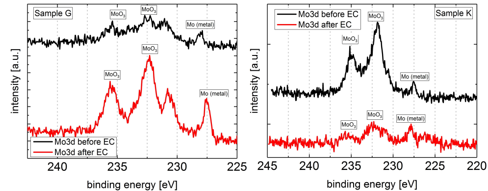
Figure 6.34: Molybdenum XP spectra of NiMo deposited at constant charge density conditions before and after the electrochemical measurement sequence (for deposition parameters see Table 6.5). Different molybdenum species are identified.
