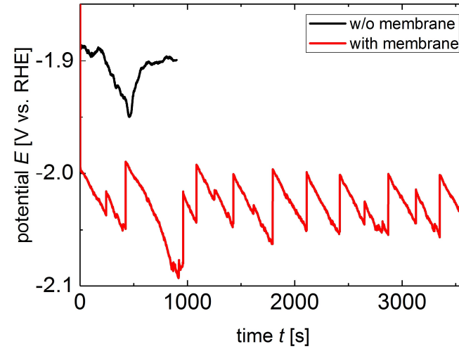
Figure 5.7: Potential over time measured for PV-EC devices employing nickel sheets as electrode in 1 M KOH solution with or without membrane. The device with membrane was monitored for 3600 s and the device without membrane was measured for 900 s. The zigzag shape of the curves is due to the detachment of gas bubbles from the electrode surface.
