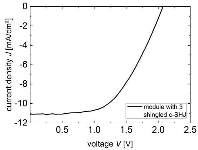
Figure 6.11: Current density-voltage curve of a module with three shingled crystalline silicon heterojunction solar cells measured under AM1.5G illumination.
