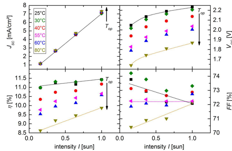
Figure 7.5: Photovoltaic parameters measured for an a-Si:H/a-Si:H/μc-Si:H triple junction cell under varied intensities and varied operating temperatures. The lines are only guides to the eye.
