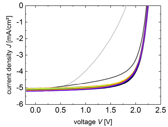
Figure A3: Current density-voltage curves of the 64 individual parts of the 64 cm² solar cell with laser processed front contact modification.
