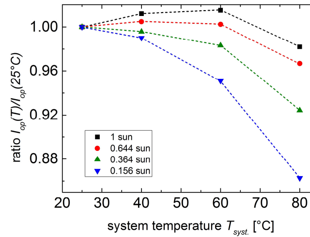
Figure 7.7: Normalized current I_{op} over system temperature T_{syst.} . For each intensity investigated, the current at the operating point of the device was normalized to the current extracted for the lowest investigated system temperature of 25 °C.
