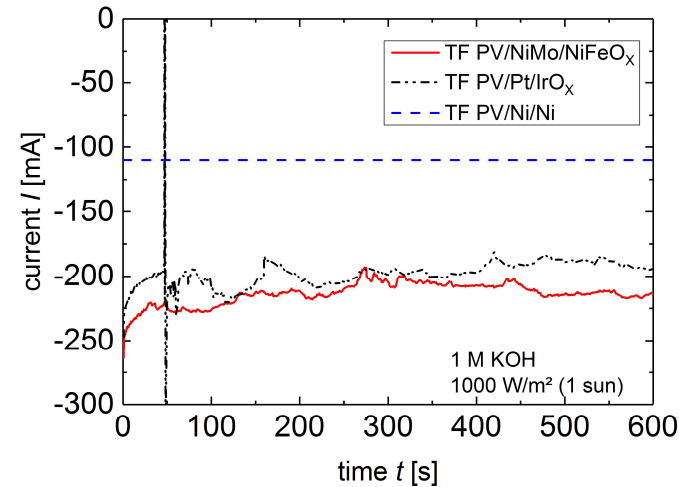
Figure 6.46: Chronoamperometric measurements of the integrated PV-EC device under bias-free conditions featuring different catalyst systems in 1 M KOH and under 1000 W/m 2 illumination. The reported current over time for the earth-abundant Ni/Ni system is shown for comparison (blue dashed line). [35]
