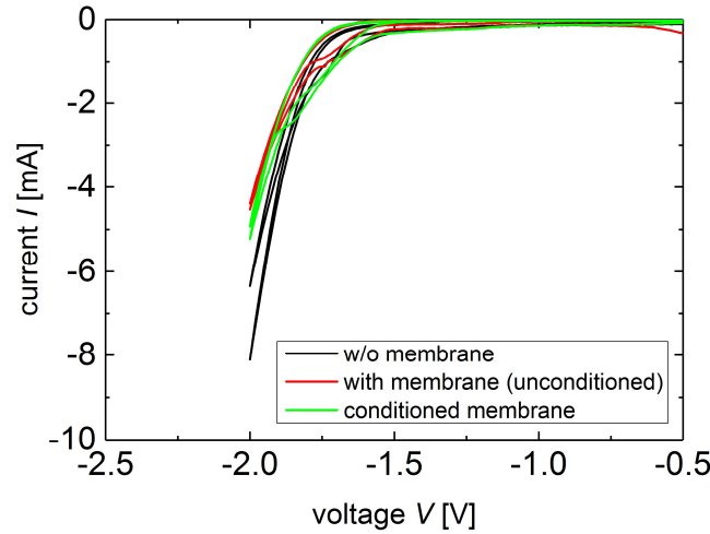
Figure 5.6: Current-voltage curves of PV-EC devices with nickel sheets on both electrode sides in 1 M KOH for the case (1) without membrane, (2) with an unconditioned membrane and (3) with a conditioned membrane (24 h in 0.5 M NaCl solution at 25 °C).
