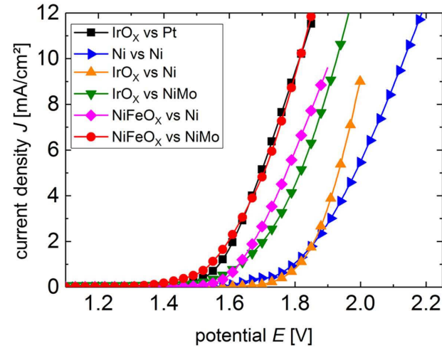
Figure 6.39: Current density-potential curves measured for various catalyst systems in alkaline media for an electrode size of 50.3 cm 2 .
