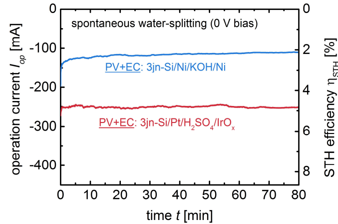
Figure 6.5: Chronoamperometric measurements of the upscaled PV-EC device under bias-free conditions employing (red curve) platinum and iridium oxide on titanium sheet substrates in acidic media (1 M H 2 SO 4 ) and (blue curve) nickel electrodes in alkaline media (1 M KOH).
