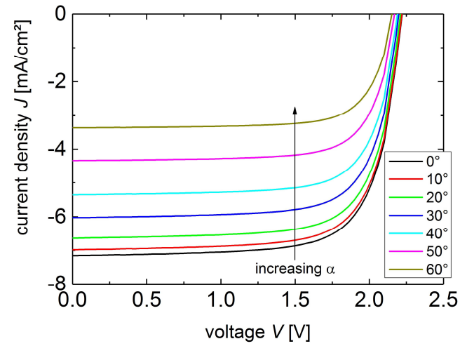
Figure A9: Current density-voltage curves measured under varied incident illumination angles for an a-Si:H/a-Si:H/ \mu c-Si:H triple junction solar cell.
