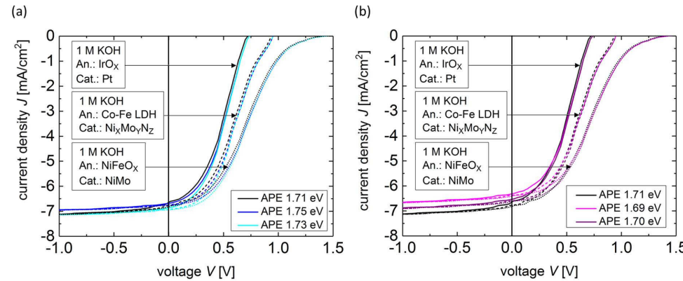
Figure 7.18: Calculated current density-voltage curves of an a-Si:H/a-Si:H/μc-Si:H triple junction solar cell based PV-EC device employing different catalyst systems (A, solid lines) Pt/IrO x , (B, dashed lines) NiMo/Nz/Co-Fe LDH and (C, dotted lines) NiMo/NiFeO x under standard test conditions (STC, AM1.5G, APE = 1.71 eV, black line) and under modified spectra: (a) high APEs (blue rich) and (b) low APEs (red rich). 1 M potassium hydroxide was used as electrolyte in all cases. The operating voltage for unbiased light induced water splitting is indicated at zero volts.
