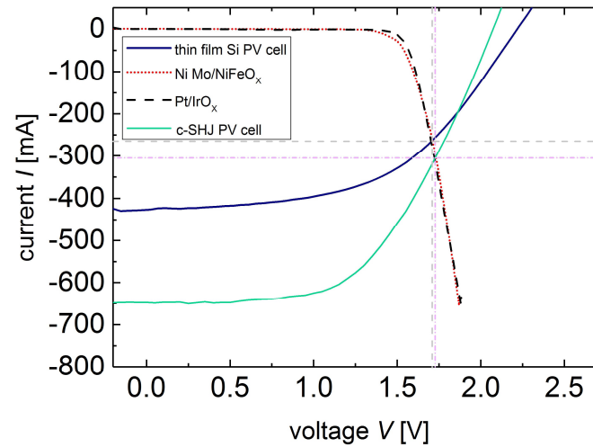
Figure 6.42: Current-voltage curves of (i) a triple junction a-Si:H/a-Si:H/ \mu c-Si:H solar cell (TF-Si, blue solid line) with an active area A_{\text{PV}} = 64 \text{ cm}^2 under AM1.5G illumination, (ii) current-voltage curve of a module with three shingled silicon heterojunction solar cells (c-Si, green solid line) with an active area A_{\text{PV}} = 58.5 \text{ cm}^2 under AM1.5G illumination and (iii) current-voltage curves of the electrochemical (EC) cells with two catalyst pair systems NiMo/NiFeO x (red dotted line) and Pt/IrO x (black dashed line) on 50.3 cm 2 area in 1 M KOH. The intersection point delivers the currents (265 mA, 304 mA) and voltages (1.7 V, 1.73 V) at the theoretical operating points of the PV-EC devices. Using equation (40), the theoretically expected solar-to-hydrogen efficiencies can be calculated for both systems ( \eta_{\text{STH}} = 5.1\% for TF-Si and \eta_{\text{STH}} = 6.4\% for c-Si).
