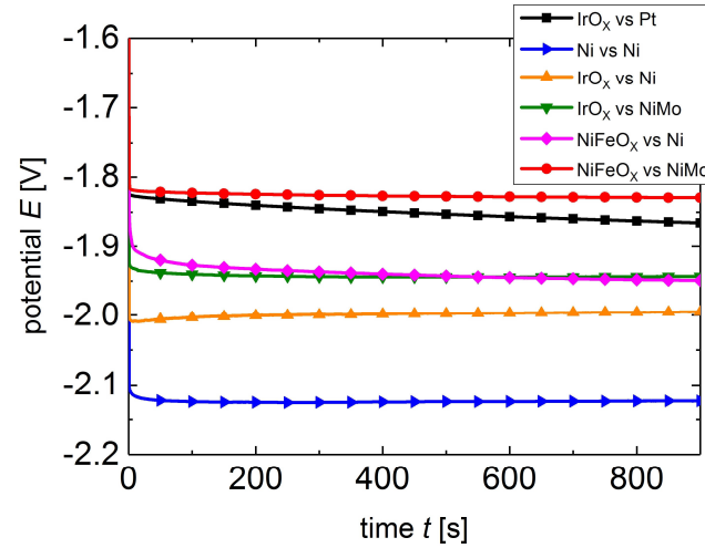
Figure 6.41: Potential measured over time (900 s) for an electrolysis at -10 mA/cm 2 in alkaline media for various catalyst systems covering an electrode size of 50.3 cm 2 .
