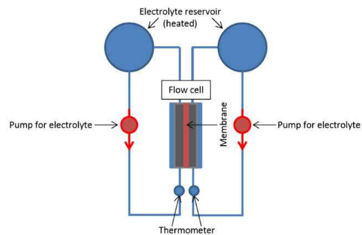
Figure A5: Schematics (not to scale) of a setup (as used by Evonik Creavis GmbH) to measure the temperature dependence of a flow (PV)-EC cell, including a membrane for gas separation, heated electrolyte reservoirs, and temperature control in the electrolyte flow circuit controlled by a peristaltic pump. The flow EC cell in zero gap configuration consisting of porous electrodes (grey) and a membrane (100 \mu m, red). In order to form a PV-EC device, a PV cell can be electrically attached to the cathode side of the EC cell.
