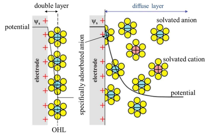
Figure 2.12: Helmholtz model of the metal/electrolyte interface. The Helmholtz layer consists of the inner and outer Helmholtz layer (specifically adsorbed anion (IHL) and OHL) and the diffusion layer. The potential drop across the different layers is indicated, adapted from reference [122] .
