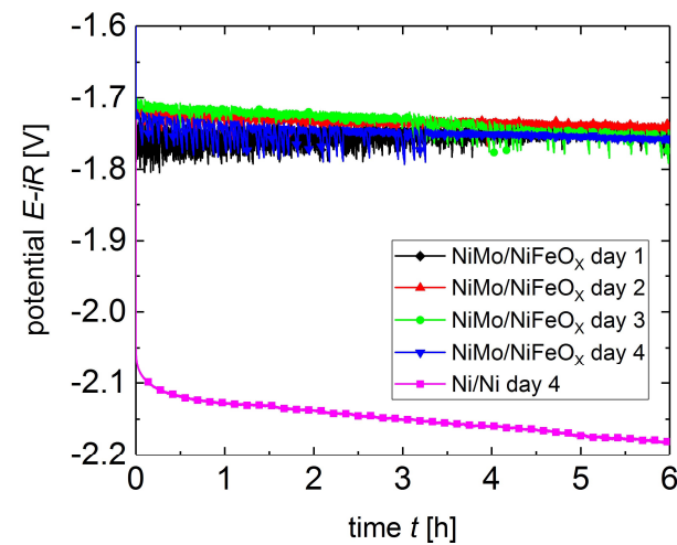
Figure 6.49: Potential over time measured for 6 h for four days at -10 mA/cm 2 electrolysis for the catalyst system consisting of NiMo/NiFeO x coated nickel sheet electrodes.
