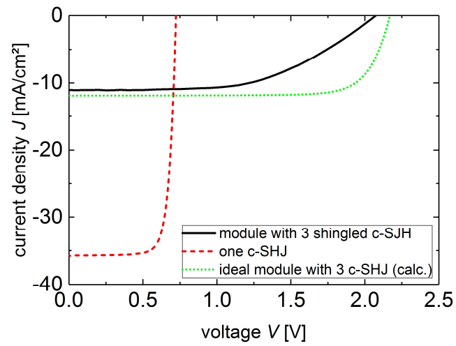
Figure 6.12: Current density-voltage curves of a single crystalline silicon heterojunction (c-SHJ) solar cell (red dashed curve), of the measured module with three shingled crystalline silicon heterojunction (c-SHJ) solar cells (black solid curve) and the ideal module with three crystalline silicon heterojunction (c-SHJ) cells without series resistance losses due to the connection (green dotted curve).
