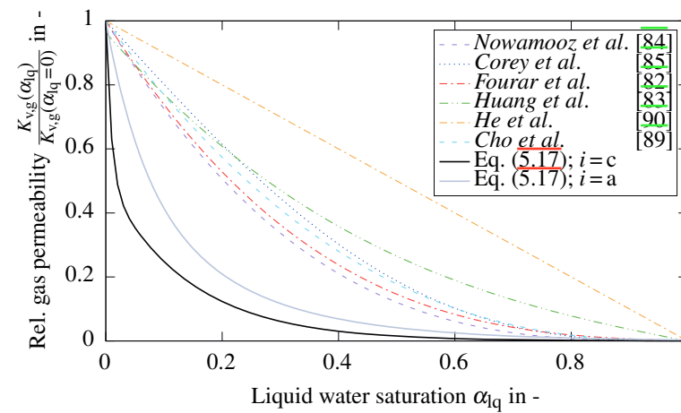
Figure 5.17: Comparison of developed permeability correlations with literature approaches initially summarized by Cho et al. [89].
