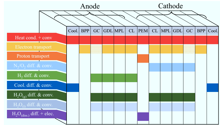
Figure 4.1: Overview of conservation equations in PEMFC model.
