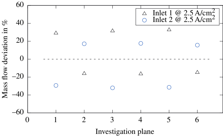
Figure A.3: Exchange mass flow rate from 4-repetition unit simulation of cathode gas channels at 2.5 A/cm 2 .
