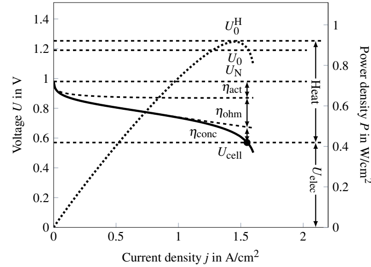
Figure 3.2: General polarization (solid) and power density curve (dotted) of a single PEMFC.
