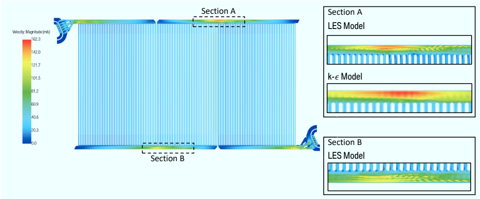
Figure A.15: Velocity profile of anode flow field cut section plane with indication of turbulence, using an LES and k-ε approach with inlet hydrogen mass flows, corresponding to \lambda_A = 4 at j_{avg} = 2.5 \text{ A/cm}^2 .
