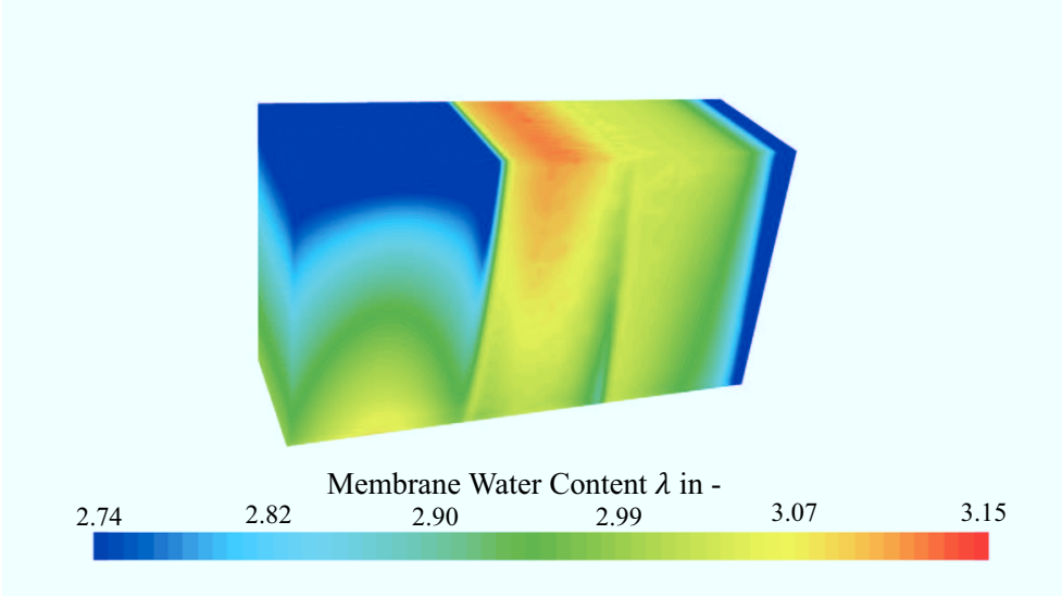
Figure A.26: Membrane water content distribution on anode CL-MEM interface of 60-cell stack for ID3 case, corresponding to a voltage of 49.1 V.
