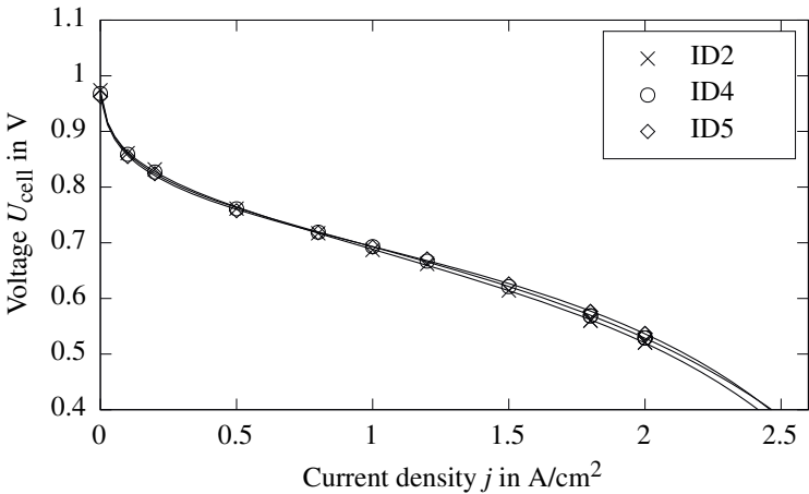
Figure A.21: Experimental polarization curves for temperature variation at ID2, ID4 and ID5.
