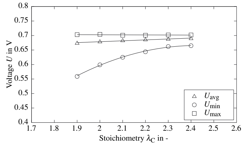
Figure A.35: Minimal, maximal and average cell voltages of 60-cell stack for cathode stoichiometry variation.
