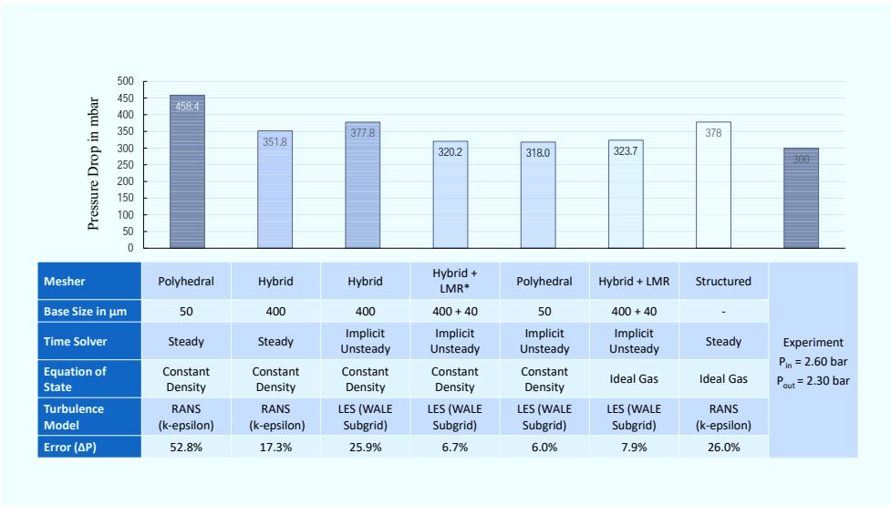
Figure A.16: Mesh independence study for anode flow field single phase pressure drop.
