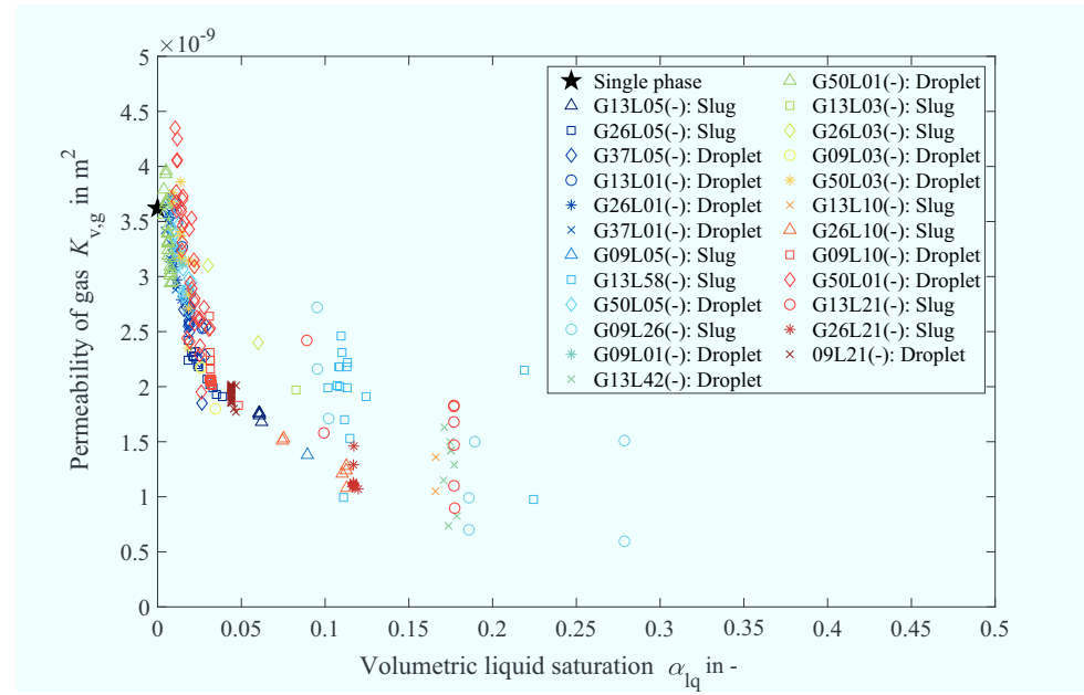
Figure A.11: Raw data of anode gas channel permeabilities from selected cases.
