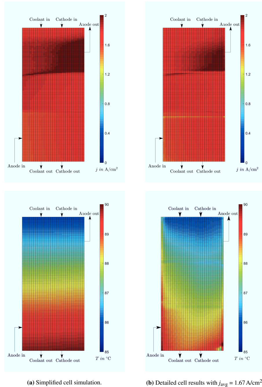
Figure A.22: Current density (top) and temperature (bottom) distribution of simplified (left) and detailed cell simulation (right) results of ID3 at 0.614 V.
