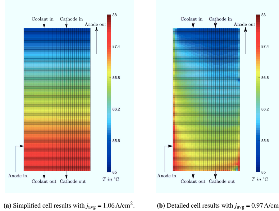
Figure 7.10: Temperature distribution of simplified (left) and detailed (right) cell simulation at 0.686V.
