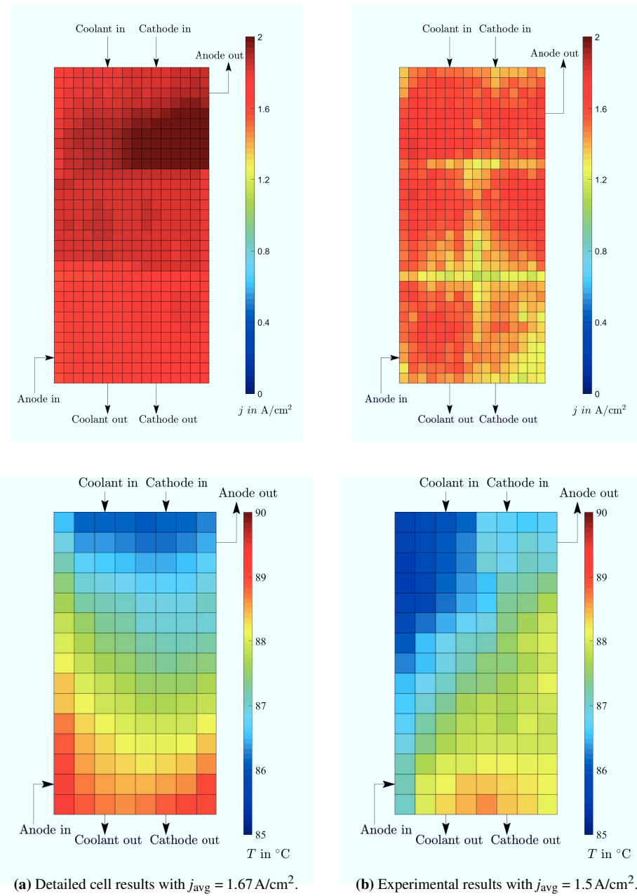
Figure A.17: Current density (top) and temperature (bottom) distribution of detailed cell simulation (left) and experimental cell (right) results of ID3 at 0.614 V.
