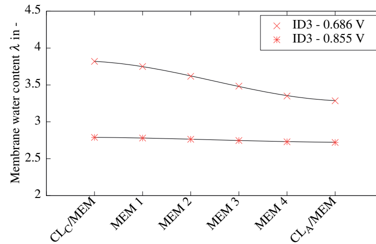
Figure 6.6: Through-plane membrane water content comparison of two ID3 cases at 0.686 and 0.855 V.
