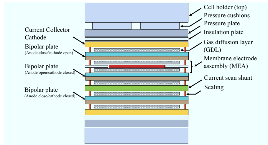
Figure 6.8: Experimental setup for local current (544 segments) and temperature (144 segments) measurement in a single automotive PEM fuel cell according to Herden et. al [96].
