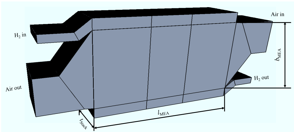
Figure 8.1: Detailed single cell geometry for PEMFC simulations.
