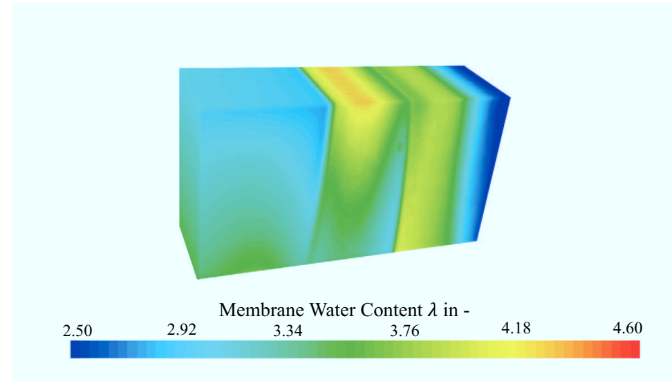
Figure 8.5: Membrane water content distribution on anode CL-MEM interface of 60-cell stack for ID3 case, corresponding to a voltage of 41.2 V.
