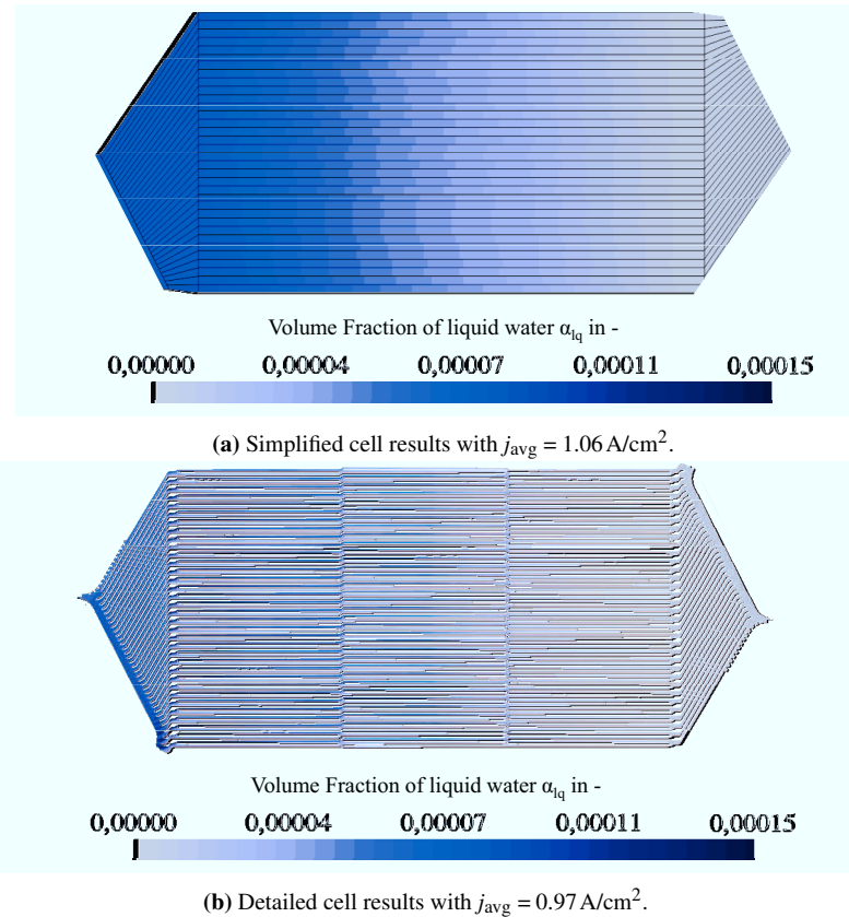
Figure 7.13: Liquid water volume fraction distribution in cathode gas channels of simplified (top) and detailed (bottom) cell simulation for ID3 at 0.686V.
