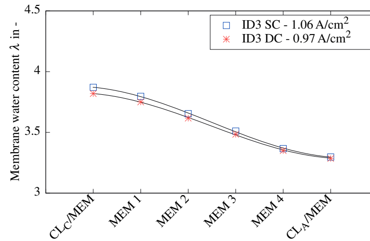
Figure 7.12: Through-plane membrane water content \lambda comparison of simplified (blue square) and detailed (red star) case for ID3 at 0.686 V.
