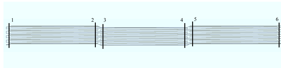
Figure A.1: 4-repetition unit geometry of cathode gas channels with investigation planes 1 - 6.
