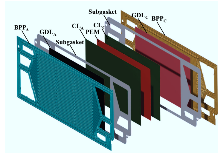
Figure 3.3: PEM fuel cell functional layers
