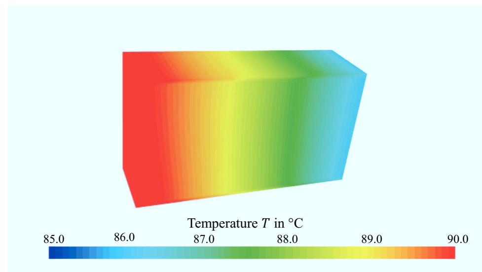
Figure A.28: Temperature distribution in coolant regions of 60-cell stack for ID3, corresponding to a voltage of 36.8 V.
