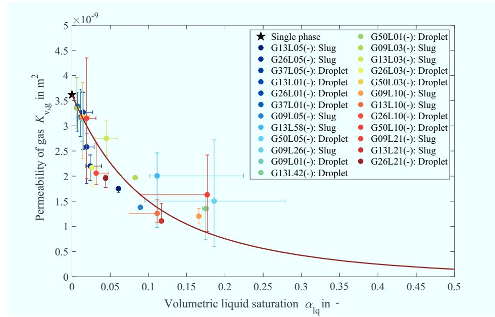
Figure 5.15: Anode gas channel permeability correlation constructed from selected cases with indication of variation bars for the respective case.
