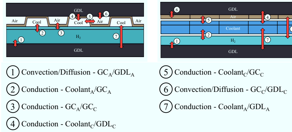
Figure 7.4: Heat exchange in detailed (left) and simplified (right) cell with indication of transfer phenomena.
