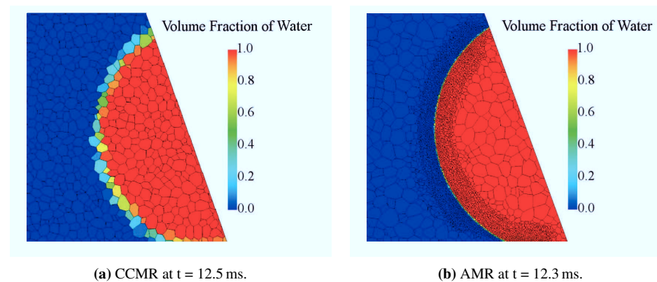
Figure 5.8: Cross-section plot of volume fraction of CCMR at 12.5 ms (left) and AMR at 12.3 ms (right) simulation results.
