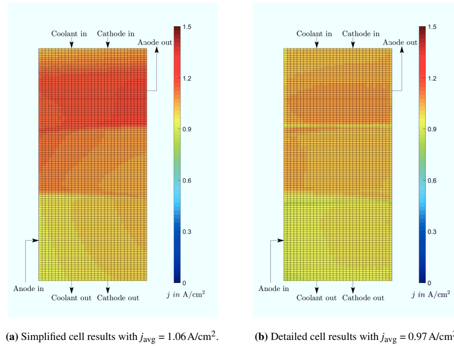
Figure 7.9: Current density distribution of simplified (left) and detailed (right) cell simulation at 0.686V.
