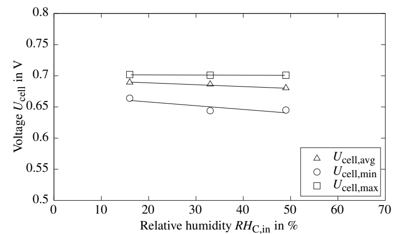
Figure A.32: Minimal, maximal and average cell voltages of 60-cell stack for cathode inlet RH variation.
