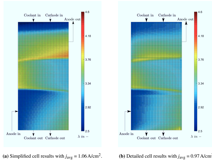
Figure 7.11: Membrane water content distribution of simplified (left) and detailed (right) cell simulation on anode CL-MEM interface for ID3 at 0.686V.
