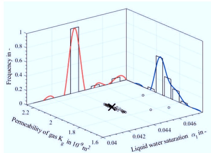
Figure 5.14: Exemplary application of k-means clustering algorithm on case G26L21.
