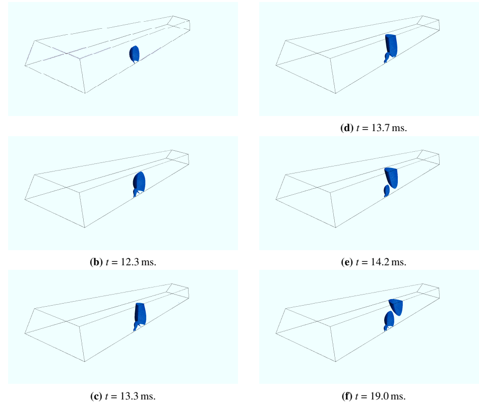
Figure 5.5: Water volume iso-surface plots at physical times of 5.0, 12.3, 13.3, 13.7, 14.2 and 19 ms. Air flows from left to right.
