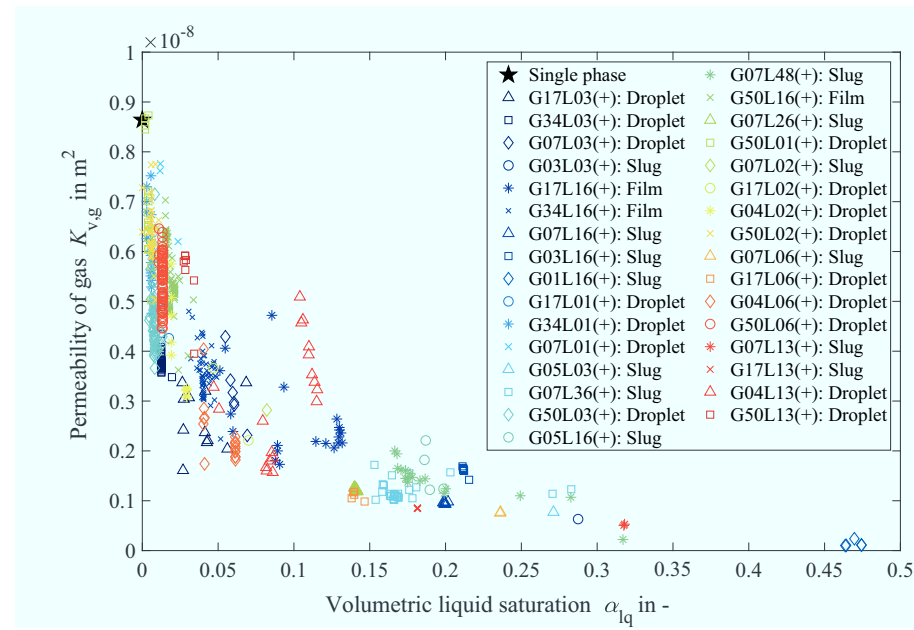
Figure A.12: Raw data of cathode gas channel permeabilities from selected cases.
