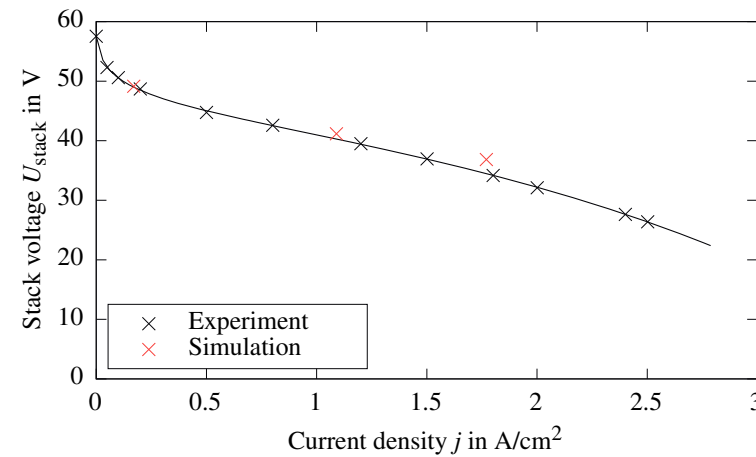
Figure 8.8: Experimental polarization curve of 60-cell stack with inclusion of simulative results.
