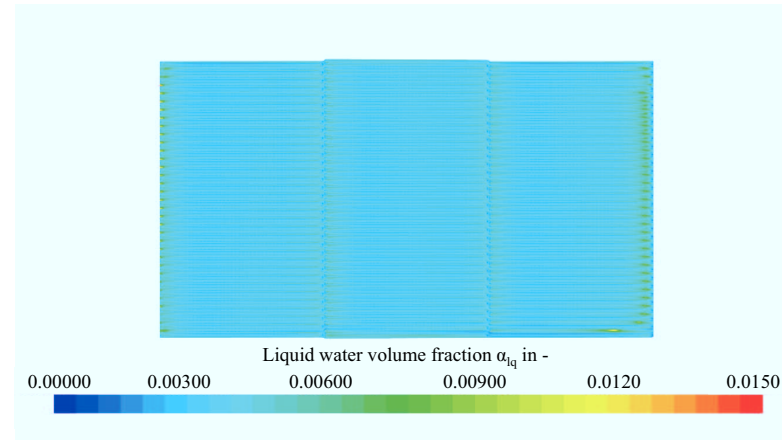
Figure 6.4: Liquid water volume fraction plot on anode CL-MEM interface for ID3 case at 0.686 V.
