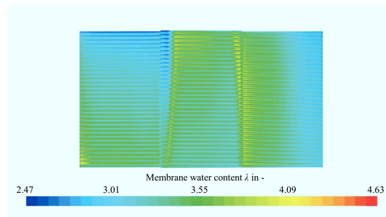
Figure 6.5: Membrane water content plot on anode CL-MEM interface for ID3 case at 0.686 V.
