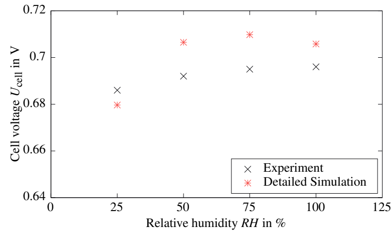
Figure 6.12: Comparison of relative humidity variation between experimental and simulative cases of ID3, ID5, ID6 and ID7 at j_{exp} = 1.0 A/cm 2 .
