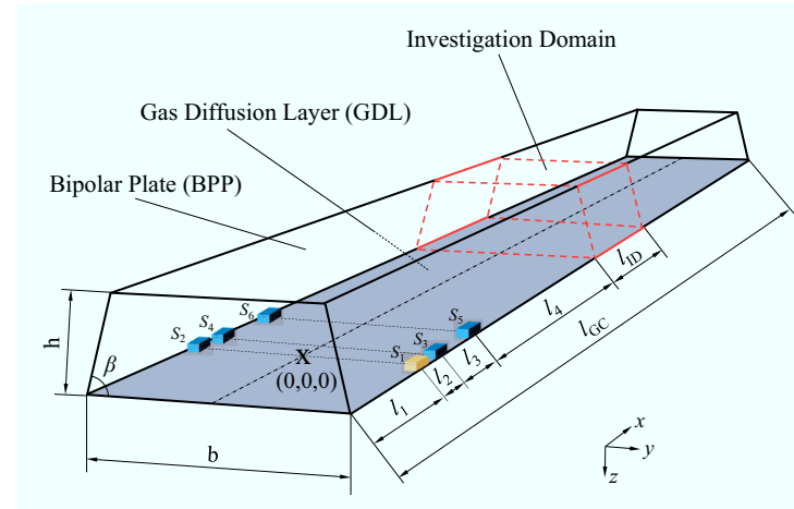
Figure 5.1: Single channel geometry for VOF simulations in cathode and anode GCs with indication of source term positions and investigation domain.
