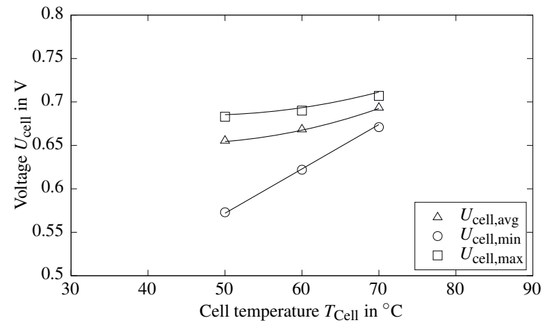
Figure A.34: Minimal, maximal and average cell voltages of 60-cell stack for cell temperature variation.
