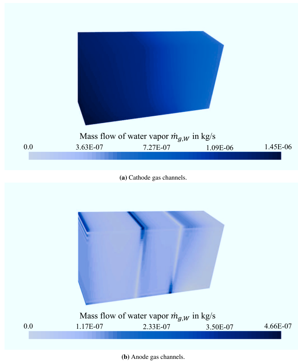
Figure A.31: Mass flow distribution of water vapor in cathode and anode gas channels of 60-cell stack for ID3 case, corresponding to a voltage of 36.8 V.
