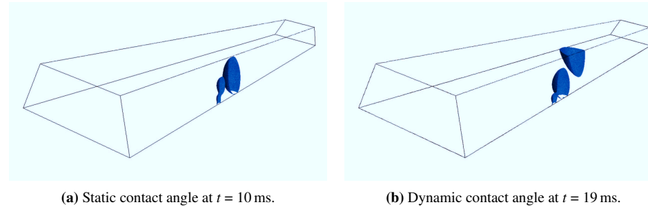
Figure 5.4: Water volume fraction iso-surface plots of static (left) and dynamic (right) contact angle case.
