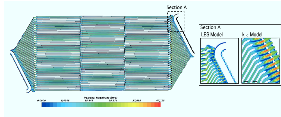
Figure A.14: Velocity profile of cathode flow field cut section plane with indication of turbulence, using an LES and k-\epsilon approach with inlet air mass flows, corresponding to \lambda_C = 4 at j_{\text{avg}} = 2.5\text{ A/cm}^2 .
