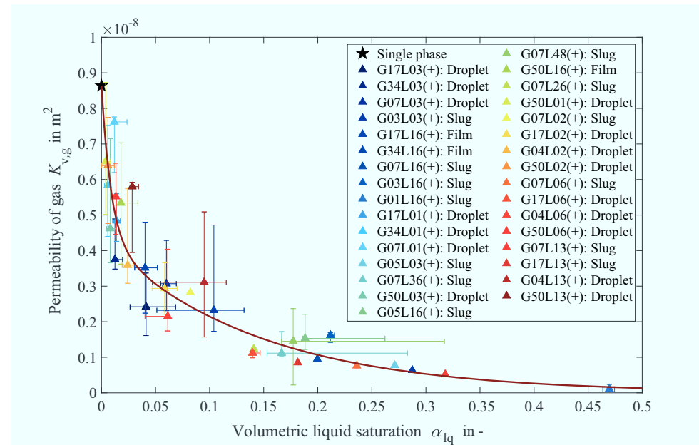
Figure 5.16: Cathode gas channel permeability correlation constructed from selected cases with indication of variation bars for the respective case.
