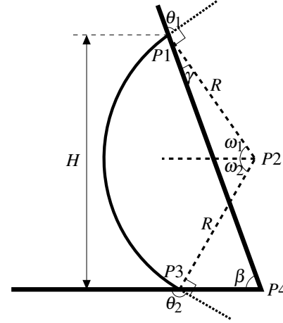
Figure A.4: 2D-Sketch of a spherical droplet inside a channel corner, for the derivation of an analytical solution.
