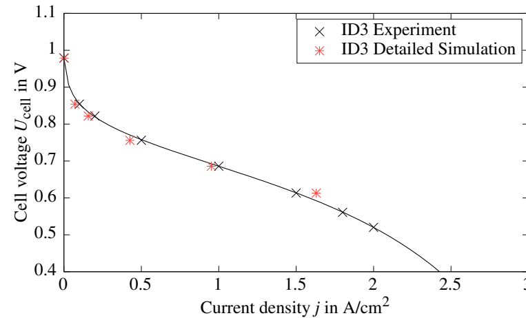
Figure 6.9: Experimental polarization curve with simulative data points at ID3.
