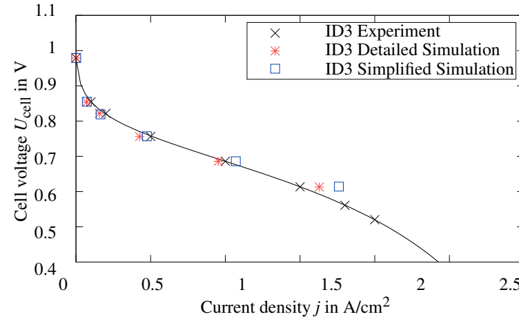
Figure 7.8: Polarization curves for simulation and experimental validation at ID3
