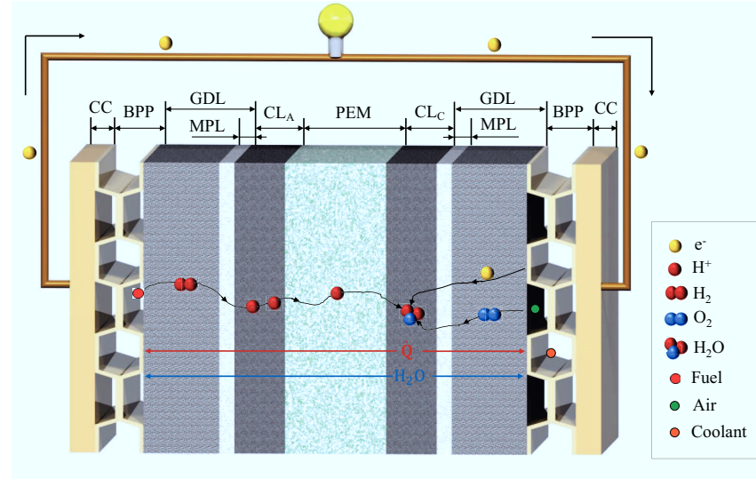
Figure 3.1: Schematic cut-plane through a low temperature PEMFC single cell
