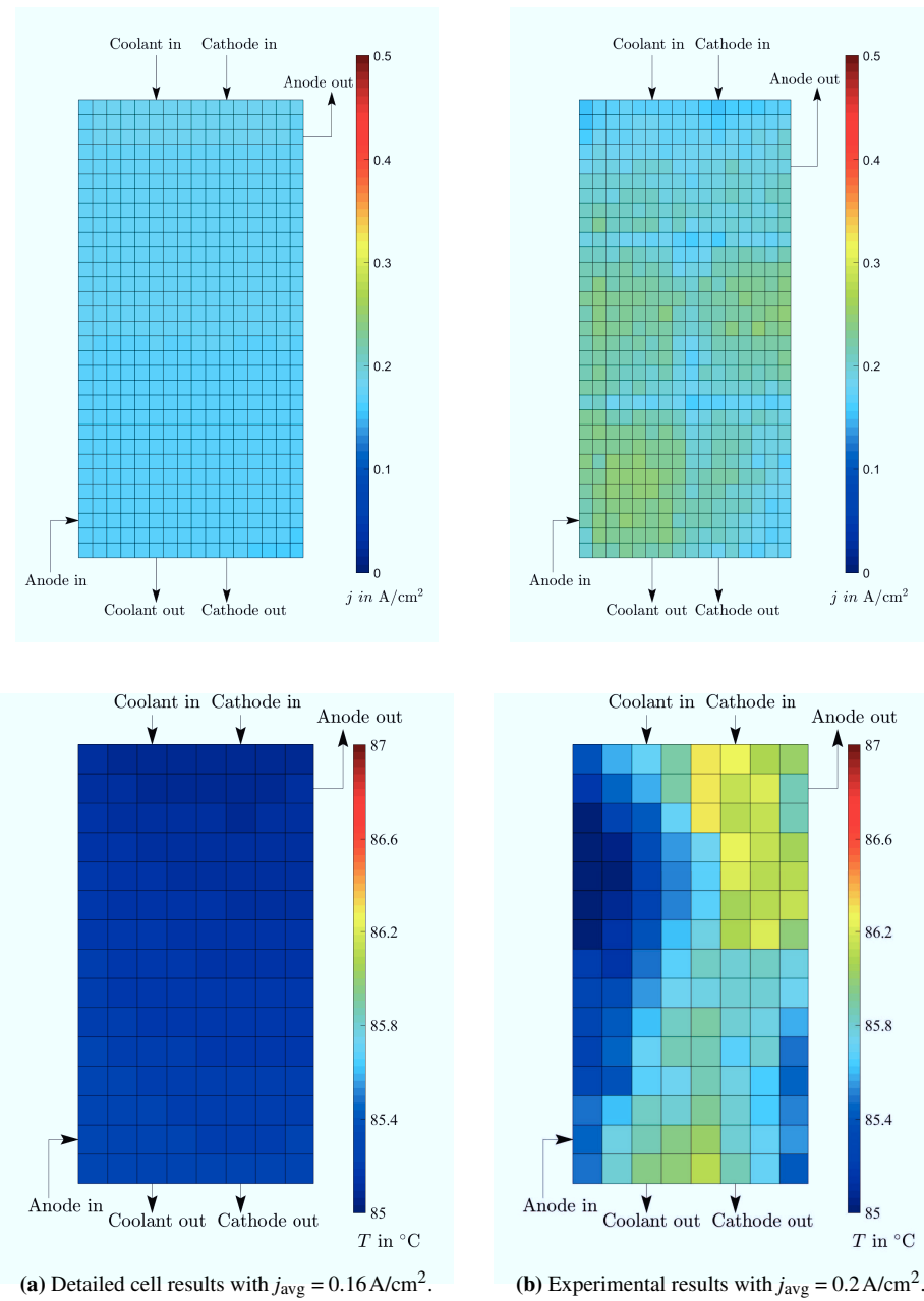
Figure A.18: Current density (top) and temperature (bottom) distribution of detailed cell simulation (left) and experimental cell (right) results of ID3 at 0.819 V.
