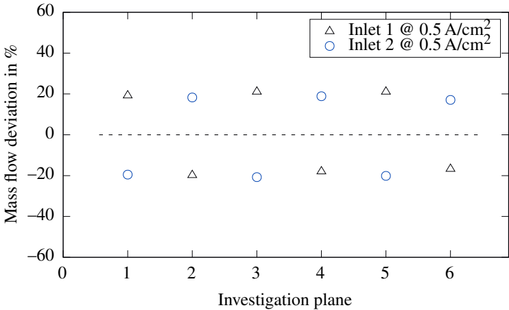
Figure A.2: Exchange mass flow rate from 4-repetition unit simulation of cathode gas channels at 0.5 A/cm 2 .
