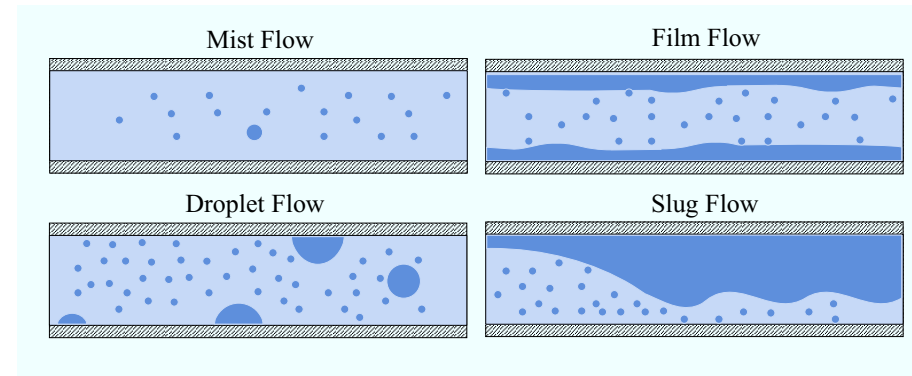
Figure 3.5: Two phase flow regimes inside PEMFC gas channels.
