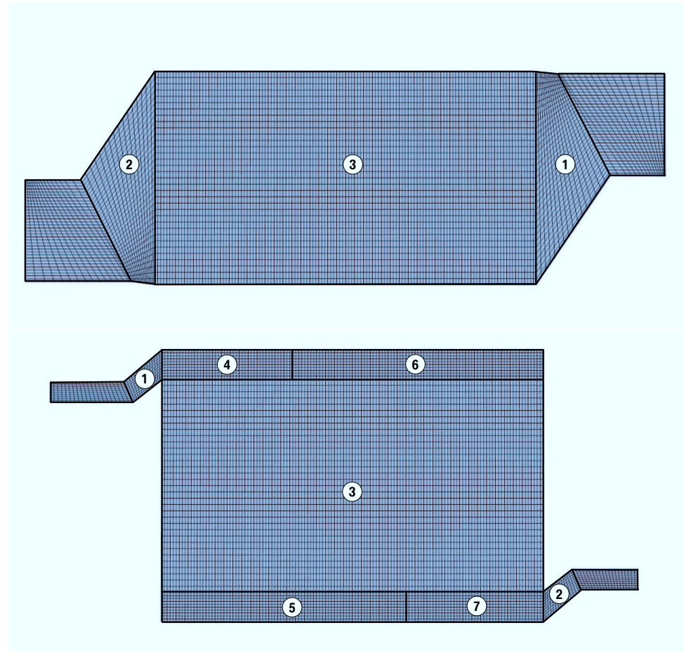
Figure 7.3: Simplified model of cathode (top) and anode (bottom) side gas channel geometries.
