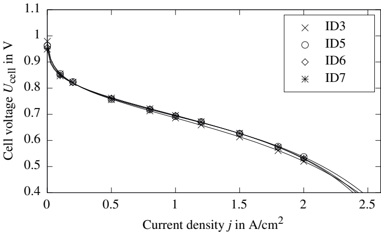
Figure A.20: Experimental polarization curves for relative humidity variation at ID3, ID5, ID6 and ID7.
