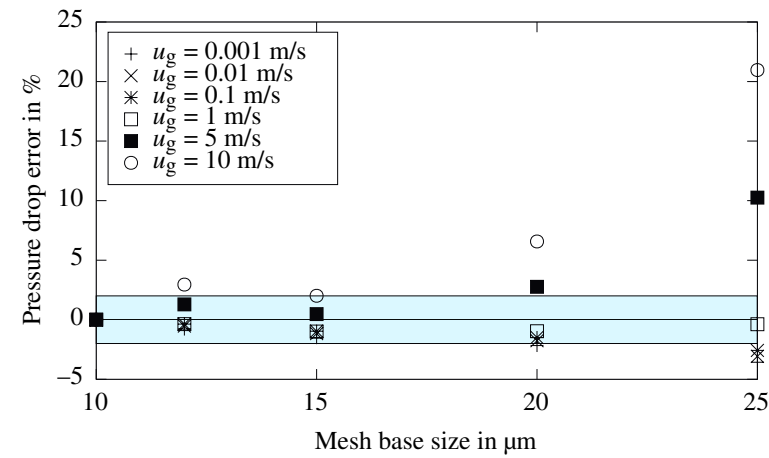
Figure A.5: Mesh independence study for single-phase flow inside anode gas channel.
