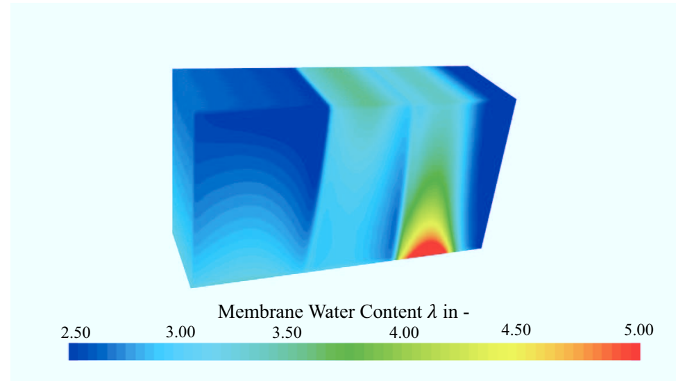
Figure A.30: Membrane water content distribution on anode CL-MEM interface of 60-cell stack for ID3 case, corresponding to a voltage of 36.8 V.
