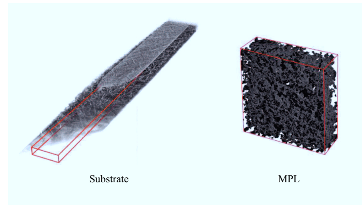
Figure A.13: Representative Volumes (RV) of substrate and MPL, produced via \mu -CT and FIB/SEM-tomographie scan reconstructions.
