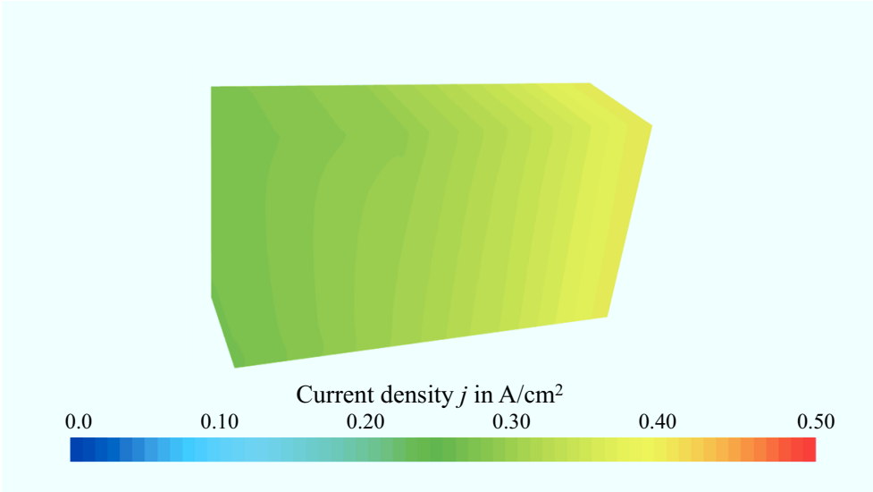
Figure A.25: Current density distribution on anode and cathode reaction planes of 60-cell stack for ID3, corresponding to a voltage of 49.1 V.
