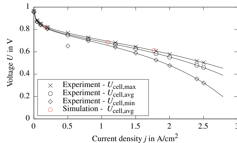
Figure 8.9: Experimental polarization curve of single cells in 60-cell stack with U_{\text{max}} , U_{\text{avg}} and U_{\text{min}} .
