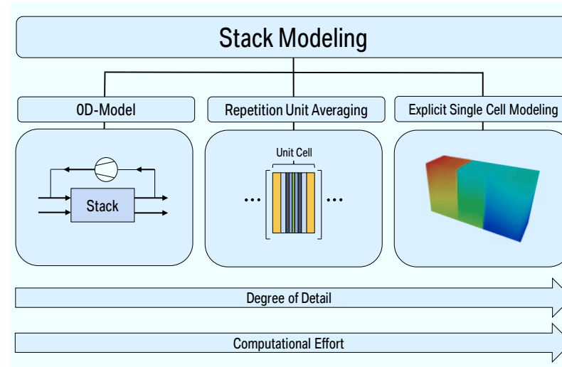
Figure 3.6: Overview of different stack modeling approaches.
