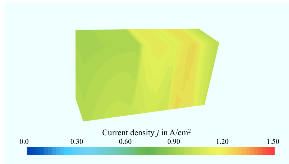
Figure 8.4: Current density distribution on reaction planes of 60-cell stack for ID3 case, corresponding to a voltage of 41.2 V.
