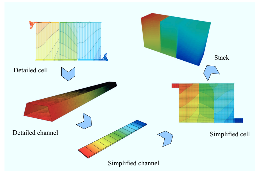
Figure 7.1: Stack model creation procedure.
