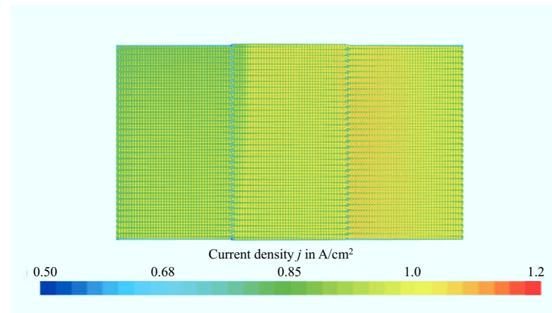
Figure 6.7: Current density plot on anode CL-MEM interface for ID3 case at 0.686 V.
