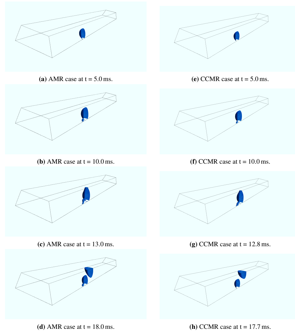
Figure 5.7: Water volume iso-surface plots of AMR and CCMR results at physical times of 5.0, 10.0, 12.8, 13.0, 17.7 and 18.0 ms. Air flows from left to right.
