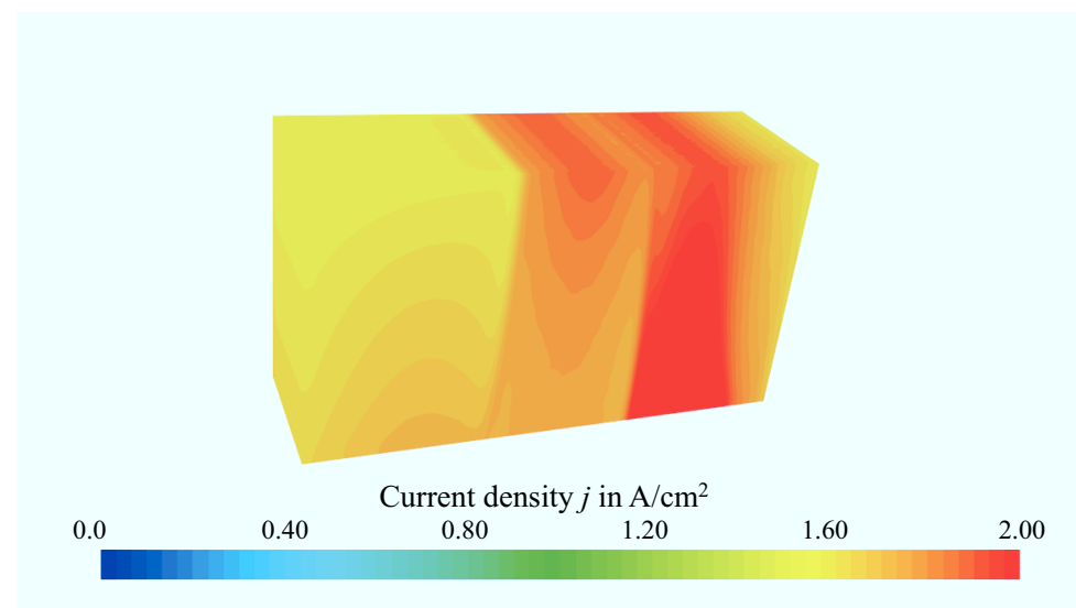
Figure A.29: Current density distribution on anode and cathode reaction planes of 60-cell stack for ID3, corresponding to a voltage of 36.8 V.
