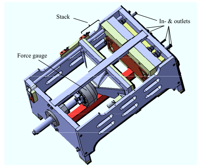
Figure 8.7: Experimental setup for 60-cell measurements.
