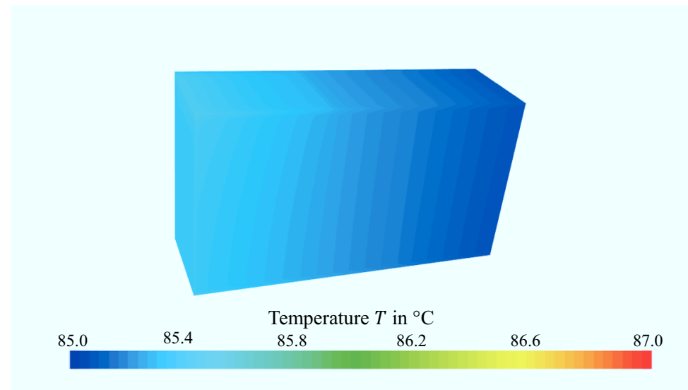
Figure A.24: Temperature distribution in coolant regions of 60-cell stack for ID3, corresponding to a voltage of 49.1 V.
