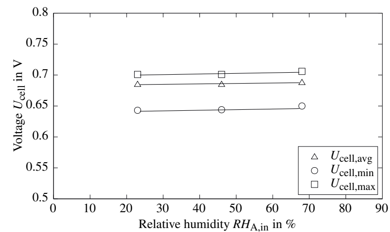
Figure A.33: Minimal, maximal and average cell voltages of 60-cell stack for anode inlet RH variation.
