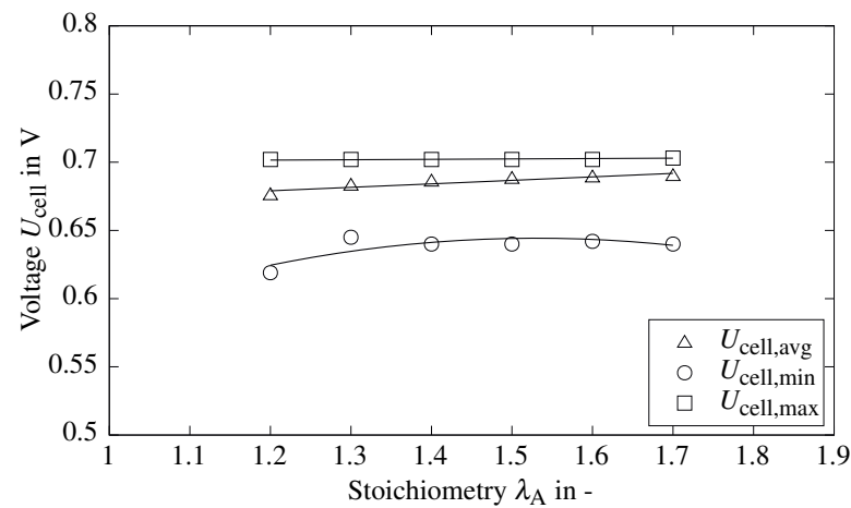
Figure A.36: Minimal, maximal and average cell voltages of 60-cell stack for anode stoichiometry variation.
