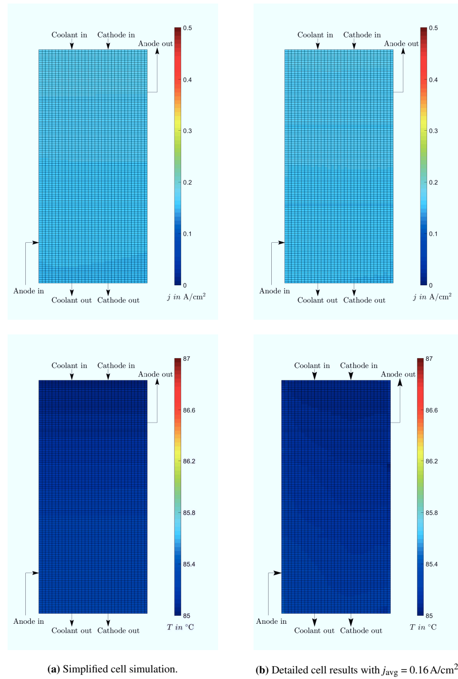
Figure A.23: Current density (top) and temperature (bottom) distribution of simplified (left) and detailed cell simulation (right) results of ID3 at 0.819 V.
