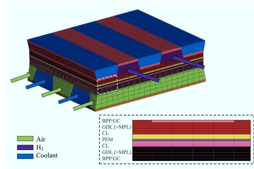
Figure 6.2: Mesh fragment of detailed single cell active area model with indications of fluid inlets.
