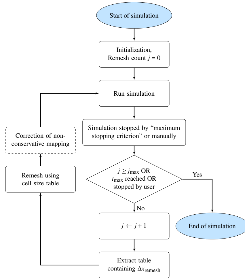
Figure 5.2: Methodology of adaptive mesh refinement. [71]
