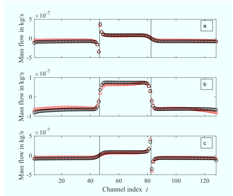
Figure 7.7: Mass flow comparison between detailed (red triangle) and simplified model (black circle) for anode flow field, evaluated on plane cut a (top), b (middle) and c (bottom).
