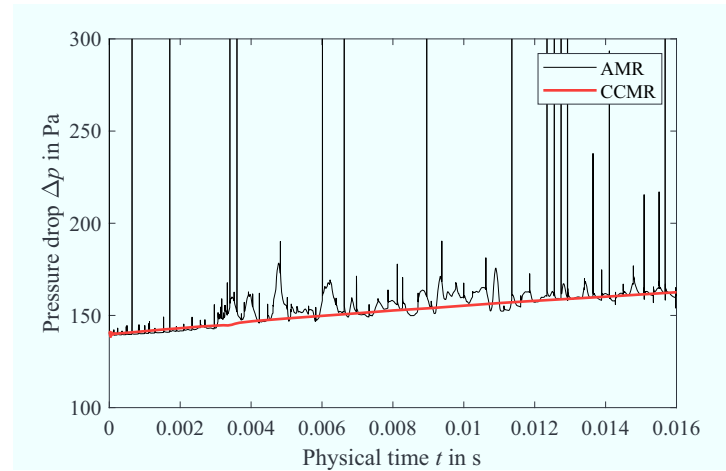
Figure 5.10: Comparison of pressure drop time-series in anode single channel simulation of AMR and CCMR simulation.
