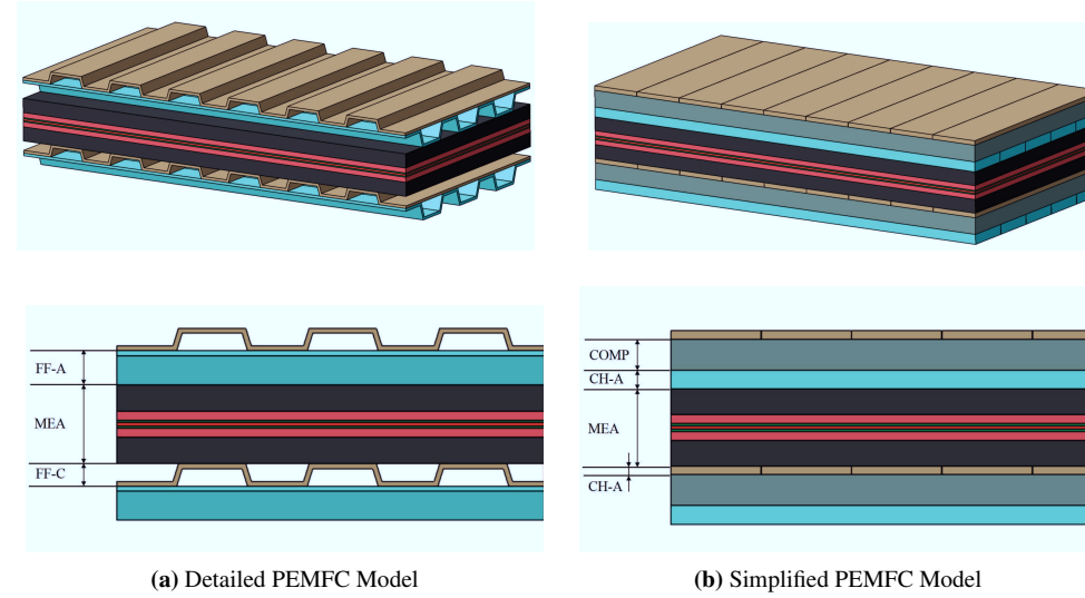
Figure 7.2: Schematic sections of detailed (a) and simplified (b) cell geometry.
