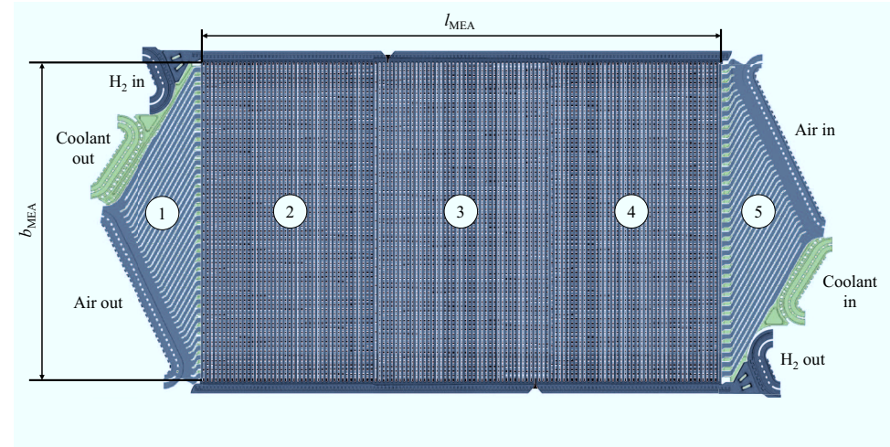
Figure 6.1: Detailed single cell geometry for PEMFC simulations.
