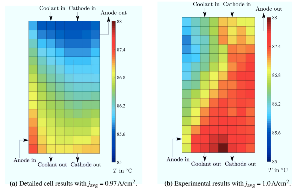
Figure 6.11: Temperature distribution of detailed cell simulation (left) and experimental cell (right) results at 0.686V A/cm 2 .
