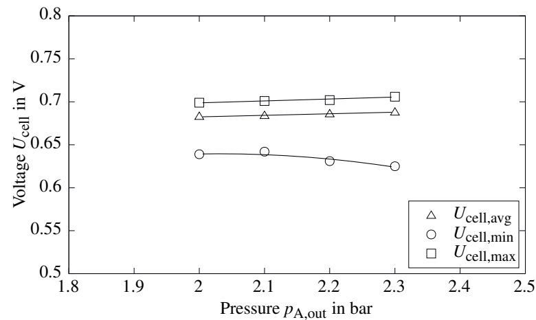
Figure A.37: Minimal, maximal and average cell voltages of 60-cell stack for cathode outlet pressure variation.
