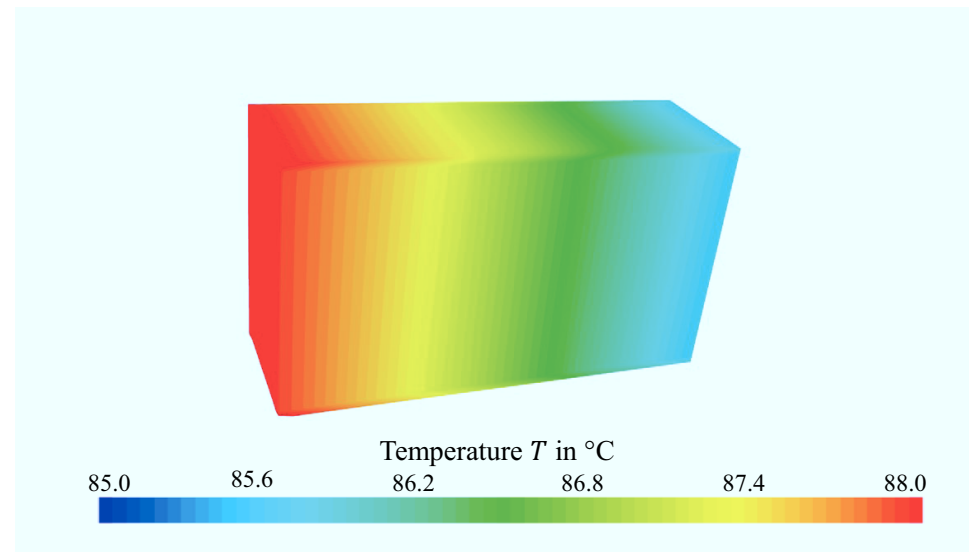
Figure 8.3: Temperature distribution in anode and cathode coolant regions of 60-cell stack for ID3 case, corresponding to a voltage of 41.1 V.
