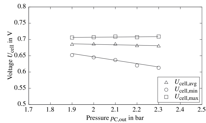
Figure A.38: Minimal, maximal and average cell voltages of 60-cell stack for anode outlet pressure variation.
