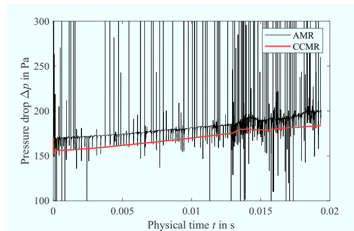
Figure 5.9: Comparison of pressure drop time-series in cathode single channel simulation of AMR and CCMR simulation.
