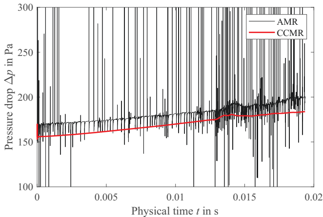
Figure 5.9: Comparison of pressure drop time-series in cathode single channel simulation of AMR and CCMR simulation.
