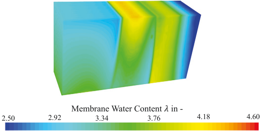
Figure 8.5: Membrane water content distribution on anode CL-MEM interface of 60-cell stack for ID3 case, corresponding to a voltage of 41.2 V.
