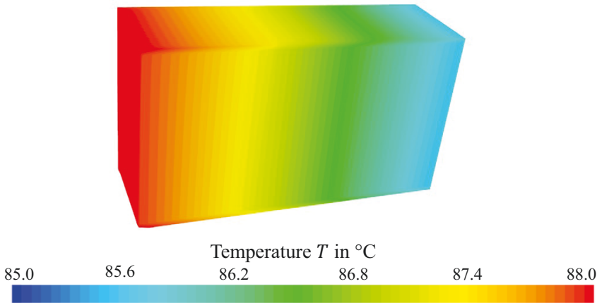
Figure 8.3: Temperature distribution in anode and cathode coolant regions of 60-cell stack for ID3 case, corresponding to a voltage of 41.1 V.
