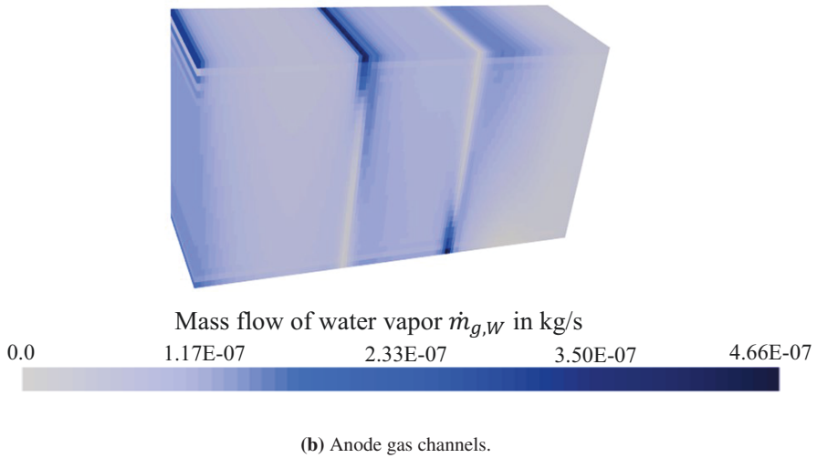
Figure A.31: Mass flow distribution of water vapor in cathode and anode gas channels of 60-cell stack for ID3 case, corresponding to a voltage of 36.8 V.
