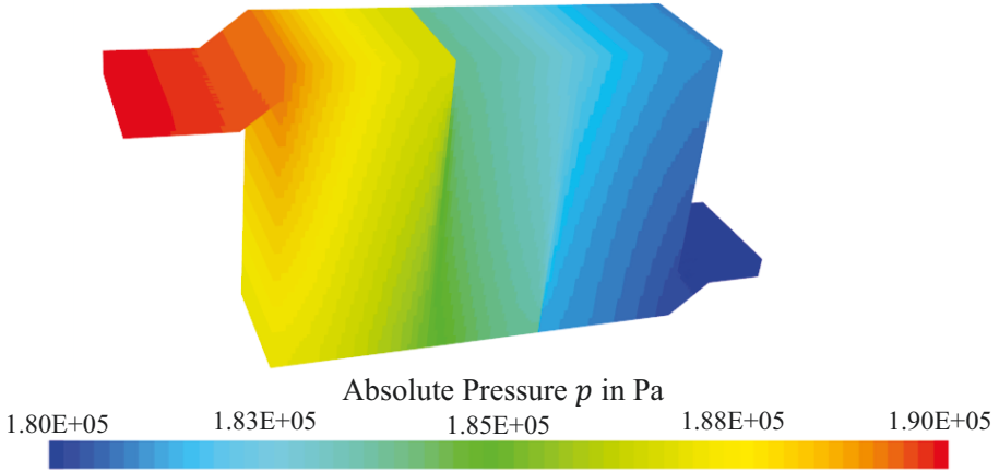
(b) Anode pressure distribution.
