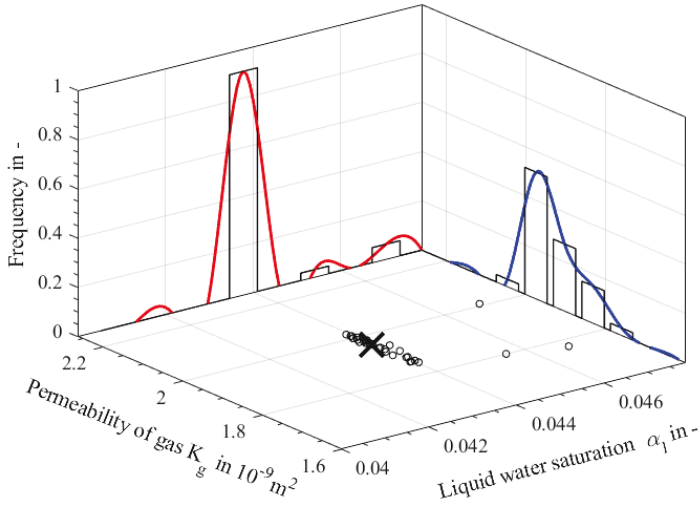
Figure 5.14: Exemplary application of k-means clustering algorithm on case G26L21.
