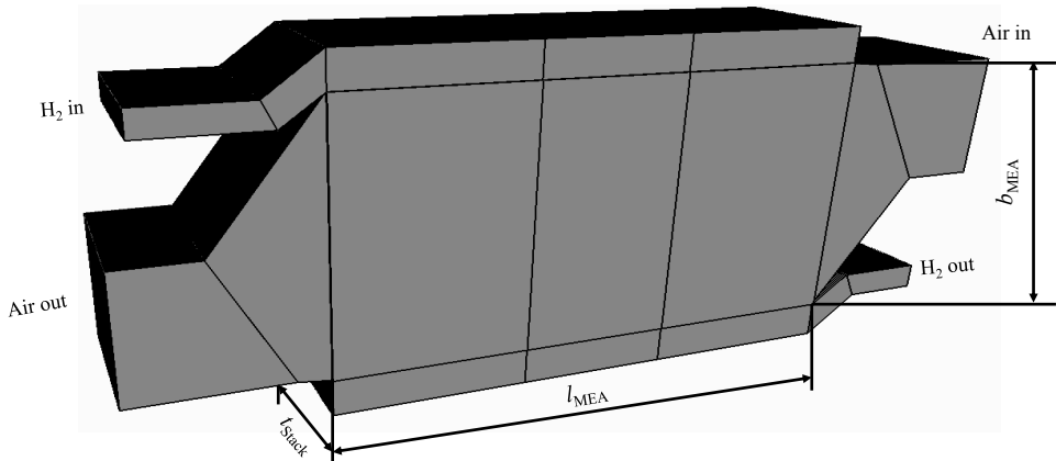
Figure 8.1: Detailed single cell geometry for PEMFC simulations.
