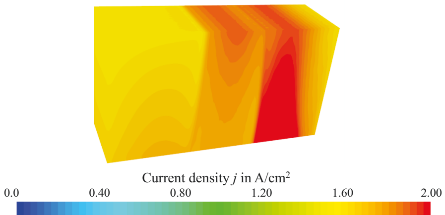
Figure A.29: Current density distribution on anode and cathode reaction planes of 60-cell stack for ID3, corresponding to a voltage of 36.8 V.
