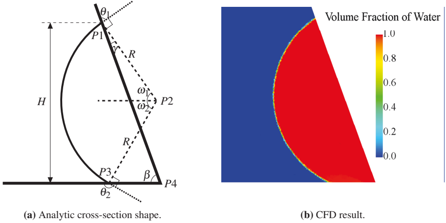
Figure 5.6: Comparison of analytic droplet shape with cross section profile of droplet at 12.3 ms
