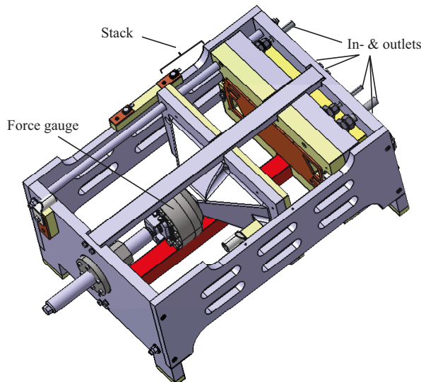
Figure 8.7: Experimental setup for 60-cell measurements.
