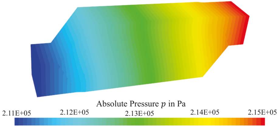
(a) Cathode pressure distribution.
