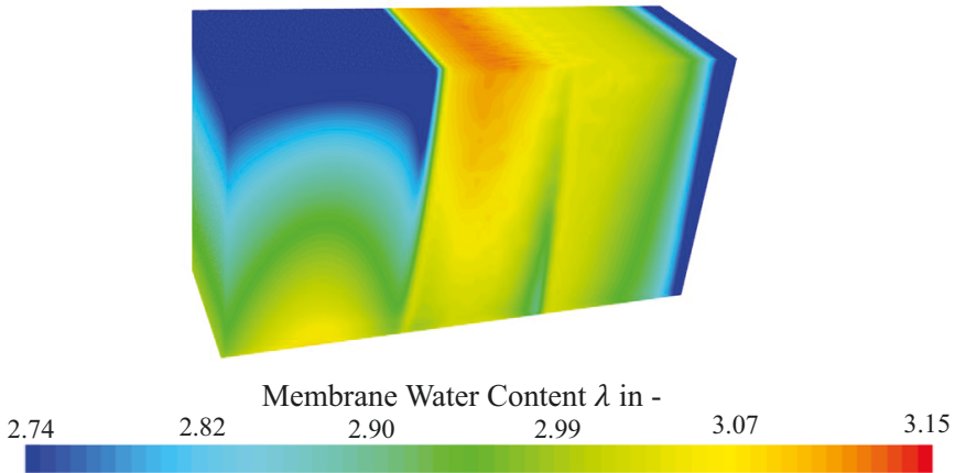
Figure A.26: Membrane water content distribution on anode CL-MEM interface of 60-cell stack for ID3 case, corresponding to a voltage of 49.1 V.
