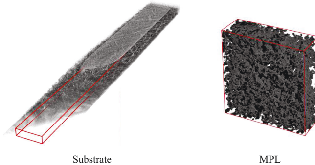
Figure A.13: Representative Volumes (RV) of substrate and MPL, produced via \mu -CT and FIB/SEM-tomographie scan reconstructions.
