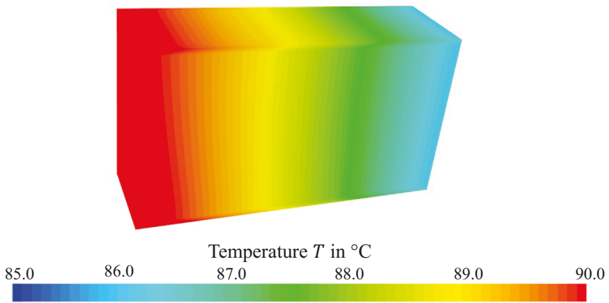
Figure A.28: Temperature distribution in coolant regions of 60-cell stack for ID3, corresponding to a voltage of 36.8 V.
