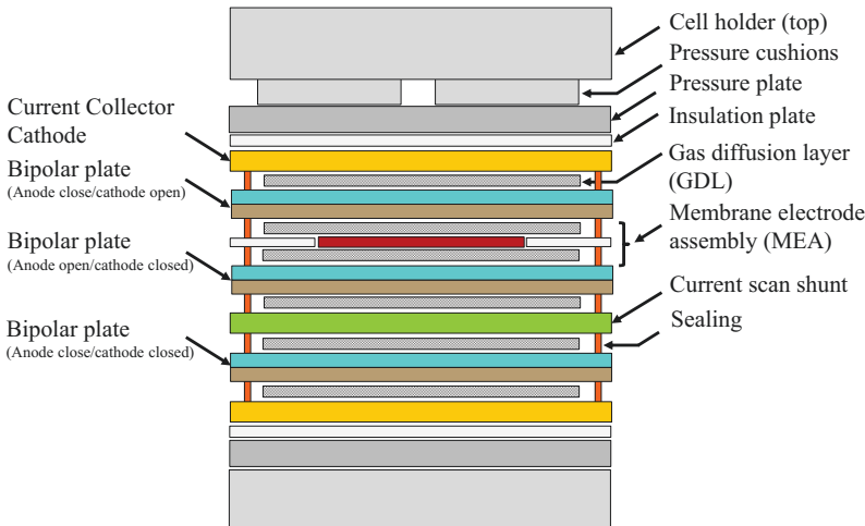
Figure 6.8: Experimental setup for local current (544 segments) and temperature (144 segments) measurement in a single automotive PEM fuel cell according to Herden et. al [96].
