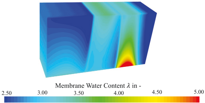
Figure A.30: Membrane water content distribution on anode CL-MEM interface of 60-cell stack for ID3 case, corresponding to a voltage of 36.8 V.
