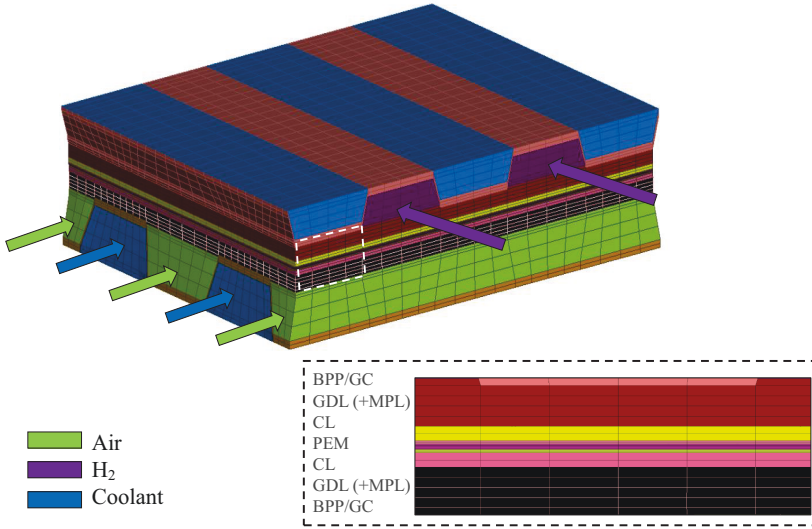
Figure 6.2: Mesh fragment of detailed single cell active area model with indications of fluid inlets.
