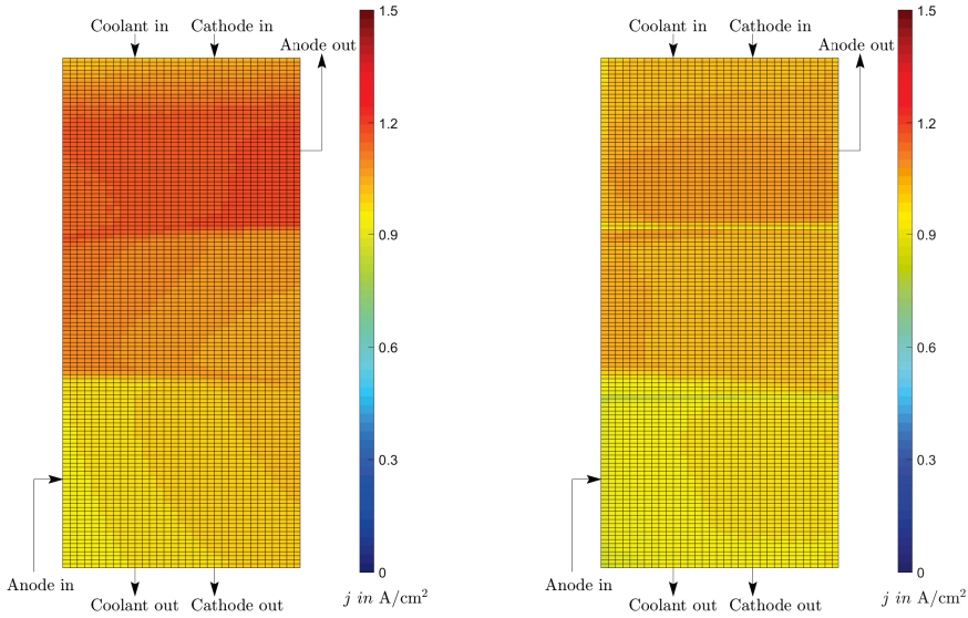
(a) Simplified cell results with j_{\text{avg}} = 1.06 \text{ A}/\text{cm}^2 .
