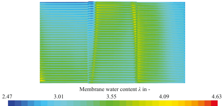
Figure 6.5: Membrane water content plot on anode CL-MEM interface for ID3 case at 0.686 V.
