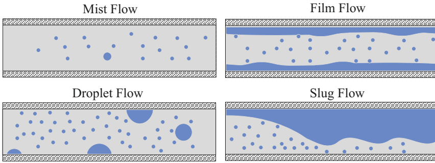
Figure 3.5: Two phase flow regimes inside PEMFC gas channels.
