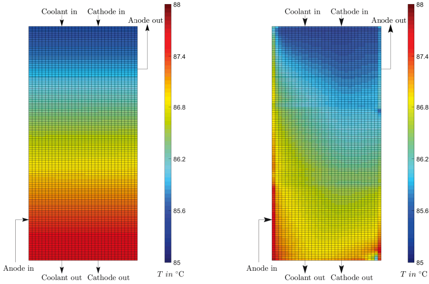
(a) Simplified cell results with j_{\text{avg}} = 1.06 \text{ A/cm}^2 .
