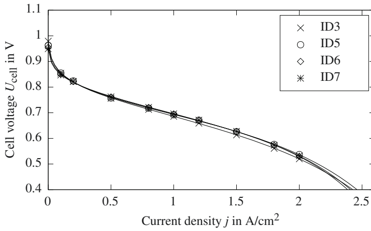
Figure A.20: Experimental polarization curves for relative humidity variation at ID3, ID5, ID6 and ID7.
