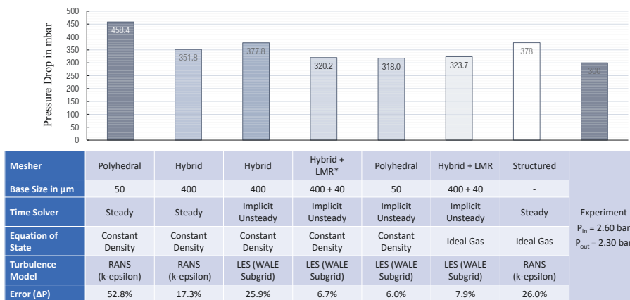
Figure A.16: Mesh independence study for anode flow field single phase pressure drop.
