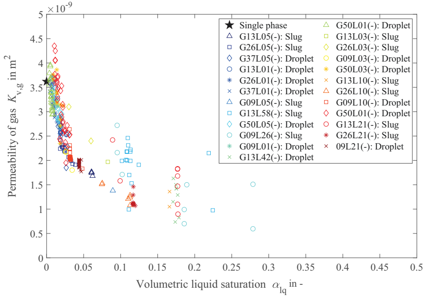
Figure A.11: Raw data of anode gas channel permeabilities from selected cases.
