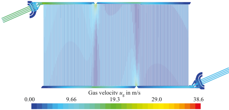
(b) Gas velocity in anode channels.
