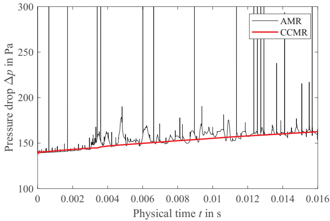
Figure 5.10: Comparison of pressure drop time-series in anode single channel simulation of AMR and CCMR simulation.
