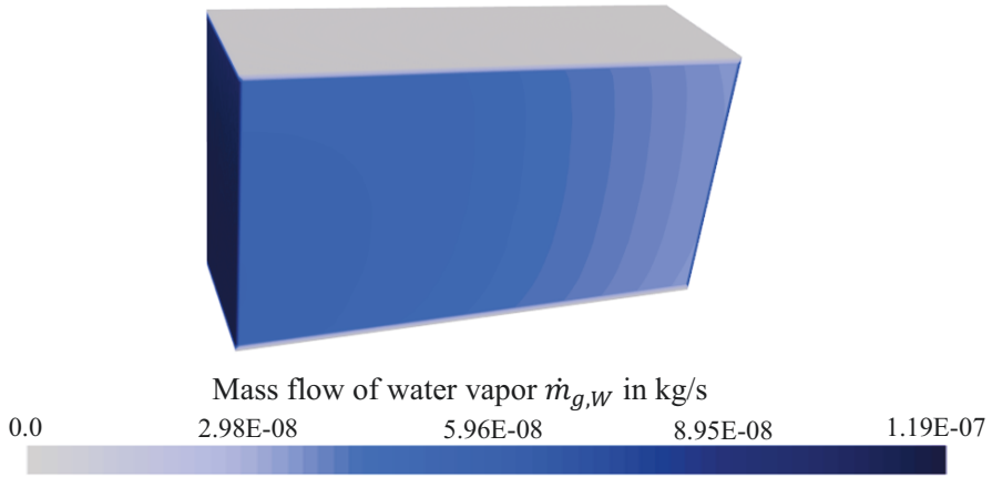
(a) Cathode gas channels.
