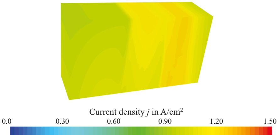
Figure 8.4: Current density distribution on reaction planes of 60-cell stack for ID3 case, corresponding to a voltage of 41.2 V.
