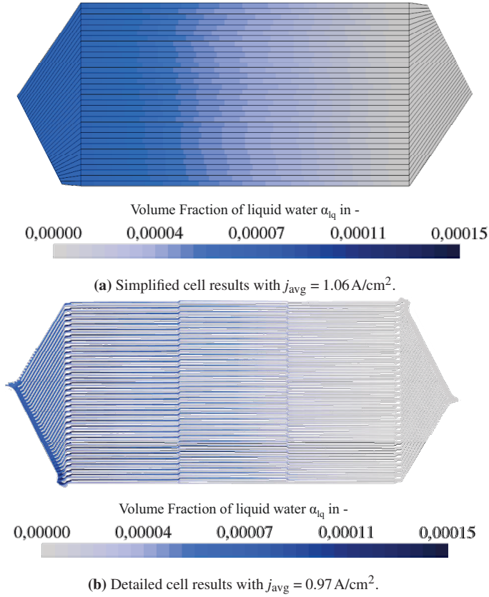
Figure 7.13: Liquid water volume fraction distribution in cathode gas channels of simplified (top) and detailed (bottom) cell simulation for ID3 at 0.686V.
