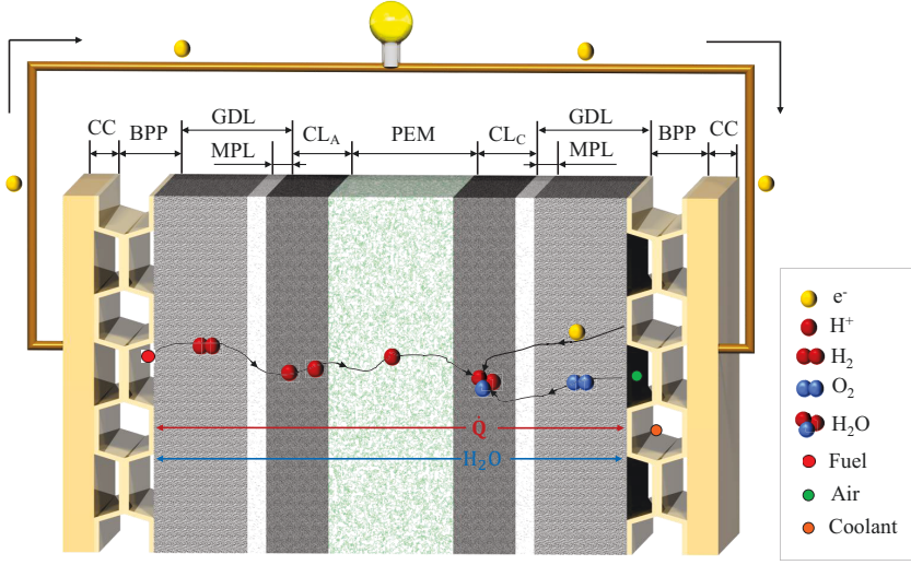
Figure 3.1: Schematic cut-plane through a low temperature PEMFC single cell
