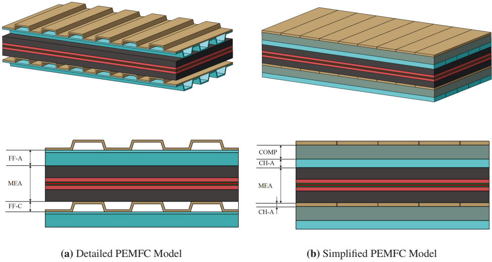
Figure 7.2: Schematic sections of detailed (a) and simplified (b) cell geometry.
