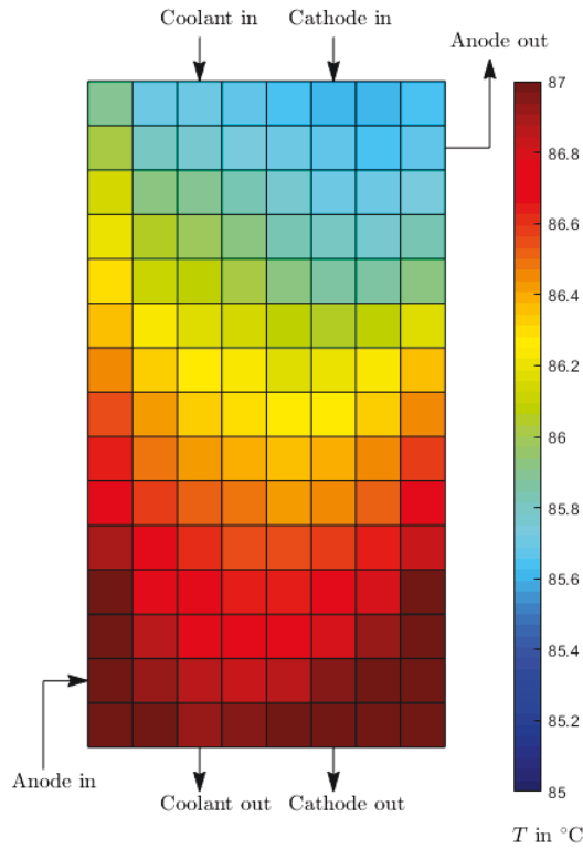
Figure A.19: Temperature profile of uneven coolant introduction simulation of ID3 at 0.686 V.
