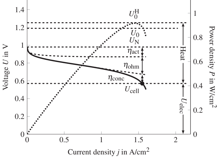
Figure 3.2: General polarization (solid) and power density curve (dotted) of a single PEMFC.
