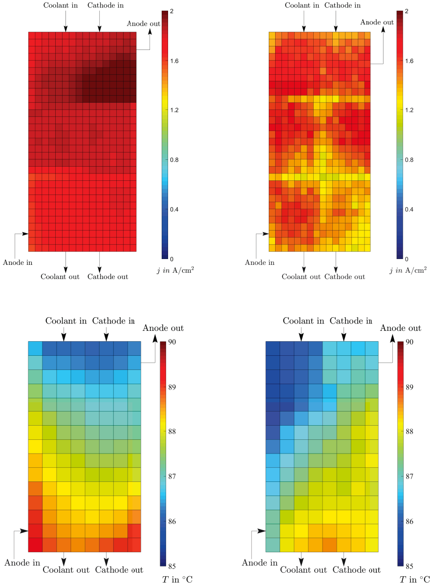
(a) Detailed cell results with j_{\text{avg}} = 1.67 \text{ A/cm}^2 .
