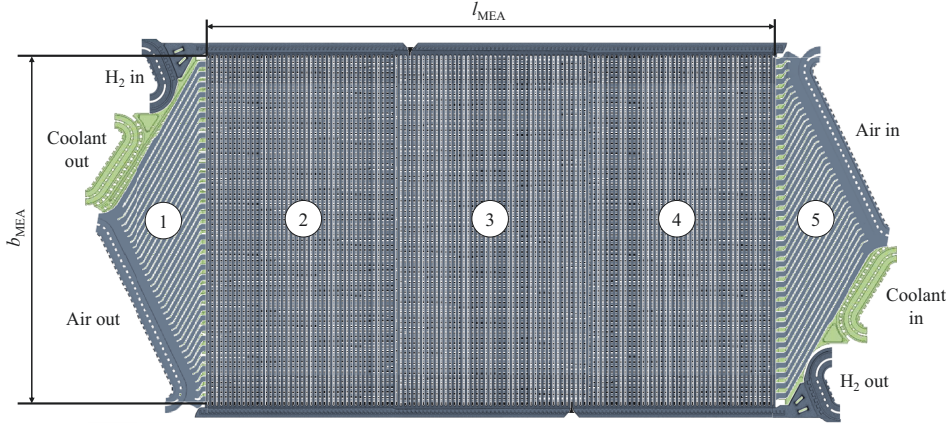
Figure 6.1: Detailed single cell geometry for PEMFC simulations.
