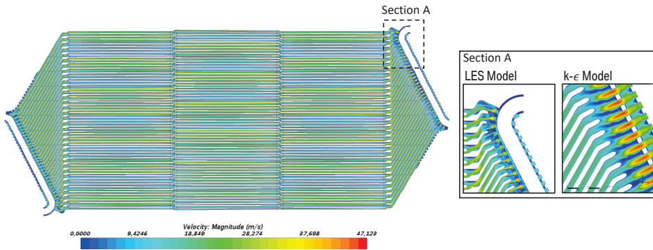
Figure A.14: Velocity profile of cathode flow field cut section plane with indication of turbulence, using an LES and k-\epsilon approach with inlet air mass flows, corresponding to \lambda_C = 4 at j_{\text{avg}} = 2.5\text{ A/cm}^2 .
