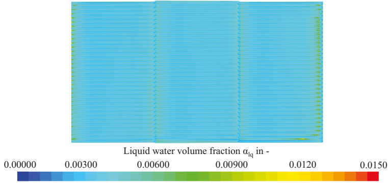
Figure 6.4: Liquid water volume fraction plot on anode CL-MEM interface for ID3 case at 0.686 V.
