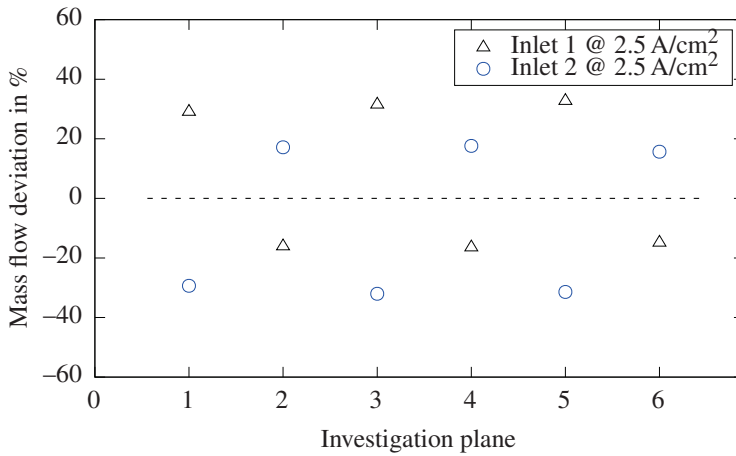
Figure A.3: Exchange mass flow rate from 4-repetition unit simulation of cathode gas channels at 2.5 A/cm².
