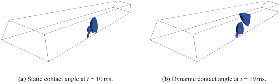
Figure 5.4: Water volume fraction iso-surface plots of static (left) and dynamic (right) contact angle case.
