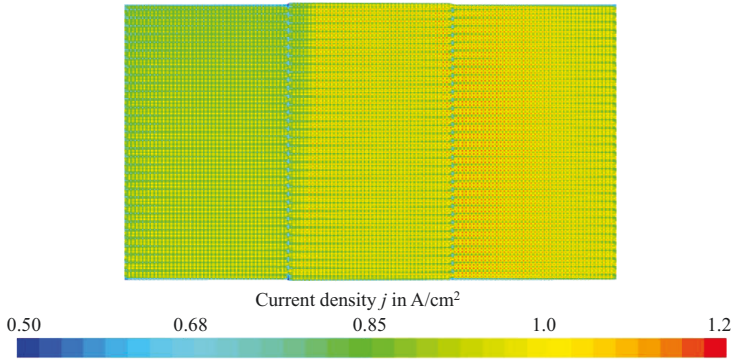
Figure 6.7: Current density plot on anode CL-MEM interface for ID3 case at 0.686 V.
