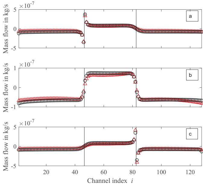
Figure 7.7: Mass flow comparison between detailed (red triangle) and simplified model (black circle) for anode flow field, evaluated on plane cut a (top), b (middle) and c (bottom).
