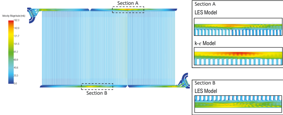
Figure A.15: Velocity profile of anode flow field cut section plane with indication of turbulence, using an LES and k- \epsilon approach with inlet hydrogen mass flows, corresponding to \lambda_A = 4 at j_{avg} = 2.5 \text{ A/cm}^2 .
