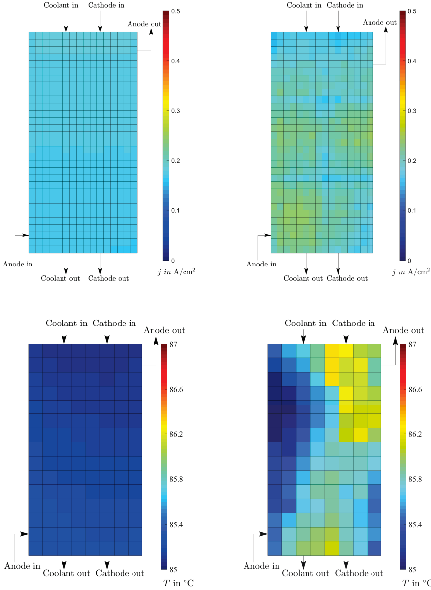
Figure A.18: Current density (top) and temperature (bottom) distribution of detailed cell simulation (left) and experimental cell (right) results of ID3 at 0.819 V.
