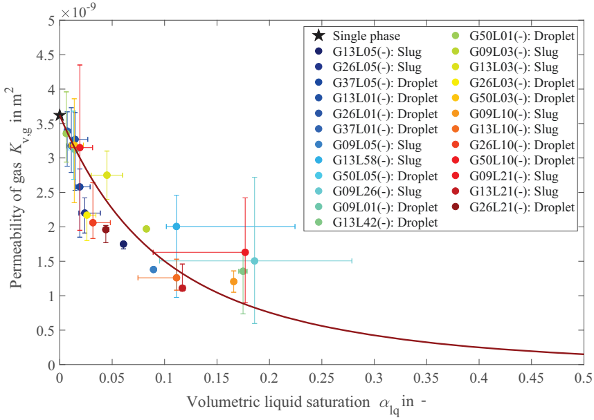
Figure 5.15: Anode gas channel permeability correlation constructed from selected cases with indication of variation bars for the respective case.
