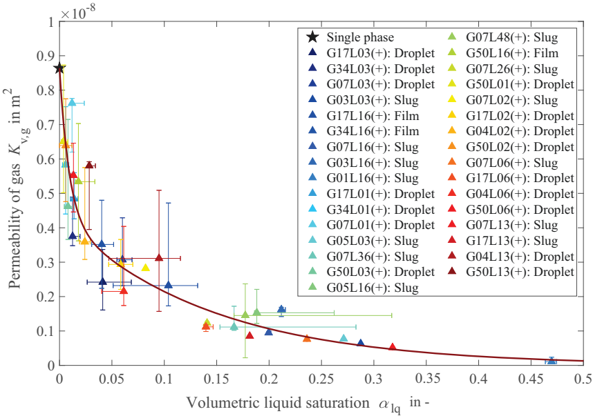
Figure 5.16: Cathode gas channel permeability correlation constructed from selected cases with indication of variation bars for the respective case.
