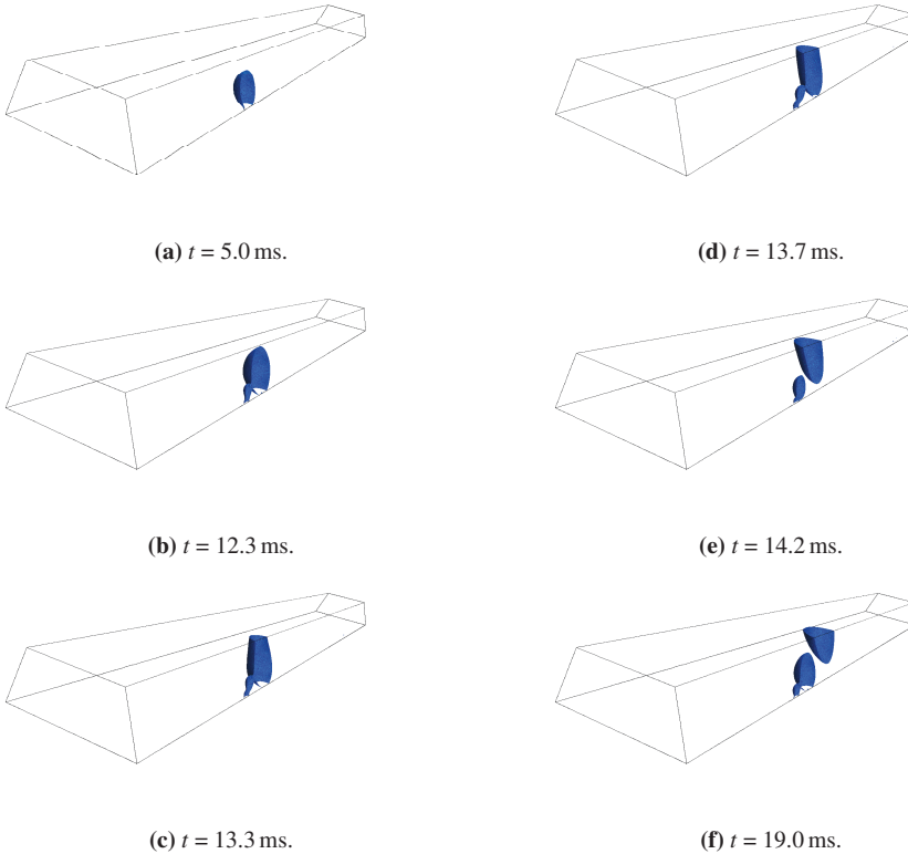
Figure 5.5: Water volume iso-surface plots at physical times of 5.0, 12.3, 13.3, 13.7, 14.2 and 19 ms. Air flows from left to right.
