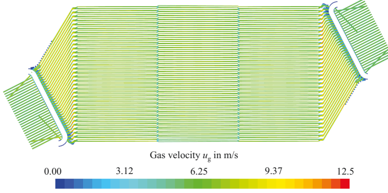
(a) Gas velocity in cathode channels.
