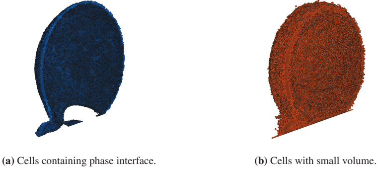
Figure 5.3: Comparison of phase interface region \Omega_{\text{refine}} ( 0.01 < \alpha < 0.99 , left) to region of small cells (right).
