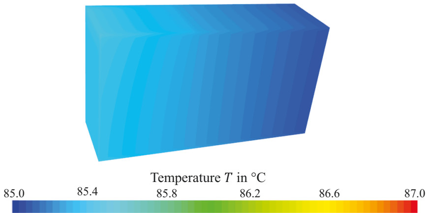
Figure A.24: Temperature distribution in coolant regions of 60-cell stack for ID3, corresponding to a voltage of 49.1 V.
