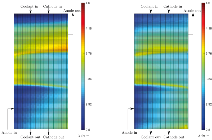
(a) Simplified cell results with j_{avg} = 1.06 \text{ A/cm}^2 .
