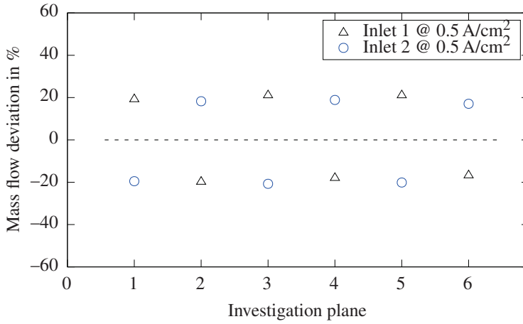
Figure A.2: Exchange mass flow rate from 4-repetition unit simulation of cathode gas channels at 0.5 A/cm².
