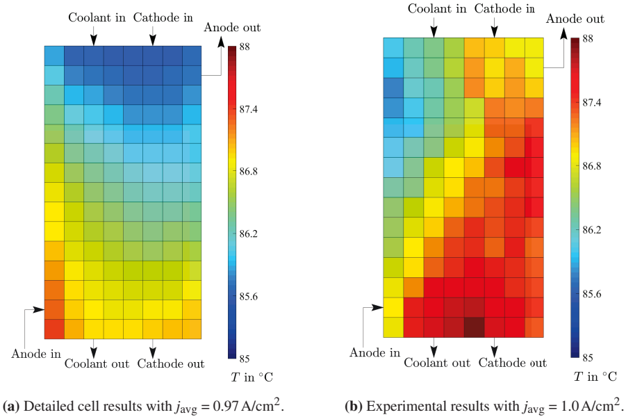
Figure 6.11: Temperature distribution of detailed cell simulation (left) and experimental cell (right) results at 0.686V A/cm 2 .
