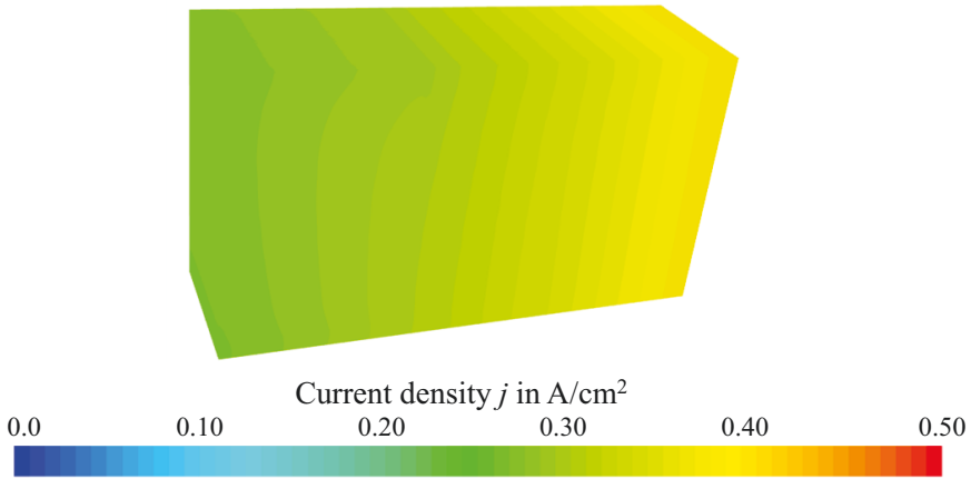
Figure A.25: Current density distribution on anode and cathode reaction planes of 60-cell stack for ID3, corresponding to a voltage of 49.1 V.
