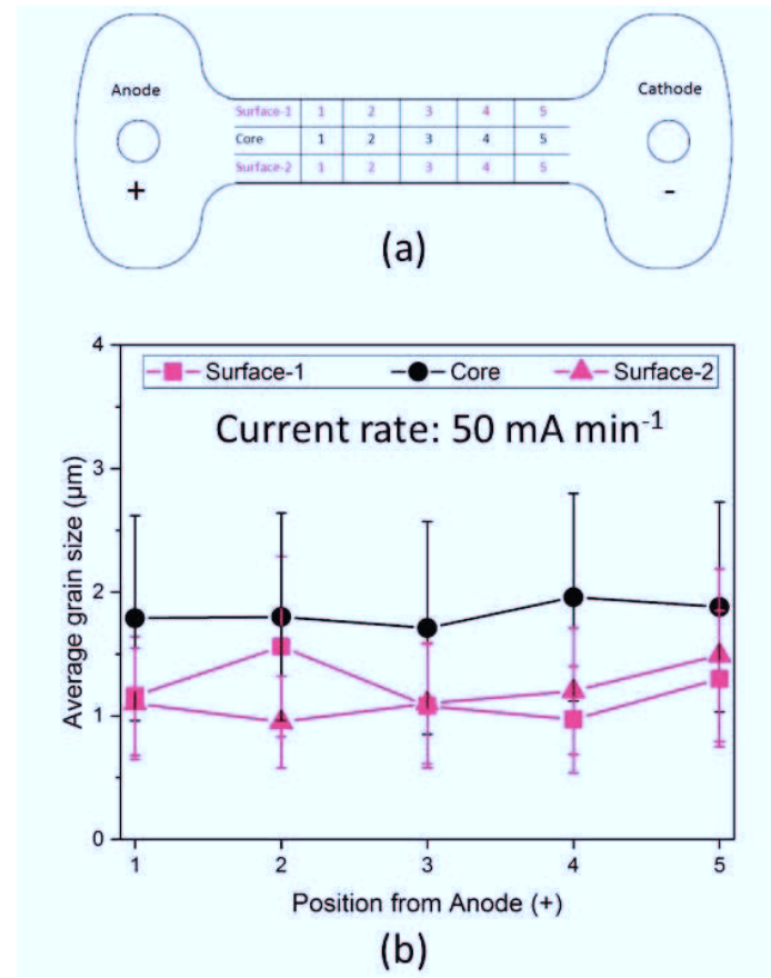
Figure 4-56 : (a) Position at the gage section where the SEM micrographs were taken for estimating the average grain size and (b) average grain size at different position of the gage section as shown in (a), the sample was flash sintered in current rate (CR) flash mode, at a current-rate of 50 mA min -1 [208].
