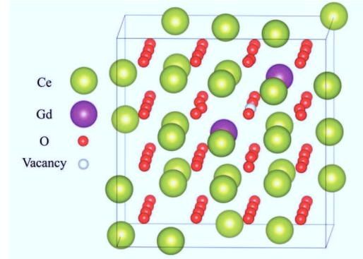
Figure 1-2 : The lowest-energy GDC configuration with one vacancy and two Gd cations, adapted from Asher et. al. [14]
