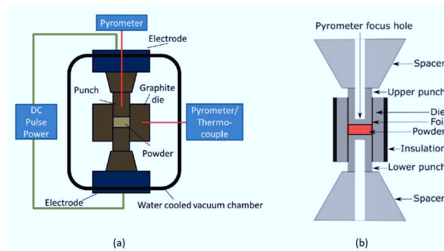
Figure 2-8 : General schematics of the (a) FAST/SPS process set-up [70] and (b) general tooling assembly
