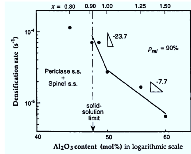
Figure 2-3 : Dependence of densification rate on MgO and \text{Al}_2\text{O}_3 content at 1600°C, Reprinted with permission from [49].
