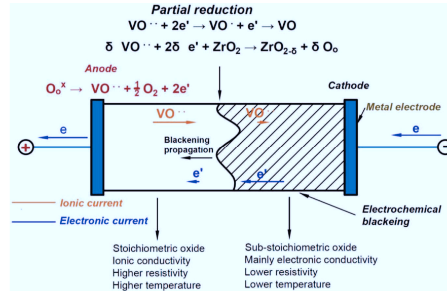
Figure 2-18 : Schematic representation of the electrochemical reactions and the propagation of the electrochemical blackening in 8YSZ during DC flash sintering [142].
