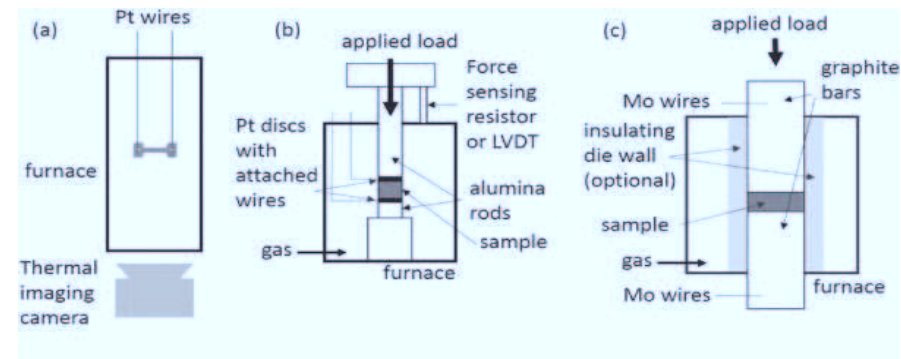
Figure 2-13 : Different flash sintering setup; (a) vertical tube furnace with dog-bone sample, (b) adapted dilatometer/mechanical loading frame and (c) flash spark plasma sintering/adapted hot press, Reprinted with permission from [31].
