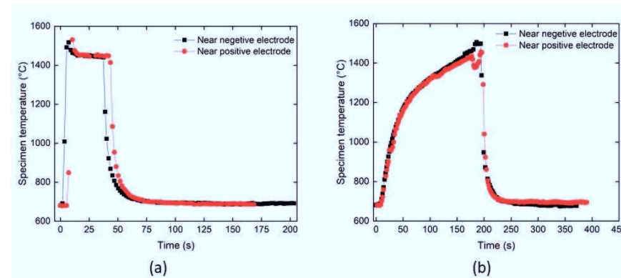
Figure 4-65 : Evolution of the sample temperature calculated from the lattice expansion during flash sintering: (a) voltage-to-current flash and (b) current rate flash. The base line peak as shown in Fig. 4-62 was used for calculation of the actual sample temperature.
