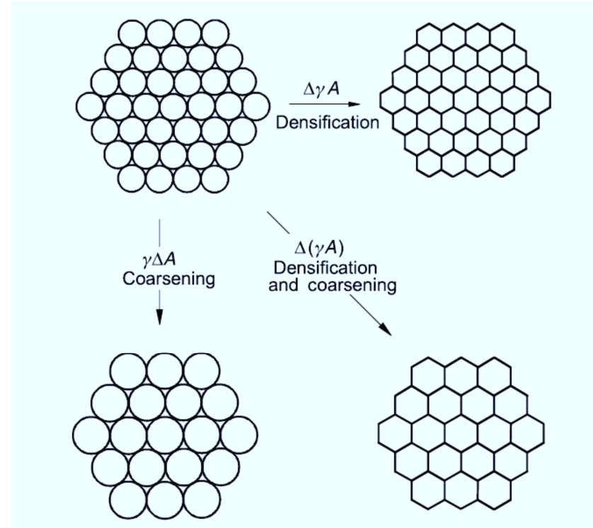
Figure 2-1 : Schematic representation of densification and coarsening from powder compact. [43]
