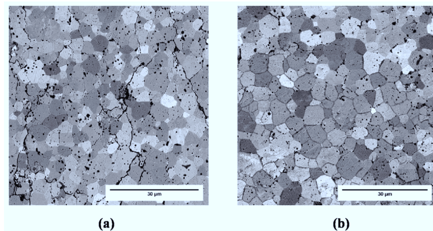
Figure 4-33 : Micrographs of pressure less (PL) sintered samples: (a) cracks formation after sintering in Ar/2.9%H 2 , (b) nearly crack-free structure after sintering in Ar-2.9%H 2 with subsequent re-oxidation [183].
