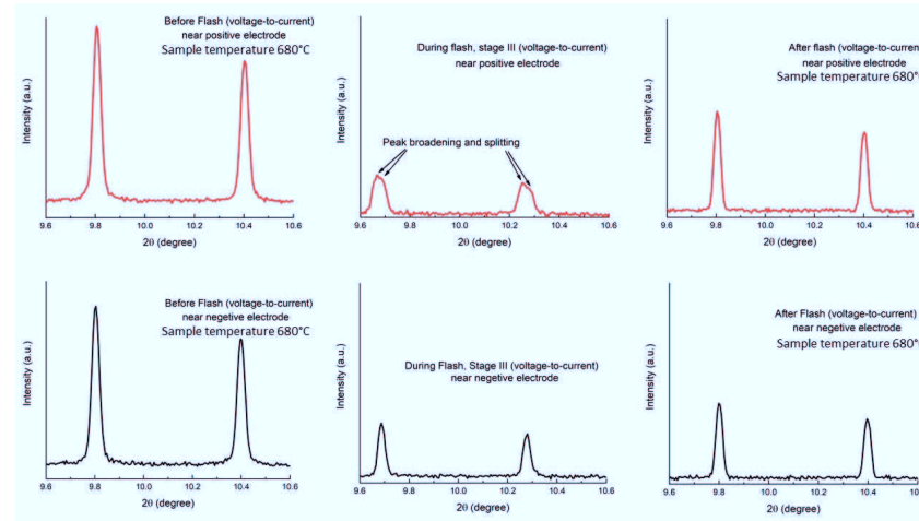
Figure 4-64 : Expanded view of the diffraction peaks before flash (at 680°C), during flash (at stage III) and after flash (at 680°C) near the positive and negative electrode, indicating a second effect in the lattice during flash in addition to the lattice expansion.
