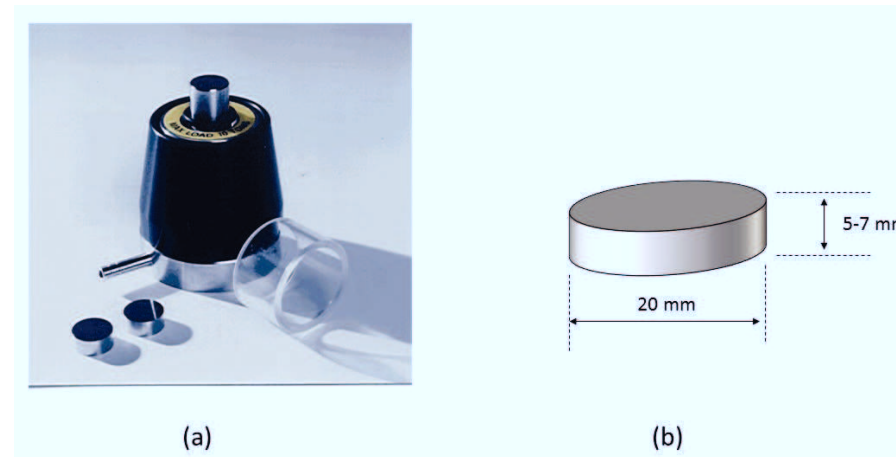
Figure 3-1 : (a) Evacuatable pressing tool used for preparing pellet shaped samples and (b) sketch of the pellet used for conventional free sintering studies
