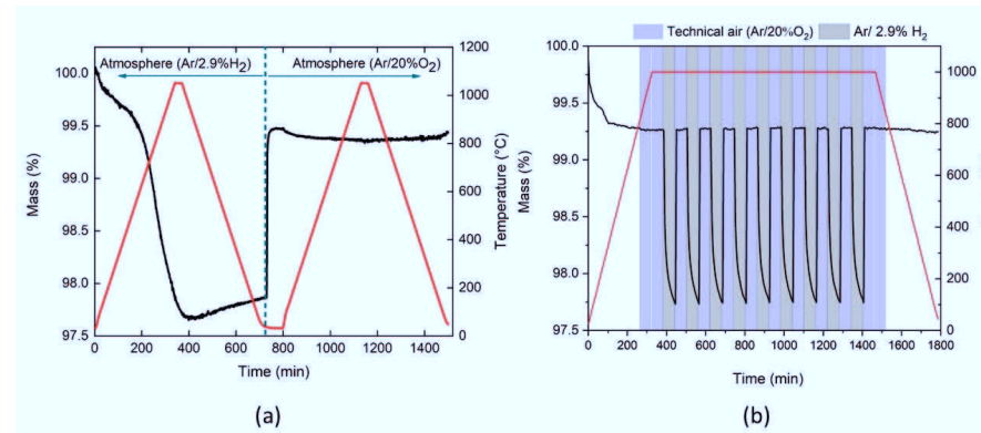
Figure 4-19 : (a) TG curves for GDC10 powder to see the redox behavior of the material, the powder sample was heated and cooled in Ar/2.9%H 2 and then atmosphere was switched to Ar/20%O 2 . The maximum temperature was 1000°C and the dwelling time was 30 minutes at the maximum temperature with a heating/cooling rate of 3°C/minute, (b) change in mass due to the change in atmosphere under isothermal temperature of 1000°C [183].
