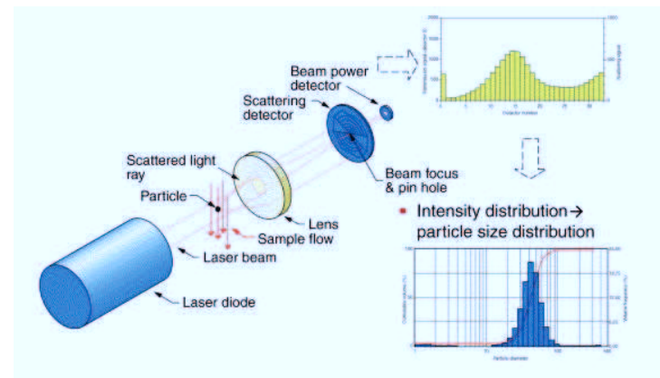
Figure 3-10 : Schematic representation of the principle of the laser diffraction analysis for measuring the particle size distribution (PSD), Reprinted with permission from [174].
