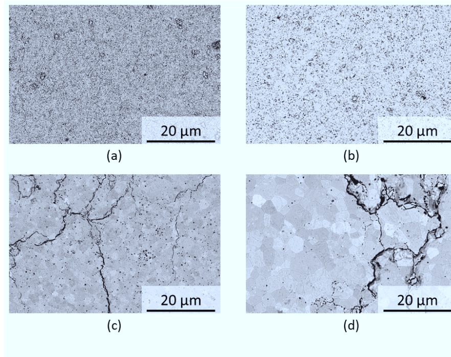
Figure 4-12 : SEM micrograph at low magnification of the polished and thermally etched surface showing the grains and micro-cracks formation, sample sintered at (a) 1100°C, (b) 1200°C, (c) 1300°C and (d) 1400°C with 30 minutes dwelling time under Ar/2.9% H 2 .
