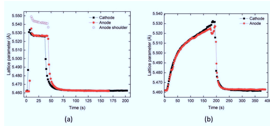
Figure 4-63 : Change in lattice parameters during flash sintering experiment in real time: (a) voltage-to-current flash sintering, occurrence of peak splitting on anode side and (b) current rate flash sintering.
