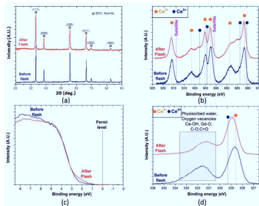
Figure 4-40 :Comparison between GDC10 samples before and after flash in air: (a) XRD spectra (b) XPS spectra of Ce 3d (c) valance band edge; and (d) O 1s XPS spectra (note that the signal at 531-533 eV is mainly related to surface impurities) [199].
