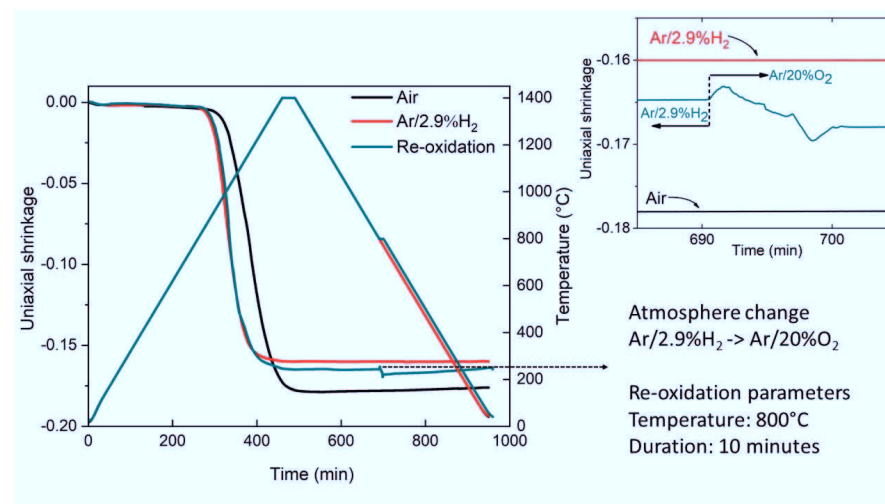
Figure 4-17 : True uniaxial shrinkage of GDC10 under entirely air, entirely Ar/2.9%H 2 atmosphere and partially under Ar/2.9%H 2 atmosphere and during cooling at 800°C re-oxidation, the inset graph shows with higher resolution the shrinkage during the re-oxidation.
