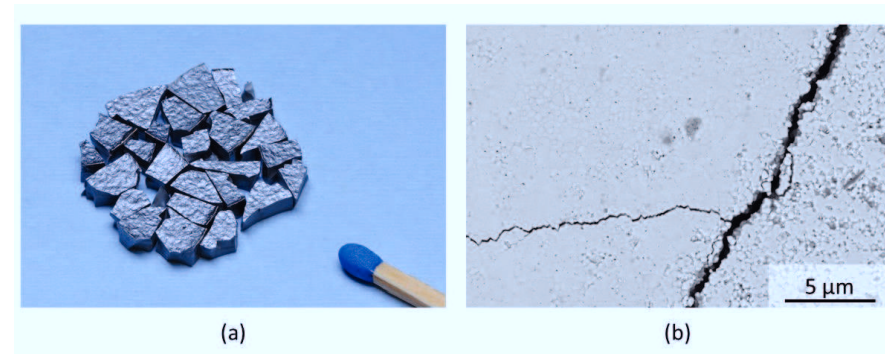
Figure 4-27 : (a) Optical image of the dense GDC10 sample fabricated by FAST/SPS at a sintering temperature of 1200°C with a dwelling time of 6 minutes and (b) SEM micrograph of the sample showing presence of typical micro-cracks in the FAST/SPS sintered GDC10 sample.
