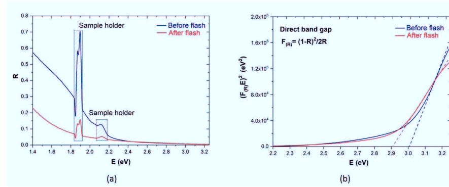
Figure 4-41 : (a) Diffuse reflectance ( R ); and (b) (F_R)E^2 vs. photon energy ( E ) plot for the determination of optical band gap of GDC10 before and after flash sintering [199].
