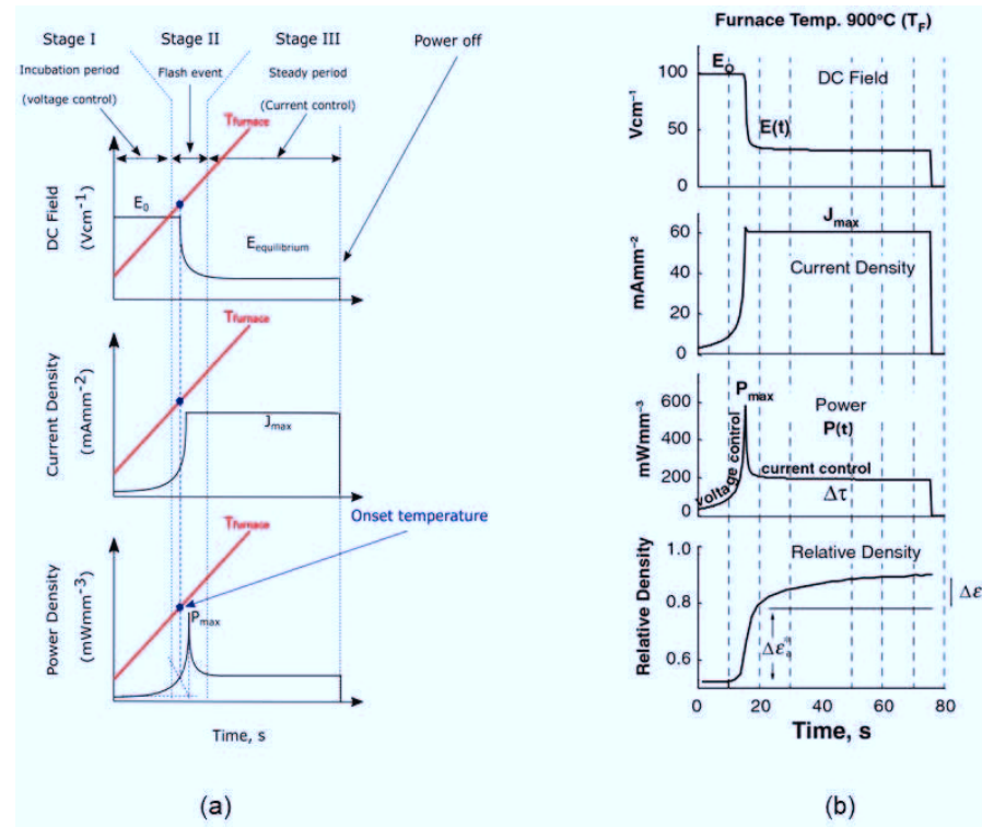
Figure 2-12 : (a) Schematic sketch of three distinct stages in a constant heating rate (CHR) flash sintering experiment, where the furnace temperature is raised at a constant rate (typically 10^\circ C \text{ min}^{-1} ) and (b) Interplay between electrical field, current density, power density and densification for a real iso-thermal flash sintering cycle for 3YSZ dog-bone sample, Reprinted with permission from [124].
