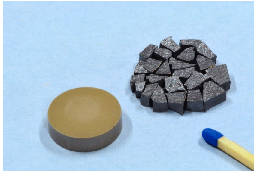
Figure 4-32 : Comparison of the FAST/SPS sintered pellets: (dark yellow and stable) with pressure less (PL) tool configuration under Ar/2.9%H 2 atmosphere and re-oxidation at 800°C and (black and fractured) with conventional pressure assisted (PA) tool under Ar/2.9%H 2 atmosphere [192].
