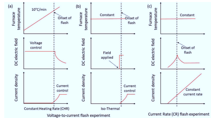
Figure 3-9 : Different flash mode used in the current work: (a) constant heating rate, voltage-to-current flash experiment, (b) iso-thermal, voltage-to-current flash experiment and (c) current rate flash experiment
