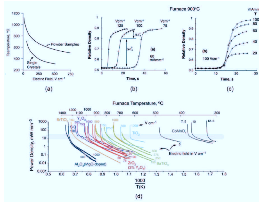
Figure 2-17 : (a) comparison of the onset temperature for single crystal and powder pressed 8-10 mol% yttria stabilized zirconia (YSZ) dog-bone shaped samples in one graph, Reprinted with permission from [141], (b) Influence of the electrical field on the incubation time and densification for 3YSZ samples, (c) influence of the maximum current density on the densification for 3YSZ samples, Reprinted with permission from [124] and (d) Arrhenius plots of power density for several ceramics showing the onset of flash occurred within a narrow band of power density, Reprinted with permission from [121].
