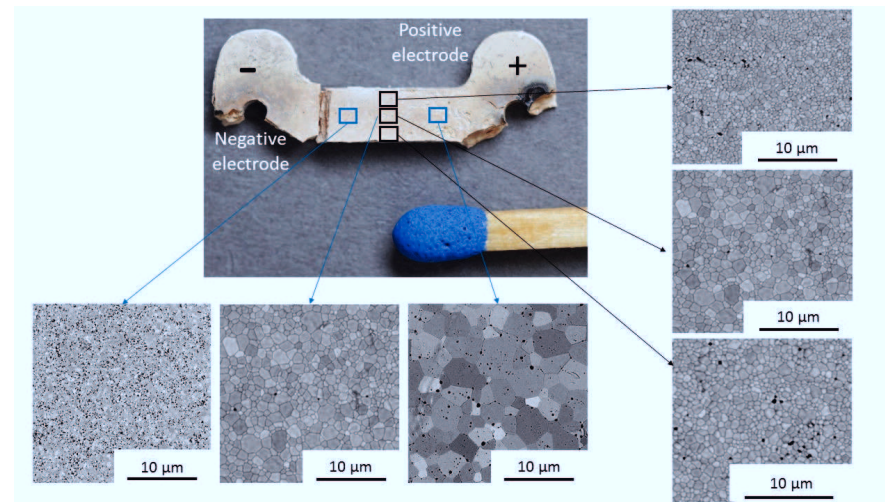
Figure 4-48 : SEM micrographs at different positions of a sample belonging to the safe region.
