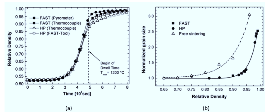
Figure 2-10 : Comparison between HP and FAST/SPS of submicron alumina: (a) Densification curve and (b) sintering trajectory, Reprinted with permission from [98].
