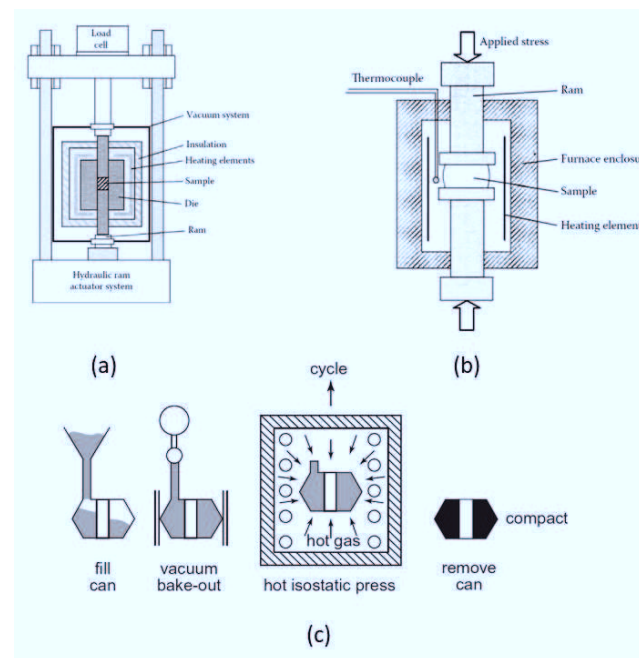
Figure 2-6 : Schematic of pressure assisted sintering techniques; (a) hot pressing, where pressure is applied along the vertical axis [41], (b) sinter forging [41] and (c) hot isostatic process, illustrating different steps involved in the HIP process [57]
