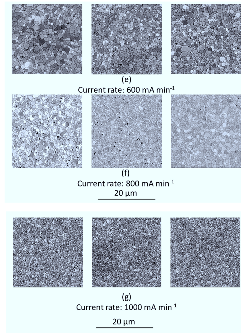
Figure 4-57 : SEM micrographs at three different positions, the positions could be visualized from the Fig. 4-56 (a) (i.e. left image: near the anode (core 1), middle image: at the center (core 3) of the sample and right image: near the cathode (core 5)) of the CR Flash sintered samples at seven different current rates, showing that higher current rates resulted in finer grain size and homogeneous grain size distribution along the gage section of the sample [208].
