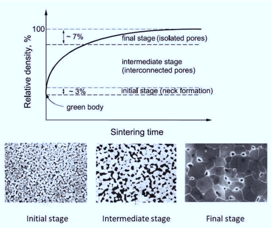
Figure 2-5 : Schematic representation of three different sintering stages of a powder compact and example of associated microstructure and grain size evolution [41,43]
