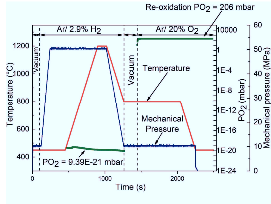
Figure 4-29 : FAST/SPS cycle under reducing atmosphere and controlled re-oxidation at 800°C during cooling showing the temperature, pressure, FAST/SPS chamber pressure and measured P(O_2) [183].
