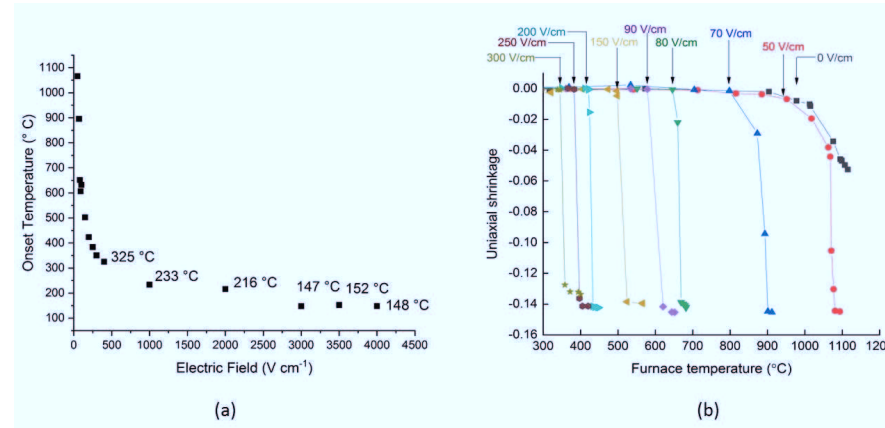
Figure 4-43 : (a) The furnace temperature for the onset of flash as a function of electric field and (b) Uniaxial shrinkage during the constant heating rate experiments at different electric fields.
