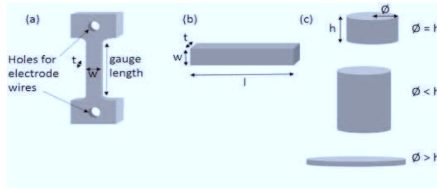
Figure 2-14 : Different specimen geometries used in flash sintering studies; (a) dog-bone shaped, (b) rectangle bar and (c) pellets, of different height: diameter ratios, Reprinted with permission from [31].
