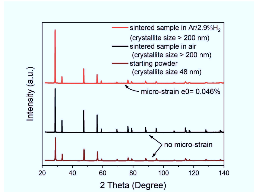
Figure 4-16 : XRD patterns of sintered GDC10 sample in air, \text{Ar}/2.9\%\text{H}_2 and starting powder.
