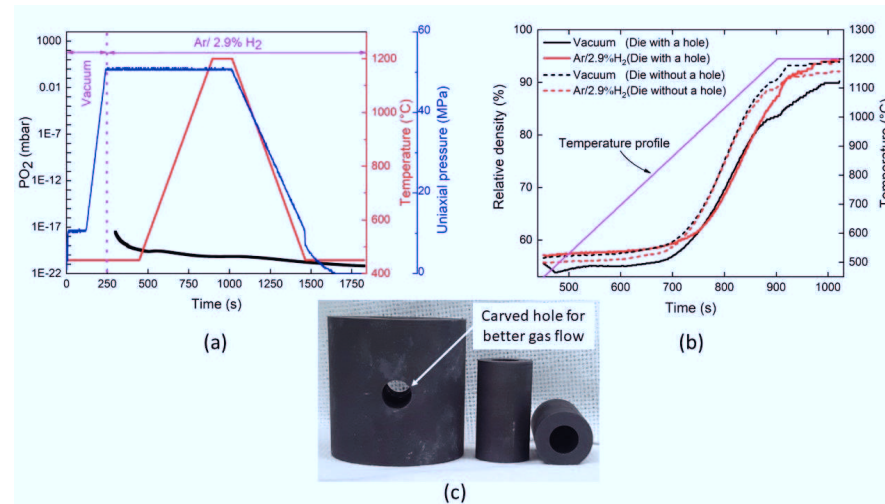
Figure 4-28 : (a) FAST/SPS cycle under reducing atmosphere showing the temperature, pressure, FAST/SPS chamber pressure and measured ( PO_2 ) (b) evolution of density under vacuum and Ar/2.9%H 2 for conventional tool configuration (PA) with and without a hole and (c) image showing the carved out hole in the die for better gas flow to the sample.
