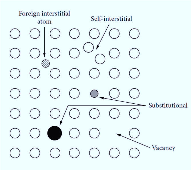
Figure 2-2 : Schematic illustration of different point defects in a crystalline solid [41]
