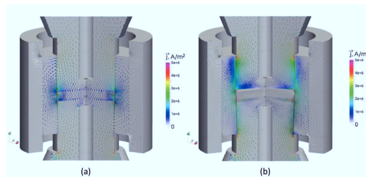
Figure 2-9 : Schematic of the current flow for the tool and sample assembly; (a) conductive powder and die, (b) non-conductive powder and conductive die, Reprinted with permission from [70].
