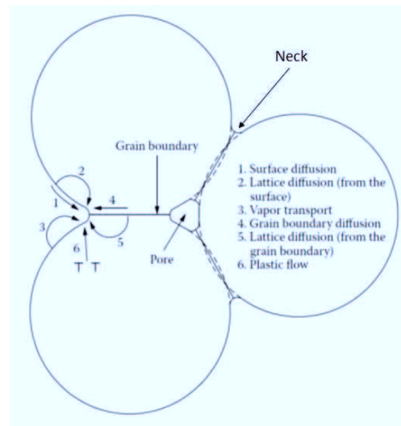
Figure 2-4 : Material transport paths during sintering and associated six different mechanisms [41]
