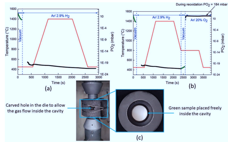
Figure 4-31 : FAST/SPS cycle with the pressure less (PL) tool configuration: (a) FAST/SPS cycle entirely under reducing atmosphere, (b) FAST/SPS cycle under reducing atmosphere and re-oxidation at 800°C and (c) image of the tool showing the carved out hole in the die for better gas flow and placement of the sample freely to allow volume expansions.
