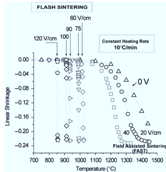
Figure 2-11 : Flash sintering of 3 mol% Yittria Stabilized Zirconia (3YSZ); flash sintering occurred at >60 \text{ Vcm}^{-1} DC electric field, Reprinted with permission from [33].
