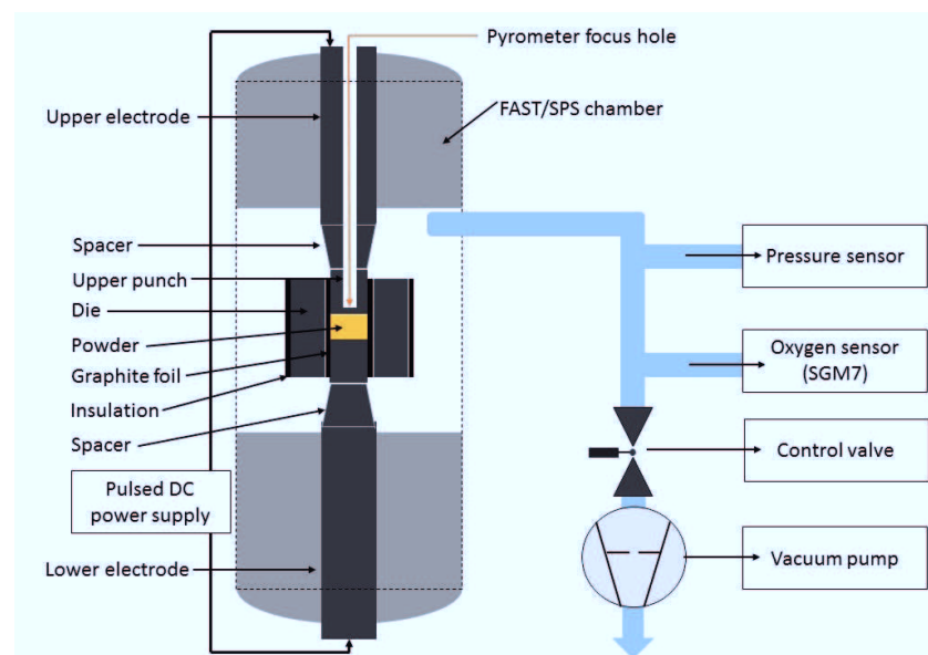
Figure 3-5 : Sketch of the FAST/SPS device showing the position of the oxygen sensor.
