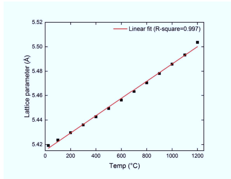
Figure 4-62 : Lattice parameter as a function of temperature for GDC10 in air measured by high temperature X-ray diffraction (measured at IEK-1, Forschungszentrum Juelich).
