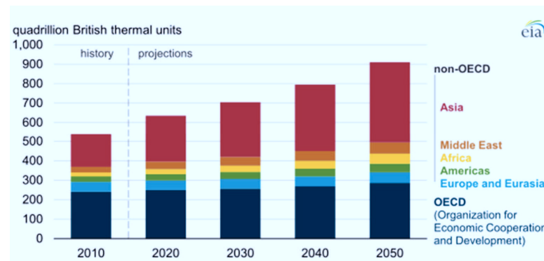
Figure 1-1 : Global primary energy consumption by region between 2010 and 2050 [1]
