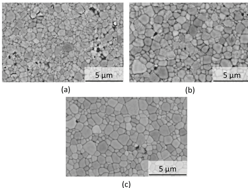
Figure 4-10 : SEM micrograph of the polished and thermally etched surface showing the grain, microstructure of samples sintered at (a) 1350°C, (b) 1400°C and (c) 1450°C with 30 minutes dwelling time in air.
