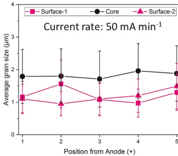
Figure 4-56 : (a) Position at the gage section where the SEM micrographs were taken for estimating the average grain size and (b) average grain size at different position of the gage section as shown in (a), the sample was flash sintered in current rate (CR) flash mode, at a current-rate of 50 mA min -1 [208].
