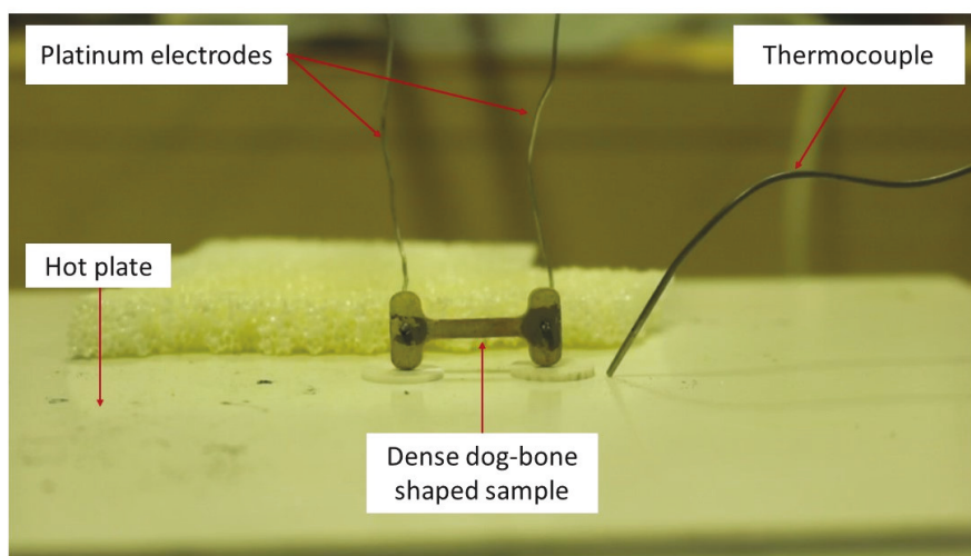
Figure 3-8 : Iso-thermal flash experiment on a hot plate with dense GDC10 sample at a constant temperature of 280°C, applied DC field 150 \text{ Vcm}^{-1} and maximum current density 25 \text{ mA mm}^{-2} . The chromatic alteration of the sample is observed by using a CCD camera.
