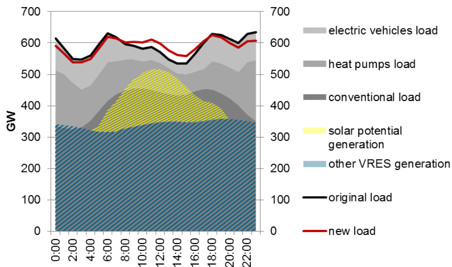
Figure 6. Total European load (before and after load shifting) and VRES potential profiles, averaged for each hour of the year.
