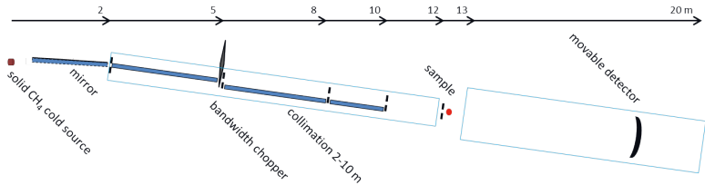
Figure VI.10: Schematic layout of the high resolution SANS instrument
