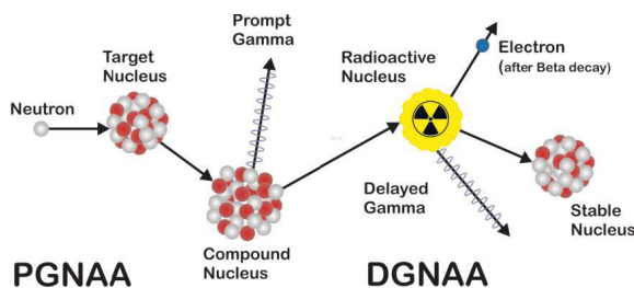
Figure IV.11: PGAA and NAA mechanism
