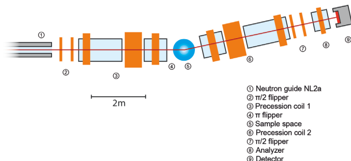
Figure VI.17: NSE instrument schema as realized for the J-NSE at MLZ. The segmented main coils guarantee an optimized field homogeneity for high resolution, for a pulsed source such as the HBS only the \pi/2 -flippers and the \pi -flipper need to be ramped with the incoming neutron wavelength during the pulse arrival, as has been realized at the SNS-NSE. All other magnetic fields are static during measurement of a Fourier time.
