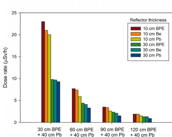
Figure V.64: Dose rate at surface of shielding after shut-down of the proton beamline and 360 days of irradiation of the tantalum target without interruption.
