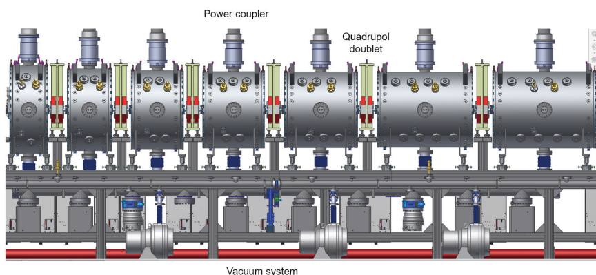
Figure V.22: The modular design of the HBS CH-DTL provides good access for maintenance and repair.
