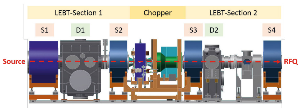
Figure V.14: Scheme of the low energy beam transport for HBS. It consists of two sections with an E×B-chopper in between.
