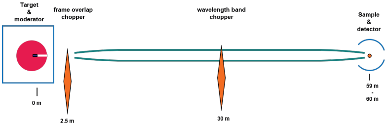
Figure VI.6: Schematic layout of diffractometer for nanoscaled and disordered materials
