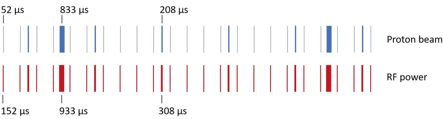
Figure V.3: Pulse scheme of the HBS linac showing pulses of the three different frequencies of 24 Hz (pulse length 833 \mu s), 96 Hz (pulse length 208 \mu s) and 384 Hz (pulse length 52 \mu s) to be delivered. The spacing in time between the short proton beam pulses is 2.548 ms (384 Hz). The longer pulses are centered between these short pulses. The pulses of the RF power supply always begin 100 \mu s earlier than the proton pulses.
