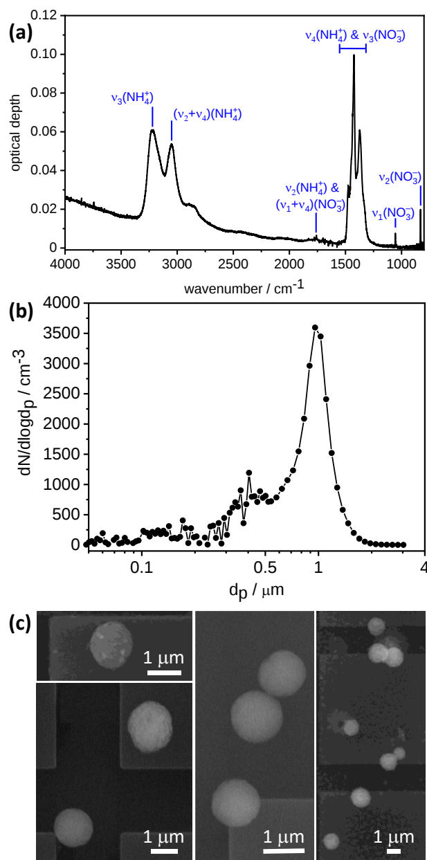
630 Figure 2: (a) Infrared extinction spectrum of crystalline AN particles recorded at 223 K. The notation of the AN vibrational modes is according to Fernandes et al. (1979). (b) Concomitant number size distribution of the almost pure AN particles crystallized from solution droplets with 99.4 mol% AN and 0.6 mol% AS. The data are shown as a function of the equal-volume sphere diameter, d_p , as obtained by converting the mobility and aerodynamic size spectra from the SMPS and APS measurements with \rho(\text{AN}) = 1.72 \text{ g cm}^{-3} and \chi = 1.1 . (c) Exemplary electron microscope images of filter-sampled, continuously cooled AN crystals from a crystallization experiment with 97.1 mol% AN and 2.9 mol% AS.
