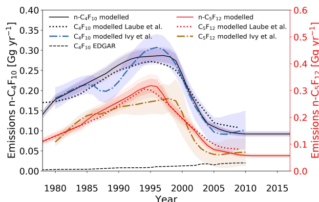
Figure 8. Estimated global emission rates for \text{n-C}_4\text{F}_{10} and \text{n-C}_5\text{F}_{12} (full black and red lines, respectively) in this study, global emission rates for \text{C}_4\text{F}_{10} as reported in the EDGARv4.2 database (dashed black line; no distinction between isomers), modelled emissions by Ivy et al. (2012b) for \text{C}_4\text{F}_{10} and \text{C}_5\text{F}_{12} (dash-dotted blue and brown lines, respectively; no distinction between isomers), and modelled emissions by Laube et al. (2012) for \text{C}_4\text{F}_{10} and \text{C}_5\text{F}_{12} (dotted black and red lines, respectively; no distinction between isomers). Note that the maximum EDGARv4.2 emission rate for \text{n-C}_5\text{F}_{12} is less than 0.6 \times 10^{-4} and is therefore not plotted here. Shadings illustrate the uncertainties.
