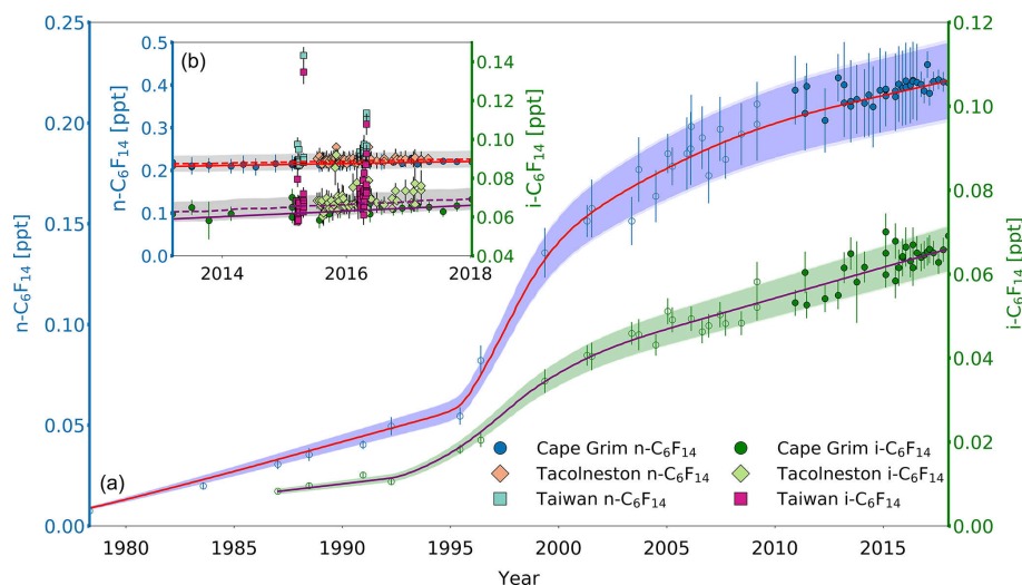
Figure 5. (a) Mixing ratios at Cape Grim of n\text{-C}_6\text{F}_{14} (blue circles, left axis) between 1978 and 2018 and i\text{-C}_6\text{F}_{14} (green circles, right axis) between 1987 and 2018. Data prior to 2010 are shown as empty symbols (Laube et al., 2012), while data from samples collected after 2010 are shown as filled symbols to illustrate the part of the time series that is extended in the current work. Note that the data from Laube et al. (2012) have been converted to a new and improved calibration scale. The atmospheric trends simulated by the model are represented by the red line for n\text{-C}_6\text{F}_{14} and by magenta line for i\text{-C}_6\text{F}_{14} . Total uncertainties (light blue for n\text{-C}_6\text{F}_{14} , light green for i\text{-C}_6\text{F}_{14} ) and trend uncertainties (dark blue for n\text{-C}_6\text{F}_{14} , dark green for i\text{-C}_6\text{F}_{14} ) are indicated with the shaded areas along the trend line. Note that there is only a very small difference between the trend and total uncertainties, and thus the latter is difficult to distinguish. (b) n\text{-C}_6\text{F}_{14} mixing ratios after 2010 (left axis) for Cape Grim (blue circles, left axis), for Tacolneston (orange diamonds), and Taiwan (light blue squares); i\text{-C}_6\text{F}_{14} mixing ratios (right axis) after 2010 for Cape Grim (green circles, right axis), for Tacolneston (light green diamonds), and Taiwan (magenta squares). The red and magenta lines indicate the modelled Southern Hemisphere baseline trend at Cape Grim for n\text{-C}_6\text{F}_{14} and i\text{-C}_6\text{F}_{14} , respectively, while the dashed red and magenta lines indicate the modelled trend for mixing ratios at Tacolneston for n\text{-C}_6\text{F}_{14} and i\text{-C}_6\text{F}_{14} , respectively. Total and trend uncertainties are indicated with the shaded grey areas along the Tacolneston dashed-trend lines for both n\text{-C}_6\text{F}_{14} and i\text{-C}_6\text{F}_{14} .
