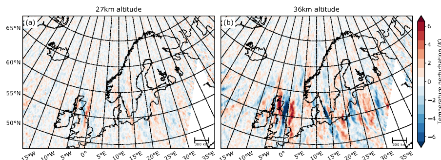
Figure 11. Temperature perturbations of the AIRS retrieval at 27 km (a) and 36 km (b) for the descending orbits with equator crossing time at 01:30 LT (between 01:00 UTC and 03:00 UTC above Scandinavia) on 29 January 2016.
