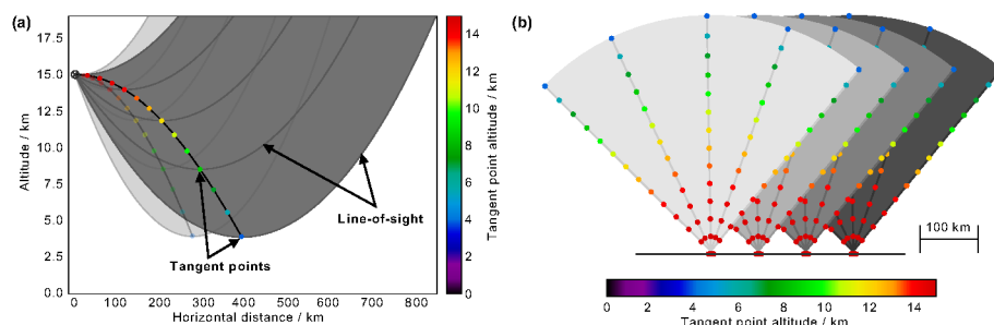
Figure 1. (a) Vertical cross-section of the limb-sounding geometry of GLORIA. The flight direction points into the paper plane. Images taken under 90^\circ azimuth cover the dark grey area with the LOS. The respective tangent points (bright coloured dots) increase in distance with decreasing altitude. The tangent points of forward- and rearward-looking images (light grey and pale coloured dots) are closer to the flightpath. The line-of-sight (LOS), which is a straight line in reality, has a parabolic shape in this plot due to the transformation into a Cartesian coordinate system with the x-axis following the Earth surface. (b) Top view in bird perspective of the flightpath of LAT. The dots again indicate the tangent points and are coloured according to their altitude. Each grey sector indicates one horizontal scan from 45 to 135^\circ . The lighter the grey, the later in time the measurements are taken. Figure taken from (Krisch et al., 2018).
