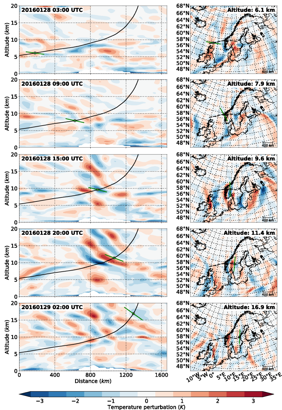
Figure 10. Cross sections through different ERA5 temperature perturbations along an exemplary GROGRAT ray trace originating from GLORIA measurements. The left column shows vertical cross sections along the ray trace (black line). The grey dot marks the location of the ray trace at the respective time step of the model. The green line shows the orientation of the phase lines as predicted by GROGRAT. The right column shows horizontal cross sections at the altitude of the ray path at the respective model time.
