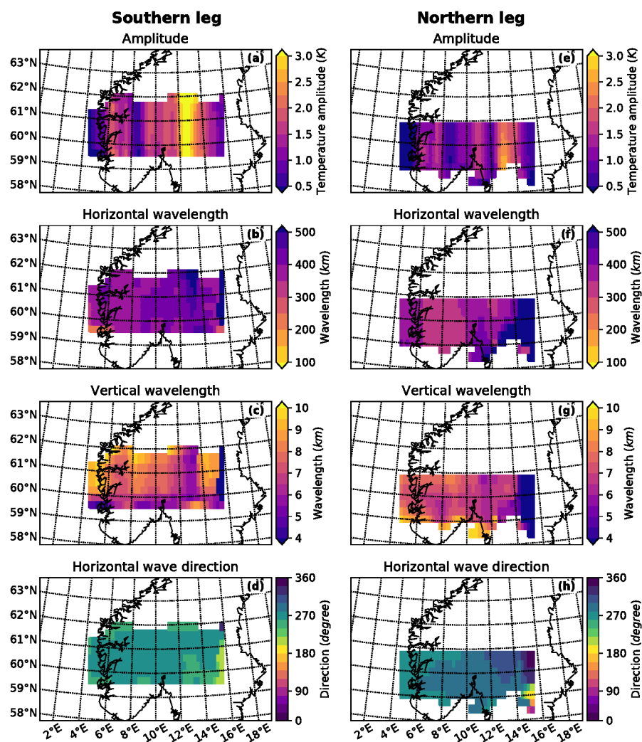
Figure 7. Three-dimensional sinusoidal wave fit of the GLORIA measurements at a centre height of 11.4 km in fitting cubes of 400 x 250 x 4 km with a tangent point weighting according to Sec. 2.5. In order to capture the spatial variation of the amplitudes, an amplitude and phase refit has been performed in fitting cubes of 100 x 250 x 1 km. Panels (d & h) show the direction of the horizontal wave vector. Eastward direction corresponds to 90° and southward direction to 180°
