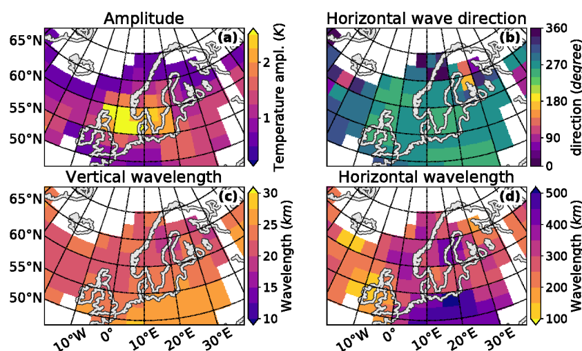
Figure 12. Three-dimensional sinusoidal wave fit of the AIRS measurements based on fitting cubes of 300 x 250 x 20 km at a centre height of 36 km.
