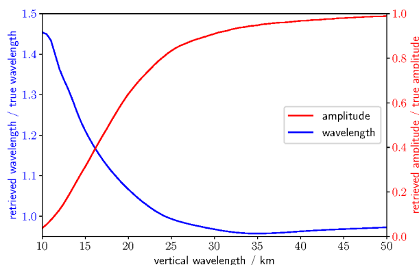
Figure 2. Sensitivity function of the AIRS temperature retrieval for GW amplitude (red) and vertical wavelength (blue) as estimated from a 1-D sinusoidal fitting routine at given real vertical wavelengths.
