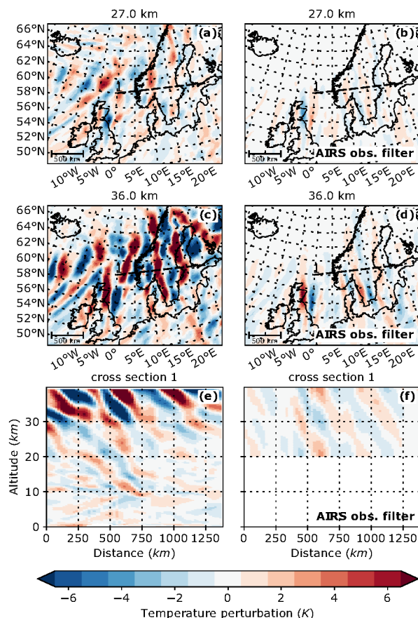
Figure 13. ECMWF forecast initialized on 29 January 2016 midnight for 03:00 UTC and the influence of the AIRS observational filter. The left column shows the original ECMWF forecast data, the right column shows what remains if the model data is multiplied with the averaging kernel matrix of the AIRS retrieval.
